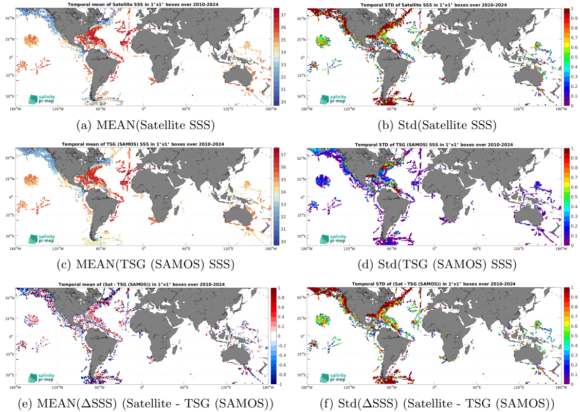
Figure 7: Temporal mean (left) and Std (right) of SSS from SMOS SSS L2Q v331 - With FLAG (CMEMS-CATDS-CPDC) (top), TSG (SAMOS) (middle), and of \Delta SSS (Satellite - TSG (SAMOS)). Only match-up pairs are used to generate these maps.
