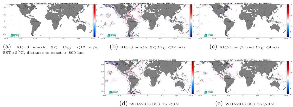
Figure 14: Temporal mean gridded over spatial boxes of size 1^\circ \times 1^\circ of \Delta\text{SSS} (SMOS SSS L2Q v331 - With FLAG (CMEMS-CATDS-CPDC) - TSG (SAMOS)) for 5 different subdatasets corresponding to: RR=0 mm/h, 3 < U_{10} < 12 m/s, SST > 5^\circ\text{C} , distance to coast > 800 km (a), RR=0 mm/h, 3 < U_{10} < 12 m/s (b), RR > 1 mm/h and U_{10} < 4 m/s (c), WOA2013 SSS Std < 0.2 (d), WOA2013 SSS Std > 0.2 (e).
