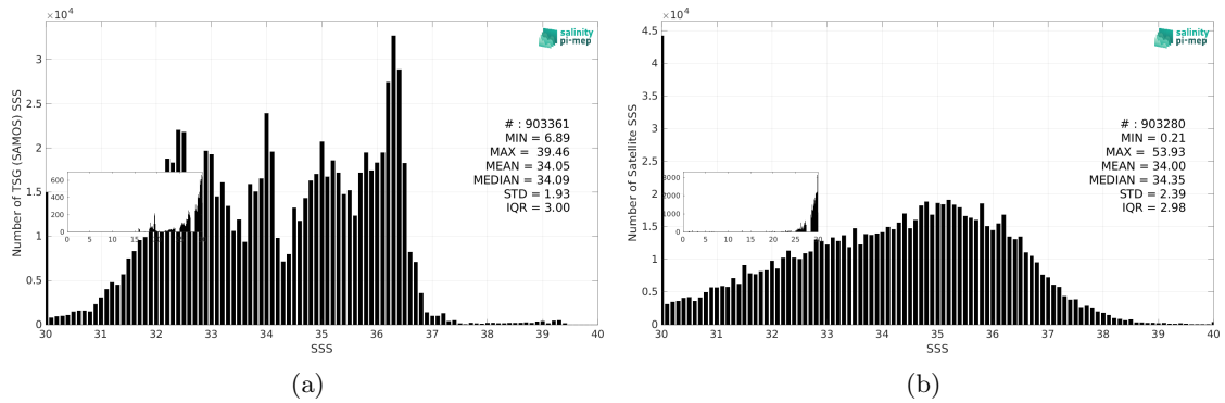
Figure 3: Histograms of SSS from TSG (SAMOS) (a) and SMOS SSS L2Q v331 - With FLAG (CMEMS-CATDS-CPDC) (b) considering all match-up pairs per bins of 0.1 over the SMOS coastal zone (<800km) 60N-60S Pi-MEP region and for the full satellite product period.
