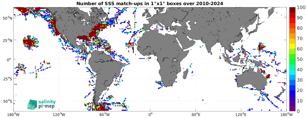
Figure 5: Number of SSS match-ups between TSG (SAMOS) SSS and the SMOS SSS L2Q v331 - With FLAG (CMEMS-CATDS-CPDC) SSS product for the SMOS coastal zone (<800km) 60N-60S Pi-MEP region over 1^{\circ} \times 1^{\circ} boxes and for the full satellite product period.
