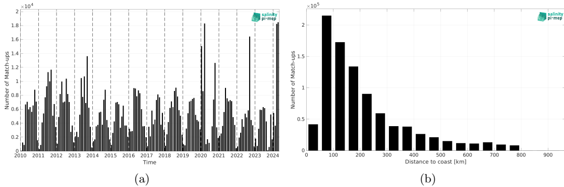
Figure 2: Number of match-ups between TSG (SAMOS) and SMOS SSS L2Q v331 - With FLAG (CMEMS-CATDS-CPDC) SSS as a function of time (a) and as function of the distance to coast (b) over the SMOS coastal zone (<800km) 60N-60S Pi-MEP region and for the full satellite product period.
