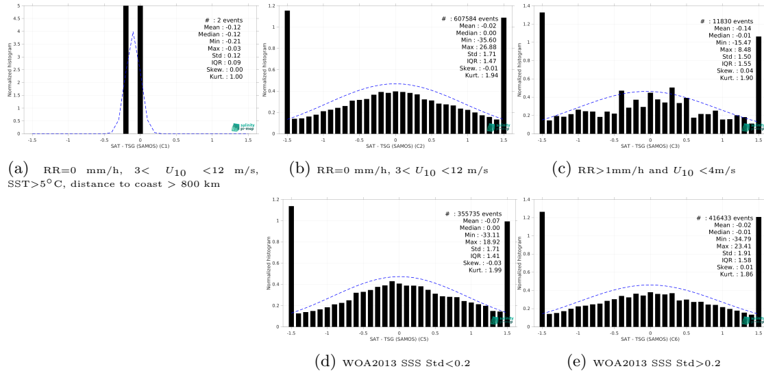
Figure 13: Normalized histogram of \Delta SSS (SMOS SSS L2Q v331 - With FLAG (CMEMS-CATDS-CPDC) - TSG (SAMOS)) for 5 different subdatasets corresponding to: RR=0 mm/h, 3 < U_{10} < 12 m/s, SST>5°C, distance to coast > 800 km (a), RR=0 mm/h, 3 < U_{10} < 12 m/s (b), RR>1mm/h and U_{10} < 4 m/s (c), WOA2013 SSS Std<0.2 (d), WOA2013 SSS Std>0.2 (e).
