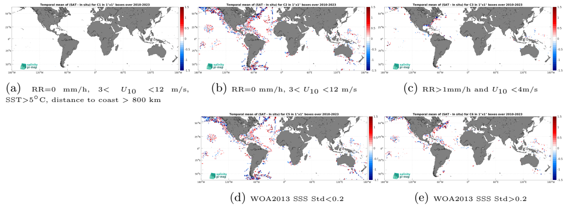
Figure 12: Temporal mean gridded over spatial boxes of size 1^\circ \times 1^\circ of \Delta\text{SSS} (SMOS SSS L2Q v331 - With FLAG (CMEMS-CATDS-CPDC) - TSG (SAMOS)) for 5 different subdatasets corresponding to:RR=0 mm/h, 3 < U_{10} < 12 m/s, SST >5^\circ\text{C} , distance to coast > 800 km (a), RR=0 mm/h, 3 < U_{10} < 12 m/s (b), RR >1 mm/h and U_{10} < 4 m/s (c), WOA2013 SSS Std <0.2 (d), WOA2013 SSS Std >0.2 (e).
