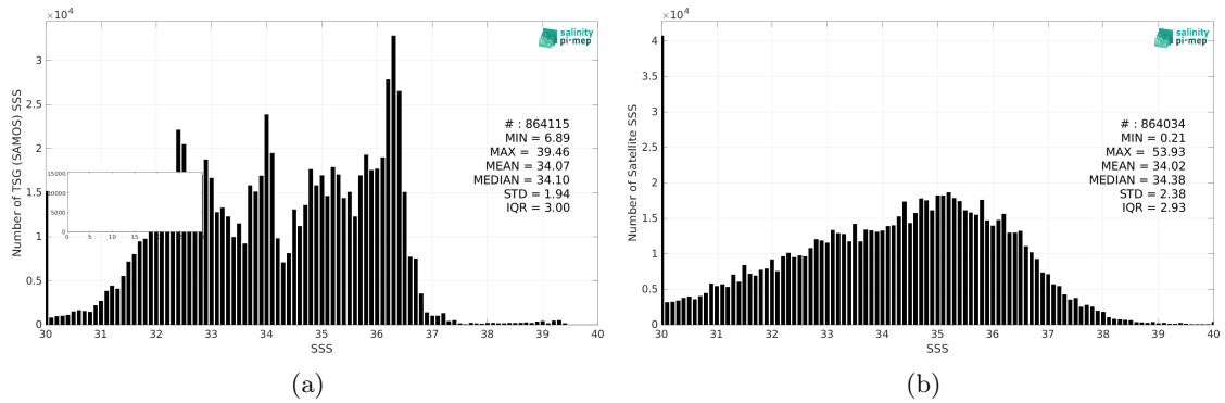
Figure 2: Histograms of SSS from TSG (SAMOS) (a) and SMOS SSS L2Q v331 - With FLAG (CMEMS-CATDS-CPDC) (b) considering all match-up pairs per bins of 0.1 over the SMOS coastal zone (<800km) 60N-60S Pi-MEP region and for the full satellite product period.
