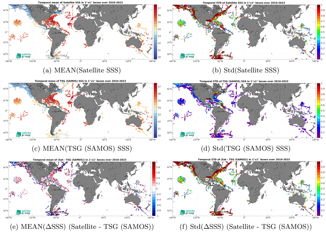
Figure 6: Temporal mean (left) and Std (right) of SSS from SMOS SSS L2Q v331 - With FLAG (CMEMS-CATDS-CPDC) (top), TSG (SAMOS) (middle), and of \Delta SSS (Satellite - TSG (SAMOS)). Only match-up pairs are used to generate these maps.
