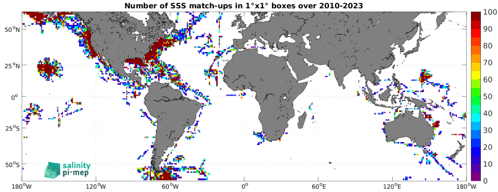
Figure 4: Number of SSS match-ups between TSG (SAMOS) SSS and the SMOS SSS L2Q v331 - With FLAG (CMEMS-CATDS-CPDC) SSS product for the SMOS coastal zone (<800km) 60N-60S Pi-MEP region over 1^\circ \times 1^\circ boxes and for the full satellite product period.
