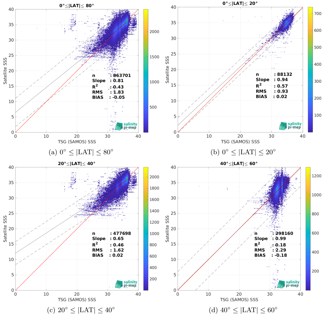
Figure 9: Contour maps of the concentration of SMOS SSS L2Q v331 - With FLAG (CMEMS-CATDS-CPDC) SSS (y-axis) versus TSG (SAMOS) SSS (x-axis) at match-up pairs for different latitude bands. For each plot, the red line shows x=y . The black thin and dashed lines indicate a linear fit through the data cloud and the \pm 95\% confidence levels, respectively. The number match-up pairs n , the slope and R^2 coefficient of the linear fit, the root mean square (RMS) and the mean bias between satellite and in situ data are indicated for each latitude band in each plots.
