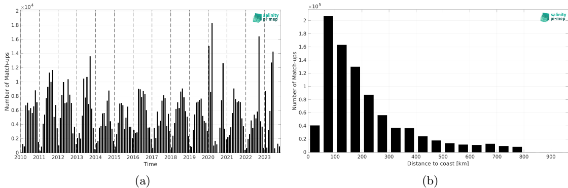
Figure 1: Number of match-ups between TSG (SAMOS) and SMOS SSS L2Q v331 - With FLAG (CMEMS-CATDS-CPDC) SSS as a function of time (a) and as function of the distance to coast (b) over the SMOS coastal zone (<800km) 60N-60S Pi-MEP region and for the full satellite product period.
