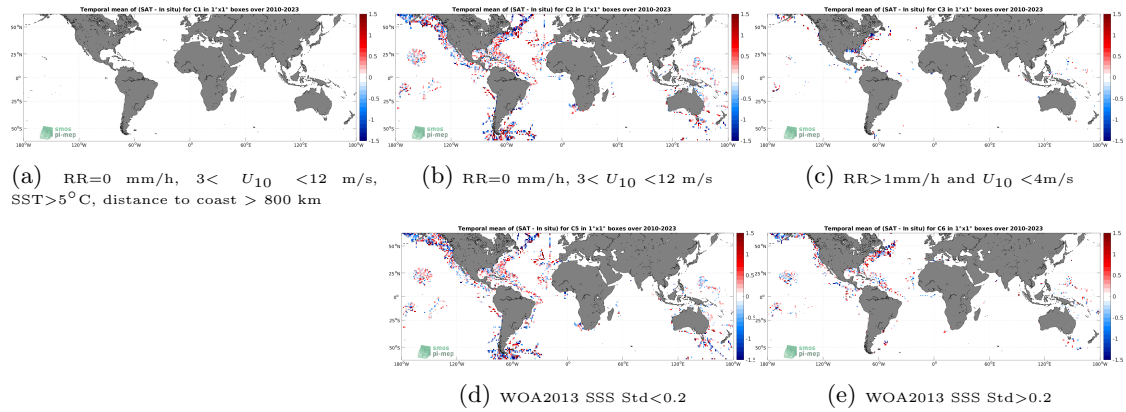
Figure 12: Temporal mean gridded over spatial boxes of size 1^\circ \times 1^\circ of \Delta SSS (SMOS SSS L2Q v331 - With FLAG (CMEMS-CATDS-CPDC) - TSG (SAMOS)) for 5 different subdatasets corresponding to:RR=0 mm/h, 3 < U_{10} < 12 m/s, SST >5^\circ\text{C} , distance to coast > 800 km (a), RR=0 mm/h, 3 < U_{10} < 12 m/s (b), RR >1 mm/h and U_{10} < 4 m/s (c), WOA2013 SSS Std <0.2 (d), WOA2013 SSS Std >0.2 (e).
