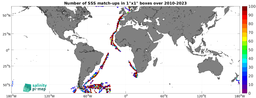
Figure 5: Number of SSS match-ups between TSG (Polarstern) SSS and the SMOS SSS L2Q v331 - With FLAG (CMEMS-CATDS-CPDC) SSS product for the SMOS coastal zone ( <800\text{km} ) 60N-60S Pi-MEP region over 1^\circ \times 1^\circ boxes and for the full satellite product period.
