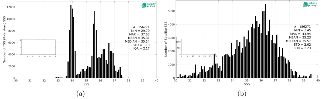
Figure 3: Histograms of SSS from TSG (Polarstern) (a) and SMOS SSS L2Q v331 - With FLAG (CMEMS-CATDS-CPDC) (b) considering all match-up pairs per bins of 0.1 over the SMOS coastal zone (<800km) 60N-60S Pi-MEP region and for the full satellite product period.
