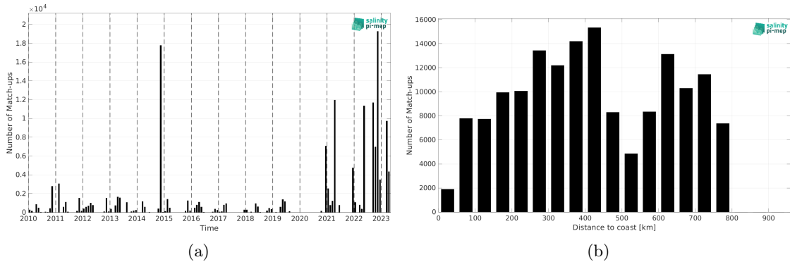
Figure 2: Number of match-ups between TSG (Polarstern) and SMOS SSS L2Q v331 - With FLAG (CMEMS-CATDS-CPDC) SSS as a function of time (a) and as function of the distance to coast (b) over the SMOS coastal zone (<800km) 60N-60S Pi-MEP region and for the full satellite product period.
