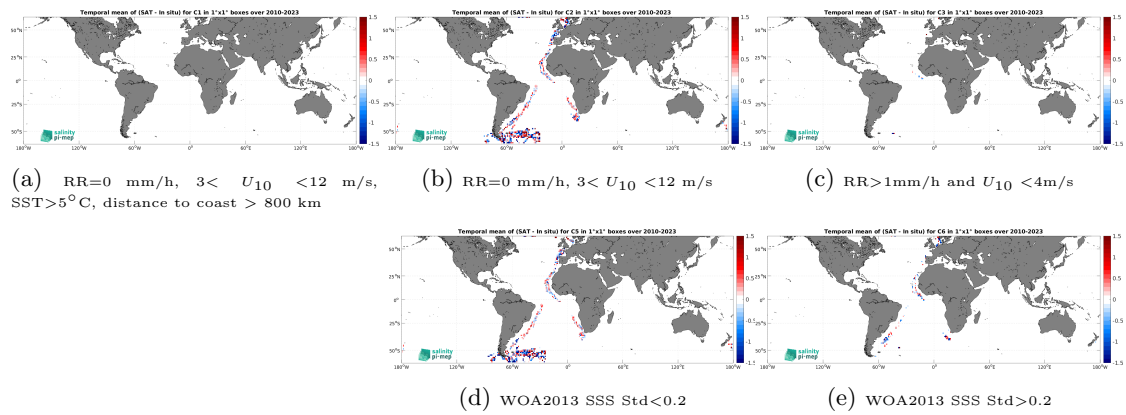
Figure 14: Temporal mean gridded over spatial boxes of size 1^\circ \times 1^\circ of \Delta\text{SSS} (SMOS SSS L2Q v331 - With FLAG (CMEMS-CATDS-CPDC) - TSG (Polarstern)) for 5 different subdatasets corresponding to: RR=0 mm/h, 3 < U_{10} < 12 m/s, SST > 5°C, distance to coast > 800 km (a), RR=0 mm/h, 3 < U_{10} < 12 m/s (b), RR > 1mm/h and U_{10} < 4 m/s (c), WOA2013 SSS Std < 0.2 (d), WOA2013 SSS Std > 0.2 (e).
