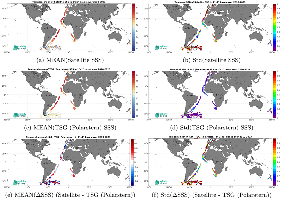
Figure 7: Temporal mean (left) and Std (right) of SSS from SMOS SSS L2Q v331 - With FLAG (CMEMS-CATDS-CPDC) (top), TSG (Polarstern) (middle), and of \Delta\text{SSS} (Satellite - TSG (Polarstern)). Only match-up pairs are used to generate these maps.
