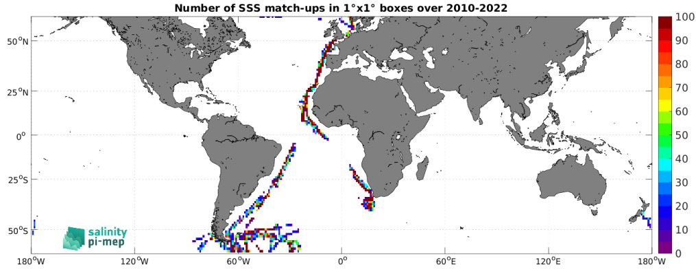
Figure 4: Number of SSS match-ups between TSG (Polarstern) SSS and the SMOS SSS L2Q v331 - With FLAG (CMEMS-CATDS-CPDC) SSS product for the SMOS coastal zone ( <800\text{km} ) 60N-60S Pi-MEP region over 1^\circ \times 1^\circ boxes and for the full satellite product period.
