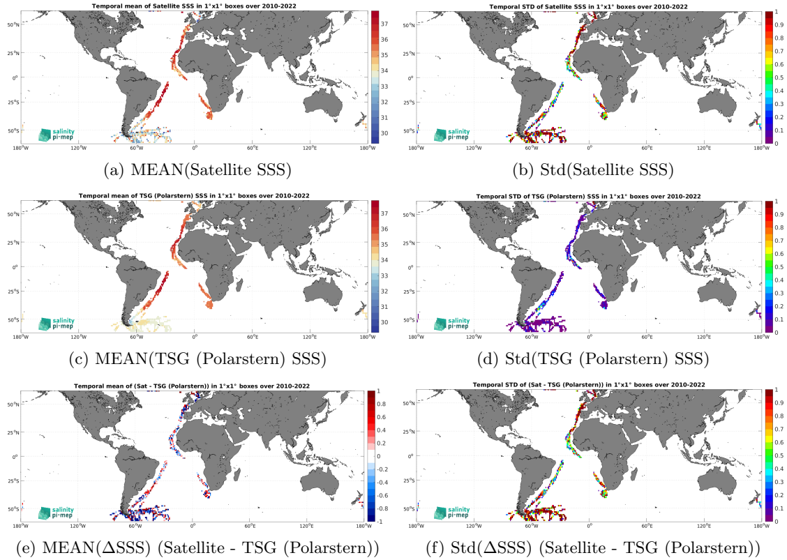
Figure 6: Temporal mean (left) and Std (right) of SSS from SMOS SSS L2Q v331 - With FLAG (CMEMS-CATDS-CPDC) (top), TSG (Polarstern) (middle), and of \Delta SSS (Satellite - TSG (Polarstern)). Only match-up pairs are used to generate these maps.
