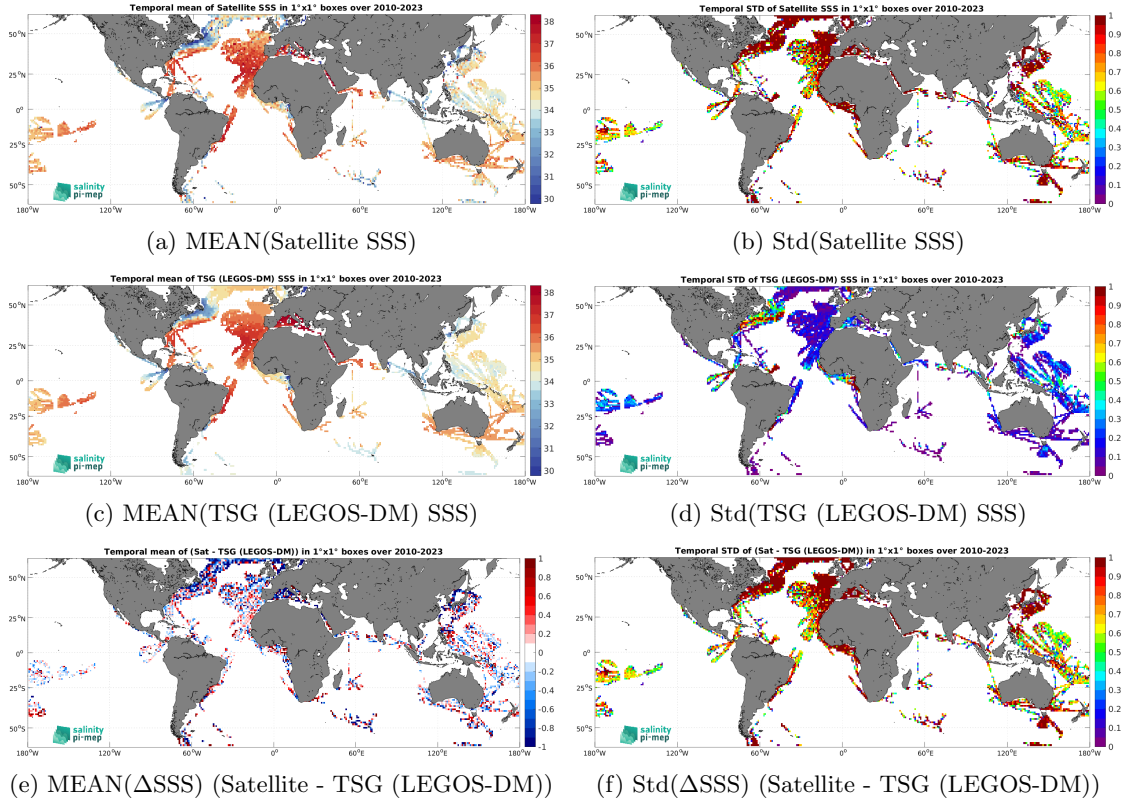
Figure 6: Temporal mean (left) and Std (right) of SSS from SMOS SSS L2Q v331 - With FLAG (CMEMS-CATDS-CPDC) (top), TSG (LEGOS-DM) (middle), and of \Delta\text{SSS} (Satellite - TSG (LEGOS-DM)). Only match-up pairs are used to generate these maps.
