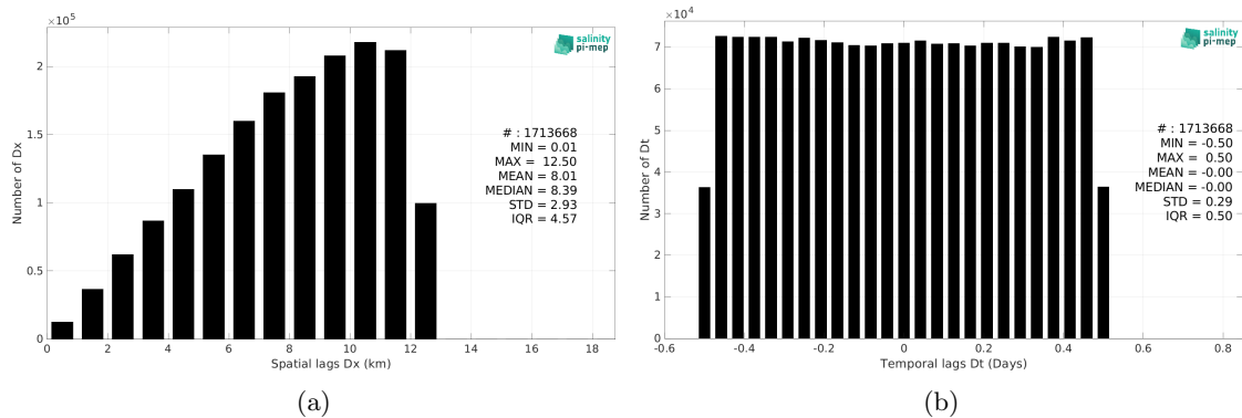
Figure 5: Histograms of the spatial (a) and temporal (b) lags between the location/time of the TSG (LEGOS-DM) measurement and the date of the corresponding SMOS SSS L2Q v331 - With FLAG (CMEMS-CATDS-CPDC) SSS pixel.
