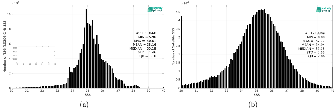
Figure 2: Histograms of SSS from TSG (LEGOS-DM) (a) and SMOS SSS L2Q v331 - With FLAG (CMEMS-CATDS-CPDC) (b) considering all match-up pairs per bins of 0.1 over the SMOS coastal zone (<800km) 60N-60S Pi-MEP region and for the full satellite product period.
