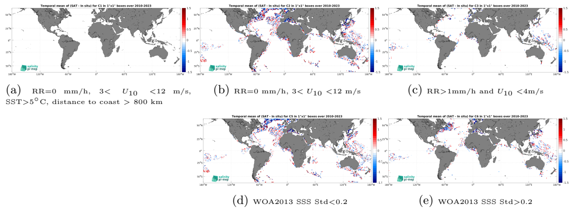
Figure 12: Temporal mean gridded over spatial boxes of size 1^\circ \times 1^\circ of \Delta SSS (SMOS SSS L2Q v331 - With FLAG (CMEMS-CATDS-CPDC) - TSG (LEGOS-DM)) for 5 different subdatasets corresponding to:RR=0 mm/h, 3 < U_{10} < 12 m/s, SST >5^\circ C, distance to coast > 800 km (a), RR=0 mm/h, 3 < U_{10} < 12 m/s (b), RR >1 mm/h and U_{10} < 4 m/s (c), WOA2013 SSS Std <0.2 (d), WOA2013 SSS Std >0.2 (e).
