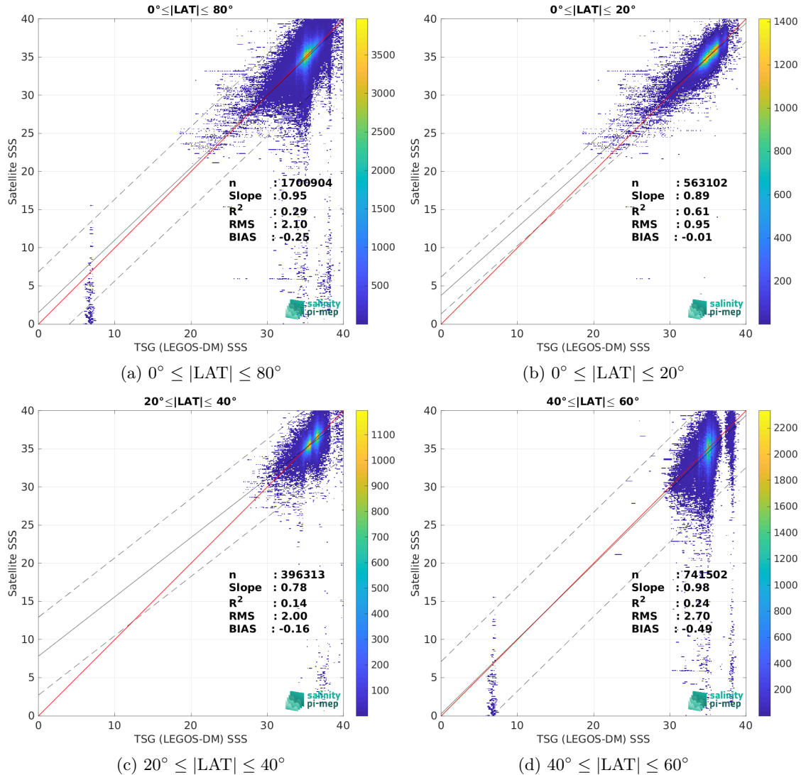
Figure 9: Contour maps of the concentration of SMOS SSS L2Q v331 - With FLAG (CMEMS-CATDS-CPDC) SSS (y-axis) versus TSG (LEGOS-DM) SSS (x-axis) at match-up pairs for different latitude bands. For each plot, the red line shows x=y . The black thin and dashed lines indicate a linear fit through the data cloud and the \pm 95\% confidence levels, respectively. The number match-up pairs n , the slope and R^2 coefficient of the linear fit, the root mean square (RMS) and the mean bias between satellite and in situ data are indicated for each latitude band in each plots.
