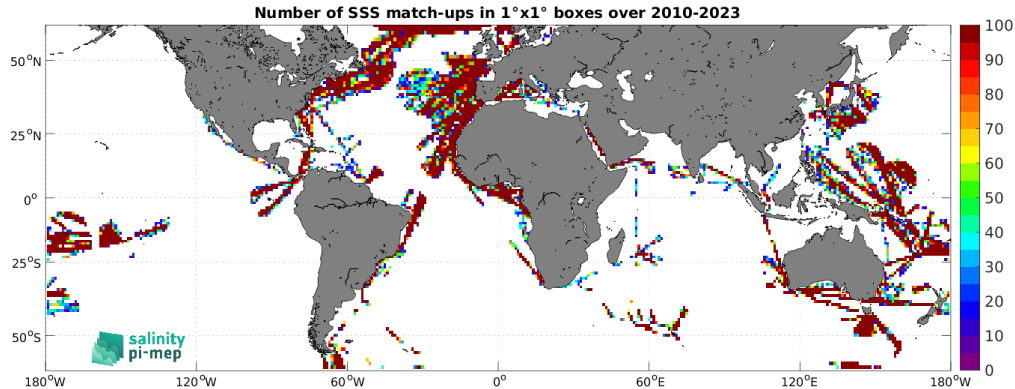
Figure 4: Number of SSS match-ups between TSG (LEGOS-DM) SSS and the SMOS SSS L2Q v331 - With FLAG (CMEMS-CATDS-CPDC) SSS product for the SMOS coastal zone ( <800\text{km} ) 60N-60S Pi-MEP region over 1^\circ \times 1^\circ boxes and for the full satellite product period.
