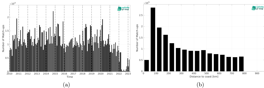
Figure 1: Number of match-ups between TSG (LEGOS-DM) and SMOS SSS L2Q v331 - With FLAG (CMEMS-CATDS-CPDC) SSS as a function of time (a) and as function of the distance to coast (b) over the SMOS coastal zone (<800km) 60N-60S Pi-MEP region and for the full satellite product period.
