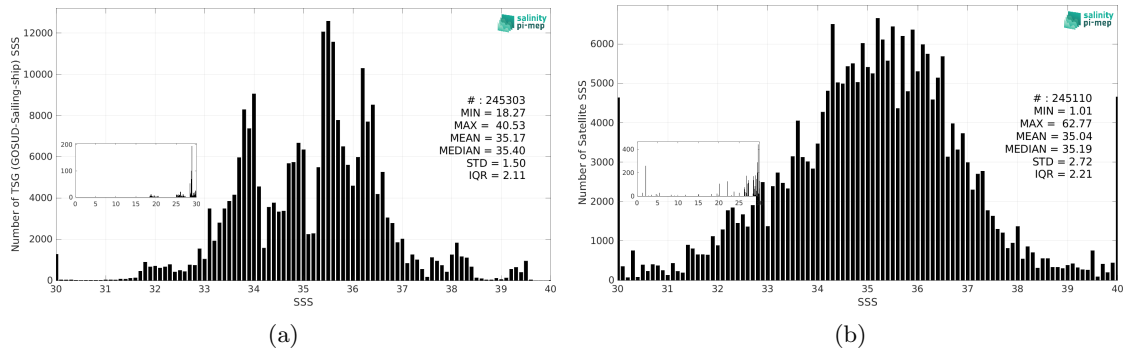
Figure 3: Histograms of SSS from TSG (GOSUD-Sailing-ship) (a) and SMOS SSS L2Q v331 - With FLAG (CMEMS-CATDS-CPDC) (b) considering all match-up pairs per bins of 0.1 over the SMOS coastal zone (<800km) 60N-60S Pi-MEP region and for the full satellite product period.
