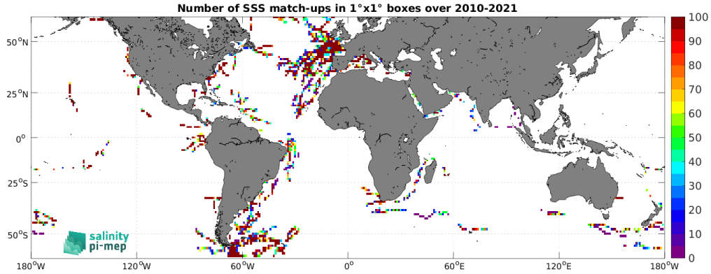
Figure 5: Number of SSS match-ups between TSG (GOSUD-Sailing-ship) SSS and the SMOS SSS L2Q v331 - With FLAG (CMEMS-CATDS-CPDC) SSS product for the SMOS coastal zone (<800km) 60N-60S Pi-MEP region over 1^{\circ} \times 1^{\circ} boxes and for the full satellite product period.
