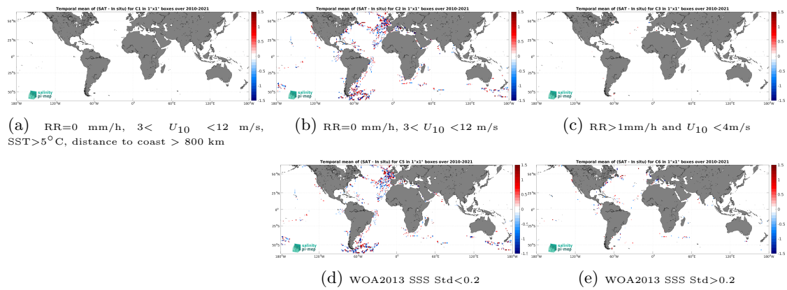
Figure 14: Temporal mean gridded over spatial boxes of size 1^\circ \times 1^\circ of \Delta\text{SSS} (SMOS SSS L2Q v331 - With FLAG (CMEMS-CATDS-CPDC) - TSG (GOSUD-Sailing-ship)) for 5 different subdatasets corresponding to: RR=0 mm/h, 3 < U_{10} < 12 m/s, SST > 5°C, distance to coast > 800 km (a), RR=0 mm/h, 3 < U_{10} < 12 m/s (b), RR > 1mm/h and U_{10} < 4 m/s (c), WOA2013 SSS Std < 0.2 (d), WOA2013 SSS Std > 0.2 (e).
