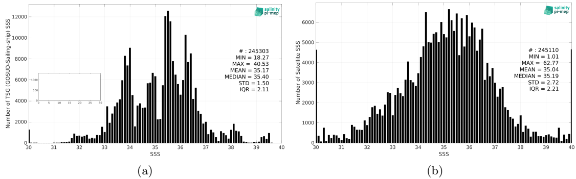
Figure 2: Histograms of SSS from TSG (GOSUD-Sailing-ship) (a) and SMOS SSS L2Q v331 - With FLAG (CMEMS-CATDS-CPDC) (b) considering all match-up pairs per bins of 0.1 over the SMOS coastal zone (<800km) 60N-60S Pi-MEP region and for the full satellite product period.
