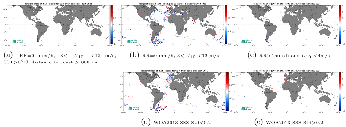
Figure 12: Temporal mean gridded over spatial boxes of size 1^\circ \times 1^\circ of \Delta SSS (SMOS SSS L2Q v331 - With FLAG (CMEMS-CATDS-CPDC) - TSG (GOSUD-Sailing-ship)) for 5 different subdatasets corresponding to:RR=0 mm/h, 3 < U_{10} < 12 m/s, SST >5^\circ C, distance to coast > 800 km (a), RR=0 mm/h, 3 < U_{10} < 12 m/s (b), RR >1 mm/h and U_{10} < 4 m/s (c), WOA2013 SSS Std <0.2 (d), WOA2013 SSS Std >0.2 (e).
