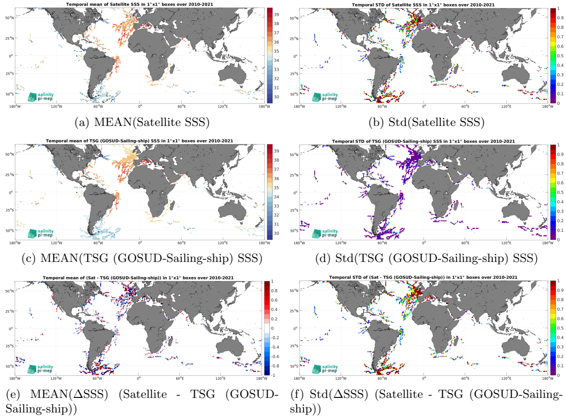
Figure 6: Temporal mean (left) and Std (right) of SSS from SMOS SSS L2Q v331 - With FLAG (CMEMS-CATDS-CPDC) (top), TSG (GOSUD-Sailing-ship) (middle), and of \Delta SSS (Satellite - TSG (GOSUD-Sailing-ship)). Only match-up pairs are used to generate these maps.
