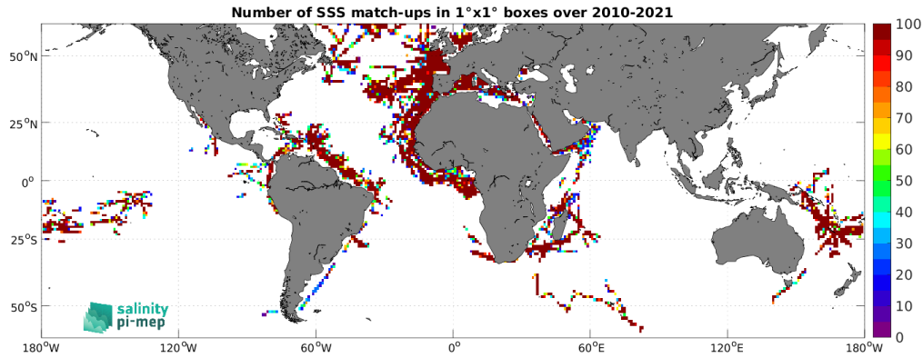
Figure 5: Number of SSS match-ups between TSG (GOSUD-Research-vessel) SSS and the SMOS SSS L2Q v331 - With FLAG (CMEMS-CATDS-CPDC) SSS product for the SMOS coastal zone (<800km) 60N-60S Pi-MEP region over 1^\circ \times 1^\circ boxes and for the full satellite product period.
