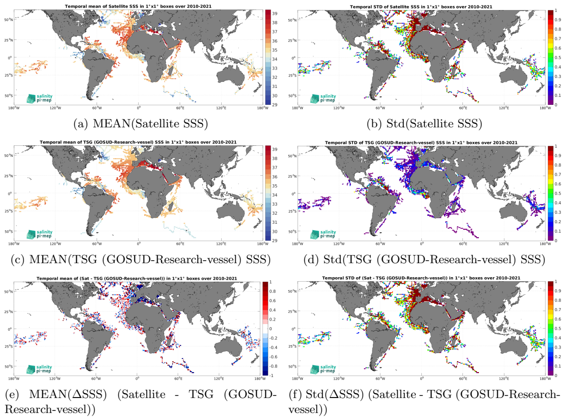
Figure 7: Temporal mean (left) and Std (right) of SSS from SMOS SSS L2Q v331 - With FLAG (CMEMS-CATDS-CPDC) (top), TSG (GOSUD-Research-vessel) (middle), and of \Delta SSS (Satellite - TSG (GOSUD-Research-vessel)). Only match-up pairs are used to generate these maps.
