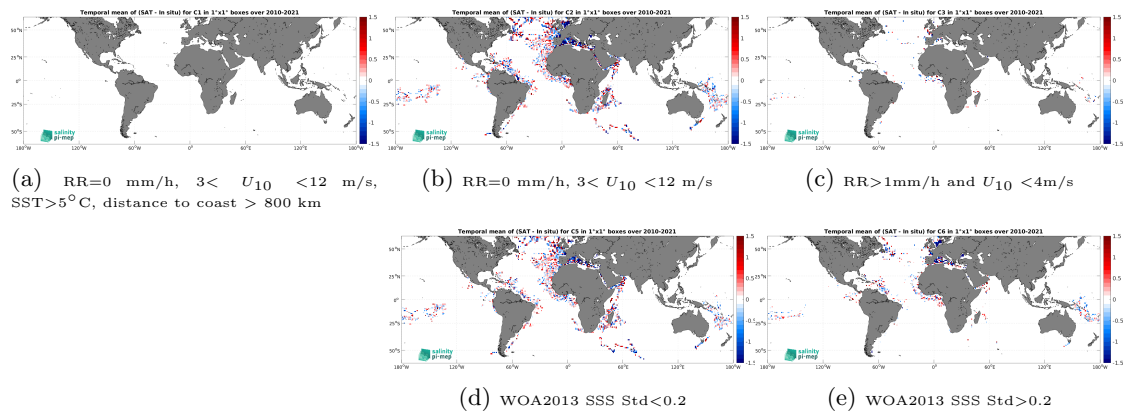
Figure 14: Temporal mean gridded over spatial boxes of size 1^\circ \times 1^\circ of \Delta SSS (SMOS SSS L2Q v331 - With FLAG (CMEMS-CATDS-CPDC) - TSG (GOSUD-Research-vessel)) for 5 different subdatasets corresponding to:RR=0 mm/h, 3 < U_{10} < 12 m/s, SST > 5^\circ\text{C} , distance to coast > 800 km (a), RR=0 mm/h, 3 < U_{10} < 12 m/s (b), RR > 1 mm/h and U_{10} < 4 m/s (c), WOA2013 SSS Std < 0.2 (d), WOA2013 SSS Std > 0.2 (e).
