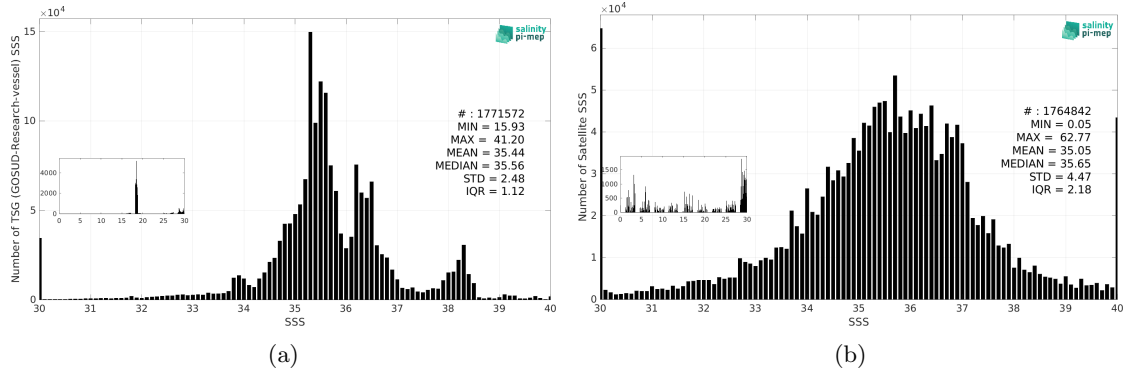
Figure 3: Histograms of SSS from TSG (GOSUD-Research-vessel) (a) and SMOS SSS L2Q v331 - With FLAG (CMEMS-CATDS-CPDC) (b) considering all match-up pairs per bins of 0.1 over the SMOS coastal zone (<800km) 60N-60S Pi-MEP region and for the full satellite product period.
