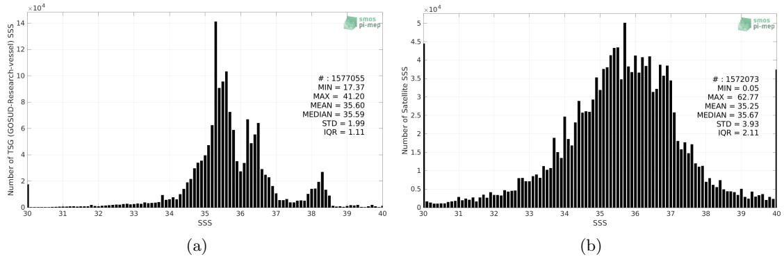
Figure 2: Histograms of SSS from TSG (GOSUD-Research-vessel) (a) and SMOS SSS L2Q v331 - With FLAG (CMEMS-CATDS-CPDC) (b) considering all match-up pairs per bins of 0.1 over the SMOS coastal zone (<800km) 60N-60S Pi-MEP region and for the full satellite product period.
