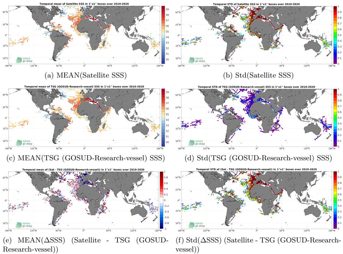
Figure 6: Temporal mean (left) and Std (right) of SSS from SMOS SSS L2Q v331 - With FLAG (CMEMS-CATDS-CPDC) (top), TSG (GOSUD-Research-vessel) (middle), and of \Delta SSS (Satellite - TSG (GOSUD-Research-vessel)). Only match-up pairs are used to generate these maps.
