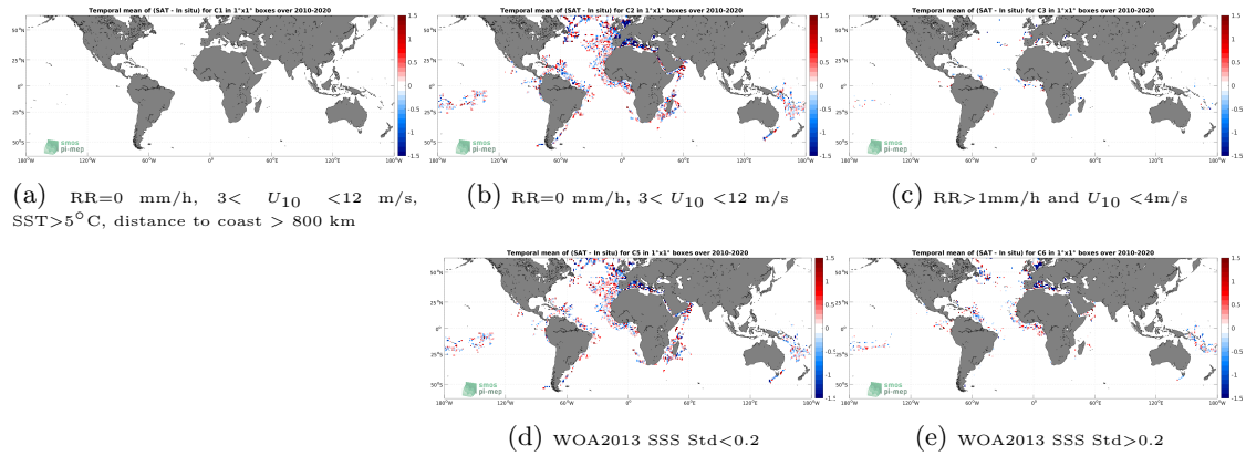
Figure 12: Temporal mean gridded over spatial boxes of size 1^\circ \times 1^\circ of \Delta SSS (SMOS SSS L2Q v331 - With FLAG (CMEMS-CATDS-CPDC) - TSG (GOSUD-Research-vessel)) for 5 different subdatasets corresponding to:RR=0 mm/h, 3 < U_{10} < 12 m/s, SST >5^\circ\text{C} , distance to coast > 800 km (a), RR=0 mm/h, 3 < U_{10} < 12 m/s (b), RR >1 mm/h and U_{10} < 4 m/s (c), WOA2013 SSS Std <0.2 (d), WOA2013 SSS Std >0.2 (e).
