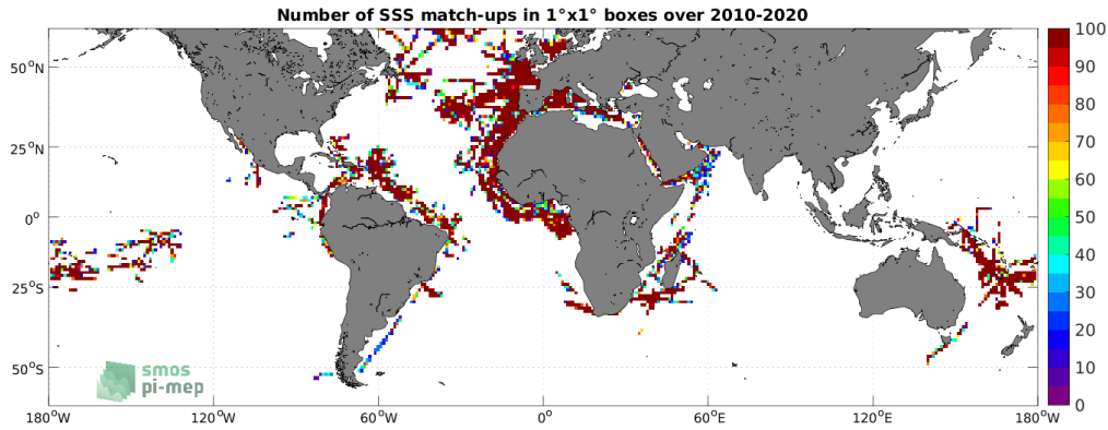
Figure 4: Number of SSS match-ups between TSG (GOSUD-Research-vessel) SSS and the SMOS SSS L2Q v331 - With FLAG (CMEMS-CATDS-CPDC) SSS product for the SMOS coastal zone (<800km) 60N-60S Pi-MEP region over 1^\circ \times 1^\circ boxes and for the full satellite product period.
