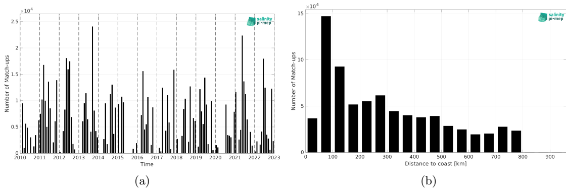
Figure 2: Number of match-ups between TSG (CSIC-UTM) and SMOS SSS L2Q v331 - With FLAG (CMEMS-CATDS-CPDC) SSS as a function of time (a) and as function of the distance to coast (b) over the SMOS coastal zone (<800km) 60N-60S Pi-MEP region and for the full satellite product period.
