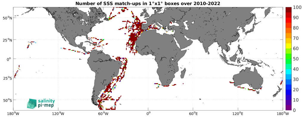
Figure 5: Number of SSS match-ups between TSG (CSIC-UTM) SSS and the SMOS SSS L2Q v331 - With FLAG (CMEMS-CATDS-CPDC) SSS product for the SMOS coastal zone (<800km) 60N-60S Pi-MEP region over 1^\circ \times 1^\circ boxes and for the full satellite product period.
