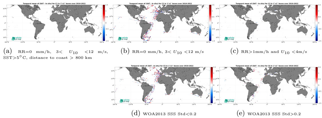
Figure 14: Temporal mean gridded over spatial boxes of size 1^\circ \times 1^\circ of \Delta\text{SSS} (SMOS SSS L2Q v331 - With FLAG (CMEMS-CATDS-CPDC) - TSG (CSIC-UTM)) for 5 different subdatasets corresponding to: RR=0 mm/h, 3 < U_{10} < 12 m/s, SST > 5°C, distance to coast > 800 km (a), RR=0 mm/h, 3 < U_{10} < 12 m/s (b), RR > 1mm/h and U_{10} < 4 m/s (c), WOA2013 SSS Std < 0.2 (d), WOA2013 SSS Std > 0.2 (e).
