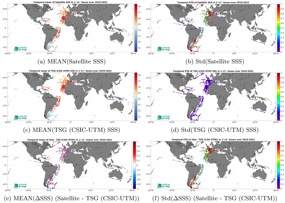
Figure 7: Temporal mean (left) and Std (right) of SSS from SMOS SSS L2Q v331 - With FLAG (CMEMS-CATDS-CPDC) (top), TSG (CSIC-UTM) (middle), and of \Delta SSS (Satellite - TSG (CSIC-UTM)). Only match-up pairs are used to generate these maps.
