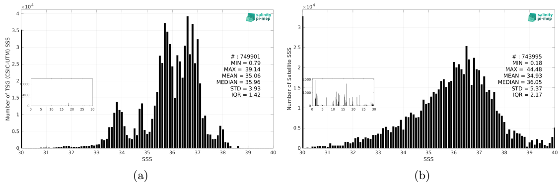
Figure 3: Histograms of SSS from TSG (CSIC-UTM) (a) and SMOS SSS L2Q v331 - With FLAG (CMEMS-CATDS-CPDC) (b) considering all match-up pairs per bins of 0.1 over the SMOS coastal zone (<800km) 60N-60S Pi-MEP region and for the full satellite product period.
