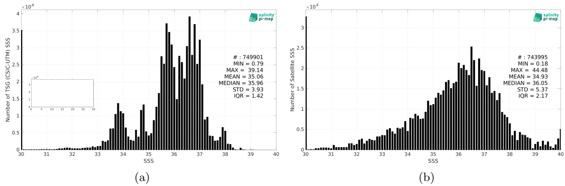
Figure 2: Histograms of SSS from TSG (CSIC-UTM) (a) and SMOS SSS L2Q v331 - With FLAG (CMEMS-CATDS-CPDC) (b) considering all match-up pairs per bins of 0.1 over the SMOS coastal zone (<800km) 60N-60S Pi-MEP region and for the full satellite product period.
