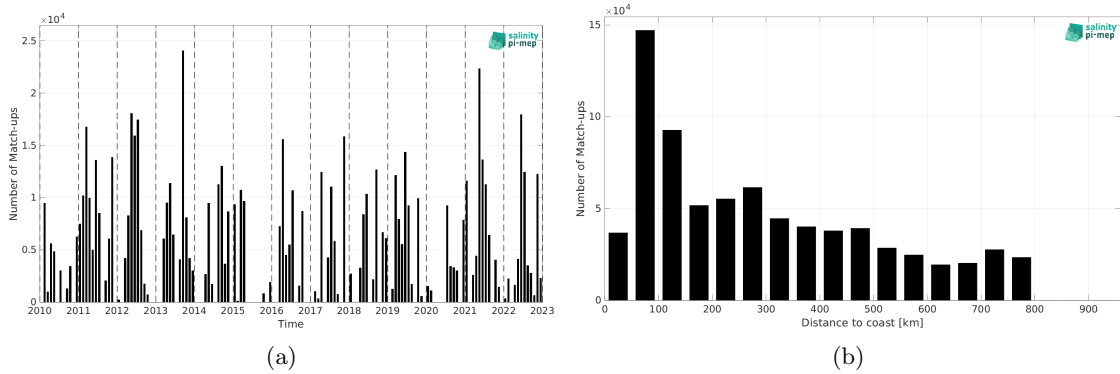
Figure 1: Number of match-ups between TSG (CSIC-UTM) and SMOS SSS L2Q v331 - With FLAG (CMEMS-CATDS-CPDC) SSS as a function of time (a) and as function of the distance to coast (b) over the SMOS coastal zone (<800km) 60N-60S Pi-MEP region and for the full satellite product period.
