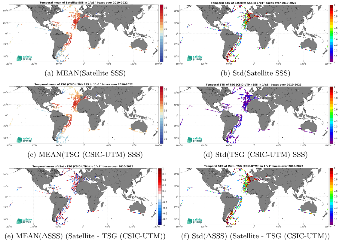
Figure 6: Temporal mean (left) and Std (right) of SSS from SMOS SSS L2Q v331 - With FLAG (CMEMS-CATDS-CPDC) (top), TSG (CSIC-UTM) (middle), and of \Delta SSS (Satellite - TSG (CSIC-UTM)). Only match-up pairs are used to generate these maps.
