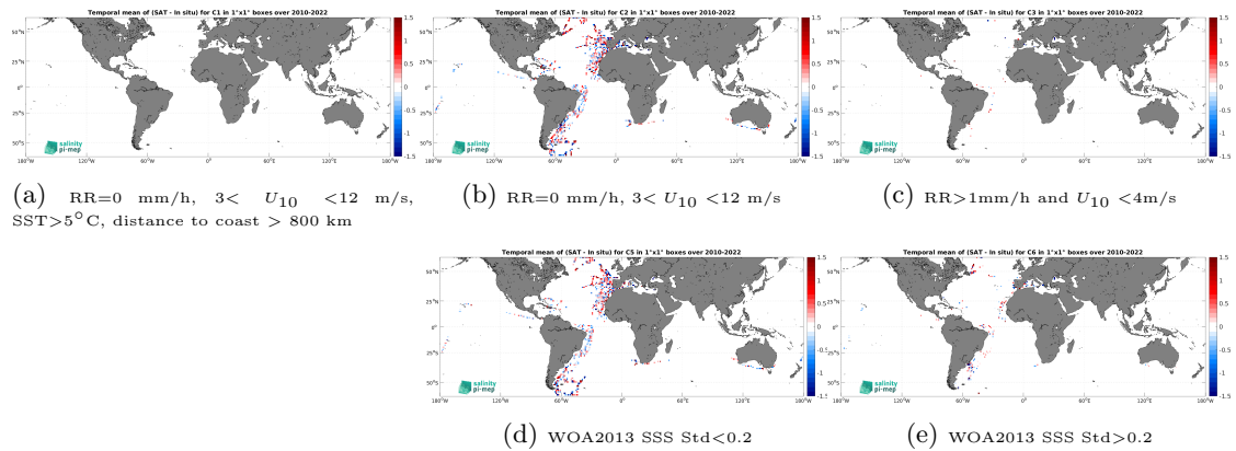
Figure 12: Temporal mean gridded over spatial boxes of size 1^\circ \times 1^\circ of \Delta SSS (SMOS SSS L2Q v331 - With FLAG (CMEMS-CATDS-CPDC) - TSG (CSIC-UTM)) for 5 different subdatasets corresponding to:RR=0 mm/h, 3 < U_{10} < 12 m/s, SST >5^\circ C, distance to coast > 800 km (a), RR=0 mm/h, 3 < U_{10} < 12 m/s (b), RR >1 mm/h and U_{10} < 4 m/s (c), WOA2013 SSS Std <0.2 (d), WOA2013 SSS Std >0.2 (e).
