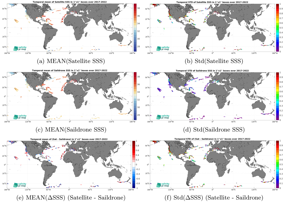
Figure 7: Temporal mean (left) and Std (right) of SSS from SMOS SSS L2Q v331 - With FLAG (CMEMS-CATDS-CPDC) (top), Saildrone (middle), and of \Delta SSS (Satellite - Saildrone). Only match-up pairs are used to generate these maps.
