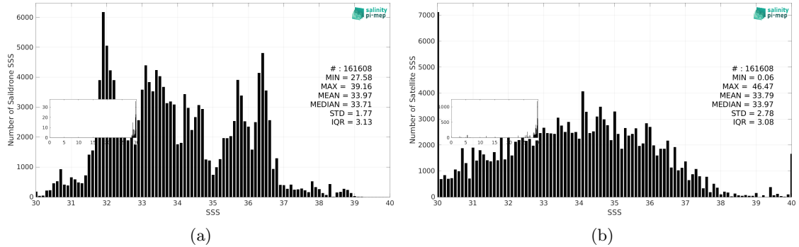
Figure 3: Histograms of SSS from Sairdrone (a) and SMOS SSS L2Q v331 - With FLAG (CMEMS-CATDS-CPDC) (b) considering all match-up pairs per bins of 0.1 over the SMOS coastal zone (<800km) 60N-60S Pi-MEP region and for the full satellite product period.
