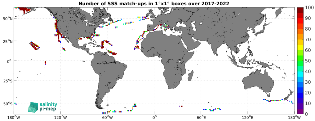
Figure 5: Number of SSS match-ups between Saildrone SSS and the SMOS SSS L2Q v331 - With FLAG (CMEMS-CATDS-CPDC) SSS product for the SMOS coastal zone (<800km) 60N-60S Pi-MEP region over 1^\circ \times 1^\circ boxes and for the full satellite product period.
