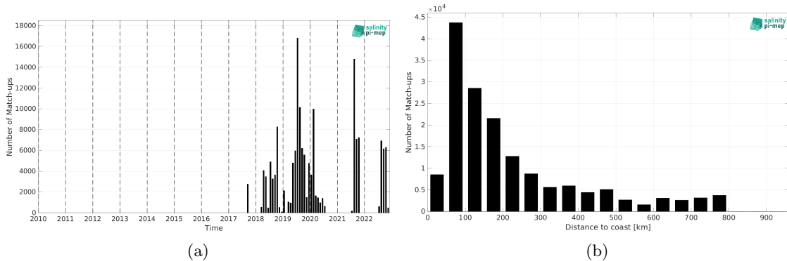
Figure 2: Number of match-ups between Saildrone and SMOS SSS L2Q v331 - With FLAG (CMEMS-CATDS-CPDC) SSS as a function of time (a) and as function of the distance to coast (b) over the SMOS coastal zone (<800km) 60N-60S Pi-MEP region and for the full satellite product period.
