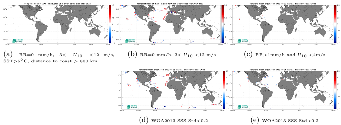
Figure 14: Temporal mean gridded over spatial boxes of size 1^\circ \times 1^\circ of \Delta SSS (SMOS SSS L2Q v331 - With FLAG (CMEMS-CATDS-CPDC) - Saildrone) for 5 different subdatasets corresponding to:RR=0 mm/h, 3 < U_{10} < 12 m/s, SST >5^\circ C, distance to coast > 800 km (a), RR=0 mm/h, 3 < U_{10} < 12 m/s (b), RR >1 mm/h and U_{10} < 4 m/s (c), WOA2013 SSS Std <0.2 (d), WOA2013 SSS Std >0.2 (e).
