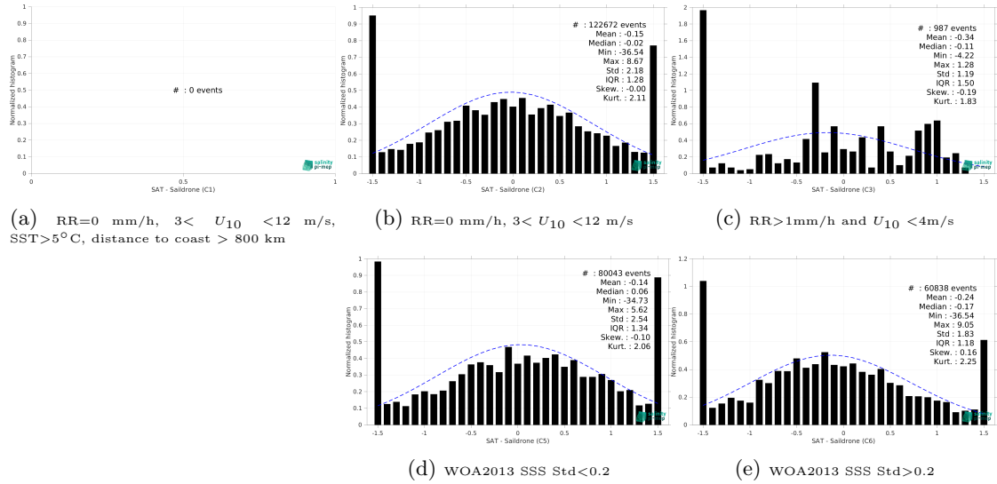
Figure 13: Normalized histogram of \Delta SSS (SMOS SSS L2Q v331 - With FLAG (CMEMS-CATDS-CPDC) - Sairdrone) for 5 different subdatasets corresponding to: RR=0 mm/h, 3 < U_{10} < 12 m/s, SST > 5°C, distance to coast > 800 km (a), RR=0 mm/h, 3 < U_{10} < 12 m/s (b), RR > 1mm/h and U_{10} < 4 m/s (c), WOA2013 SSS Std < 0.2 (d), WOA2013 SSS Std > 0.2 (e).
