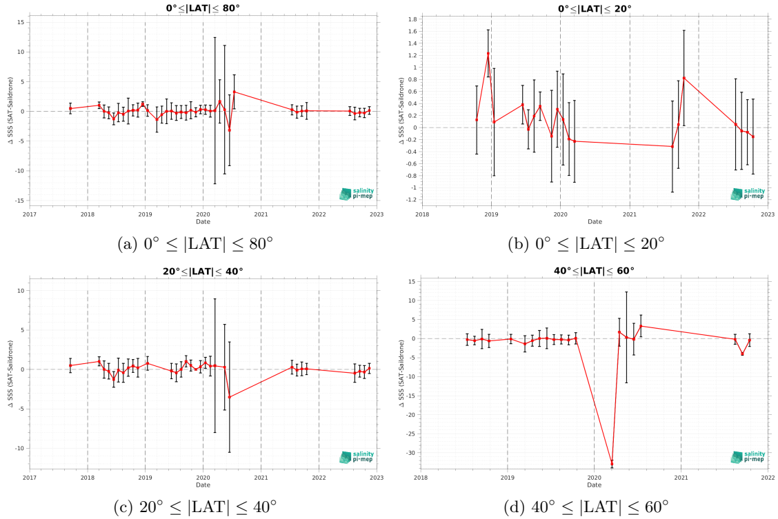
Figure 10: Monthly median (red curves) of \Delta\text{SSS} (Satellite - Sairdronne) and \pm 1 Std (black vertical thick bars) as function of time for all the collected Pi-MEP match-up pairs estimated over the SMOS coastal zone ( < 800\text{km} ) 60N-60S Pi-MEP region and for the full satellite product period are shown for different latitude bands: (a) 80°S-80°N, (b) 20°S-20°N, (c) 40°S-20°S and 20°N-40°N and (d) 60°S-40°S and 40°N-60°N.
