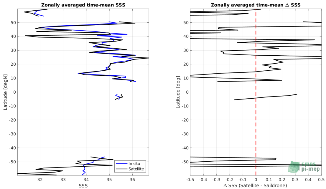
Figure 8: Left panel: Zonal mean SSS from SMOS SSS L2Q v331 - With FLAG (CMEMS-CATDS-CPDC) satellite product (black) and from Sairdrone (blue). Right panel: Zonal mean of \Delta SSS (Satellite - Sairdrone) for all the collected Pi-MEP match-up pairs estimated over the full satellite product period.
