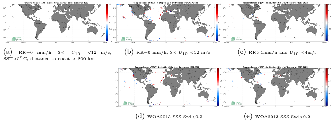
Figure 12: Temporal mean gridded over spatial boxes of size 1^\circ \times 1^\circ of \Delta\text{SSS} (SMOS SSS L2Q v331 - With FLAG (CMEMS-CATDS-CPDC) - Saildrone) for 5 different subdatasets corresponding to:RR=0 mm/h, 3 < U_{10} < 12 m/s, SST >5^\circ\text{C} , distance to coast > 800 km (a), RR=0 mm/h, 3 < U_{10} < 12 m/s (b), RR >1 mm/h and U_{10} < 4 m/s (c), WOA2013 SSS Std <0.2 (d), WOA2013 SSS Std >0.2 (e).
