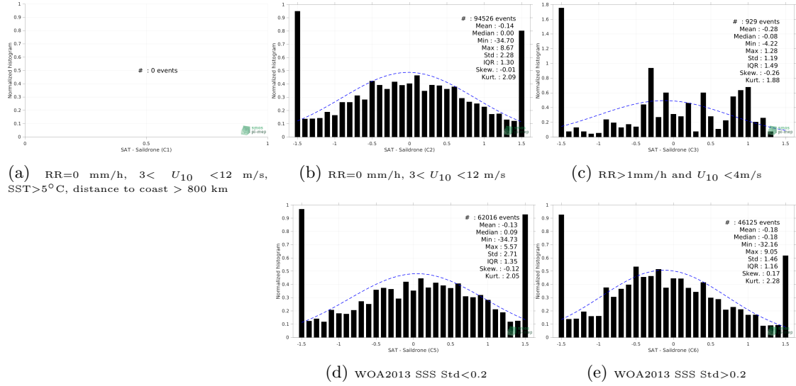
Figure 13: Normalized histogram of \Delta SSS (SMOS SSS L2Q v331 - With FLAG (CMEMS-CATDS-CPDC) - Saildrone) for 5 different subdatasets corresponding to: RR=0 mm/h, 3 < U_{10} < 12 m/s, SST>5°C, distance to coast > 800 km (a), RR=0 mm/h, 3 < U_{10} < 12 m/s (b), RR>1mm/h and U_{10} < 4 m/s (c), WOA2013 SSS Std<0.2 (d), WOA2013 SSS Std>0.2 (e).
