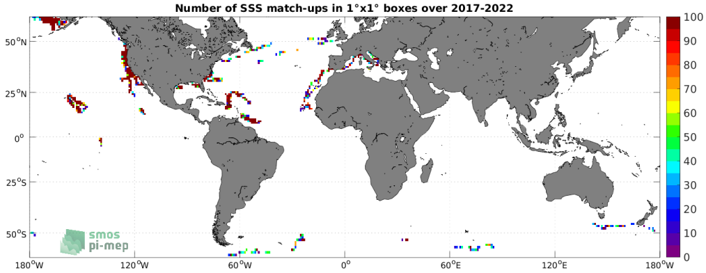
Figure 4: Number of SSS match-ups between Saildrone SSS and the SMOS SSS L2Q v331 - With FLAG (CMEMS-CATDS-CPDC) SSS product for the SMOS coastal zone (<800km) 60N-60S Pi-MEP region over 1^\circ \times 1^\circ boxes and for the full satellite product period.
