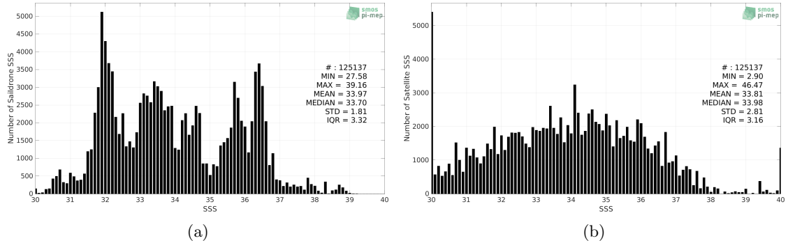
Figure 2: Histograms of SSS from Sairdrone (a) and SMOS SSS L2Q v331 - With FLAG (CMEMS-CATDS-CPDC) (b) considering all match-up pairs per bins of 0.1 over the SMOS coastal zone (<800km) 60N-60S Pi-MEP region and for the full satellite product period.
