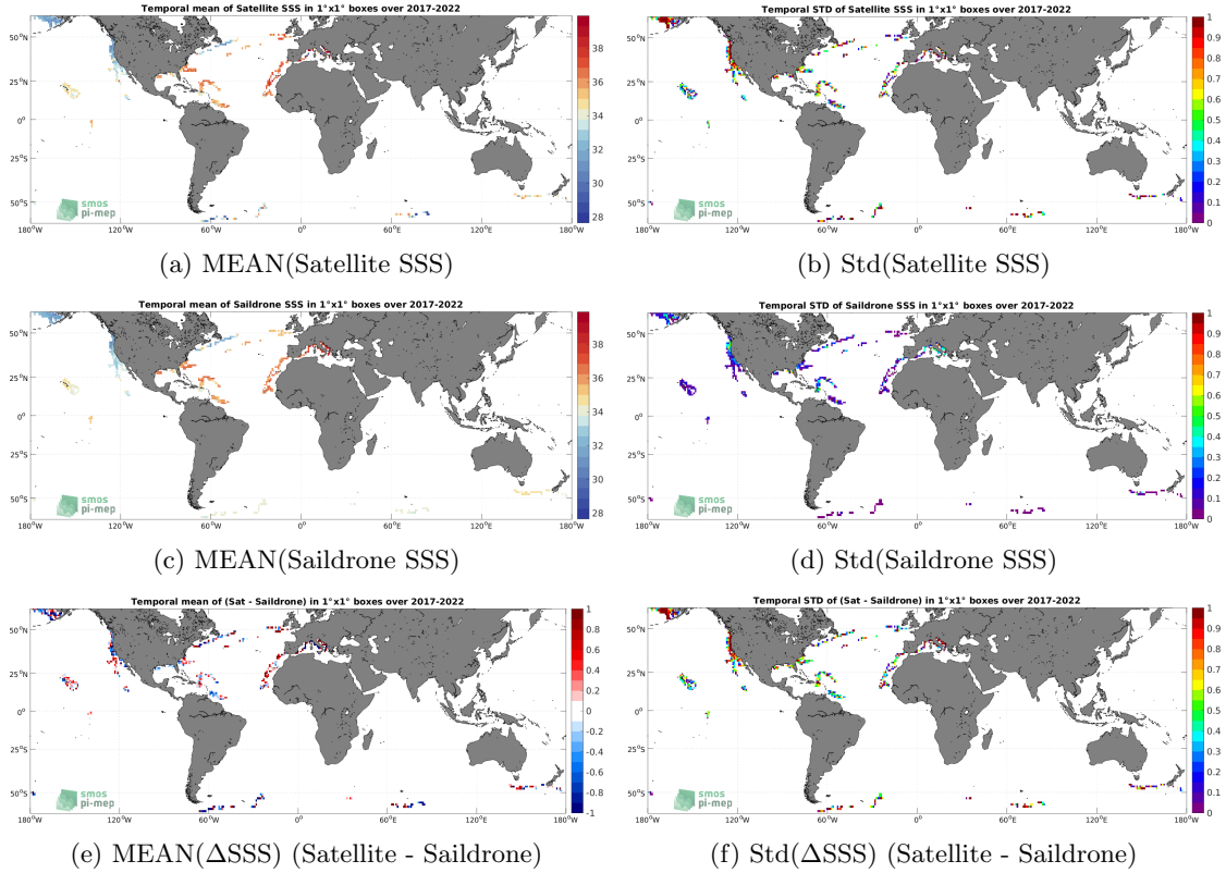
Figure 6: Temporal mean (left) and Std (right) of SSS from SMOS SSS L2Q v331 - With FLAG (CMEMS-CATDS-CPDC) (top), Saildrone (middle), and of \Delta SSS (Satellite - Saildrone). Only match-up pairs are used to generate these maps.
