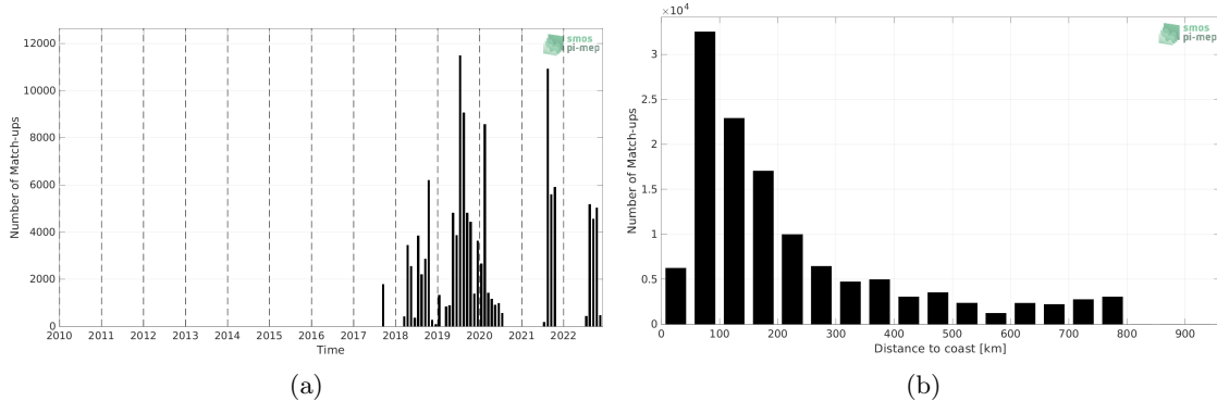
Figure 1: Number of match-ups between Saildrone and SMOS SSS L2Q v331 - With FLAG (CMEMS-CATDS-CPDC) SSS as a function of time (a) and as function of the distance to coast (b) over the SMOS coastal zone (<800km) 60N-60S Pi-MEP region and for the full satellite product period.
