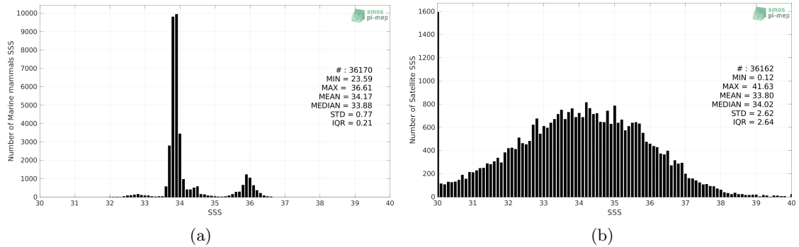
Figure 2: Histograms of SSS from Marine mammals (a) and SMOS SSS L2Q v331 - With FLAG (CMEMS-CATDS-CPDC) (b) considering all match-up pairs per bins of 0.1 over the SMOS coastal zone (<800km) 60N-60S Pi-MEP region and for the full satellite product period.
