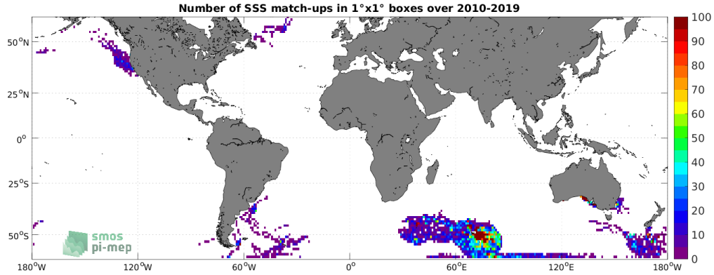
Figure 4: Number of SSS match-ups between Marine mammals SSS and the SMOS SSS L2Q v331 - With FLAG (CMEMS-CATDS-CPDC) SSS product for the SMOS coastal zone ( <800\text{km} ) 60N-60S Pi-MEP region over 1^\circ \times 1^\circ boxes and for the full satellite product period.
