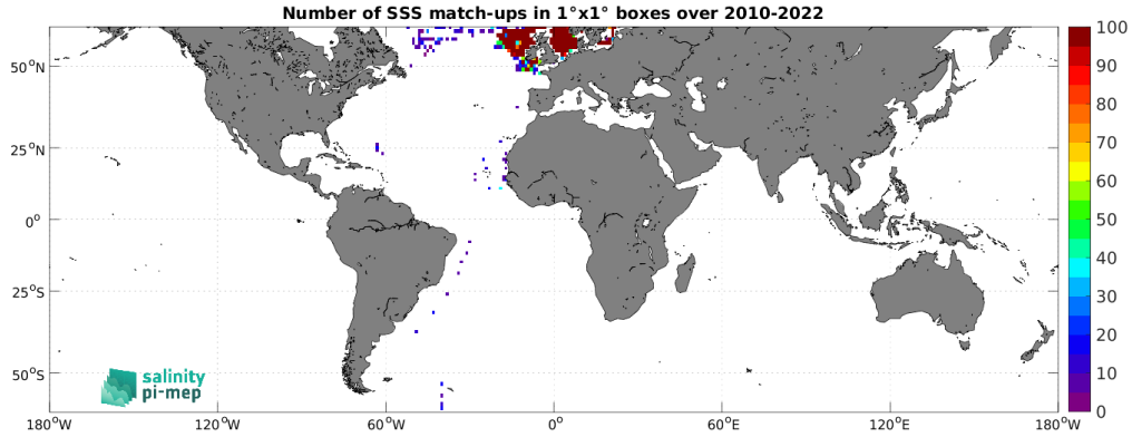
Figure 5: Number of SSS match-ups between ICES SSS and the SMOS SSS L2Q v331 - With FLAG (CMEMS-CATDS-CPDC) SSS product for the SMOS coastal zone (<800km) 60N-60S Pi-MEP region over 1^{\circ} \times 1^{\circ} boxes and for the full satellite product period.
