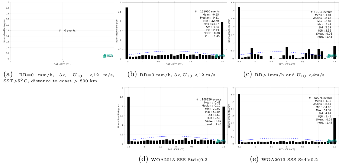
Figure 15: Normalized histogram of \Delta SSS (SMOS SSS L2Q v331 - With FLAG (CMEMS-CATDS-CPDC) - ICES) for 5 different subdatasets corresponding to: RR=0 mm/h, 3 < U_{10} < 12 m/s, SST>5°C, distance to coast > 800 km (a), RR=0 mm/h, 3 < U_{10} < 12 m/s (b), RR>1mm/h and U_{10} < 4 m/s (c), WOA2013 SSS Std<0.2 (d), WOA2013 SSS Std>0.2 (e).
