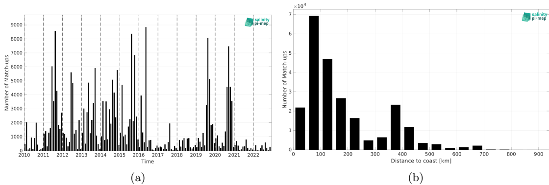
Figure 2: Number of match-ups between ICES and SMOS SSS L2Q v331 - With FLAG (CMEMS-CATDS-CPDC) SSS as a function of time (a) and as function of the distance to coast (b) over the SMOS coastal zone (<800km) 60N-60S Pi-MEP region and for the full satellite product period.
