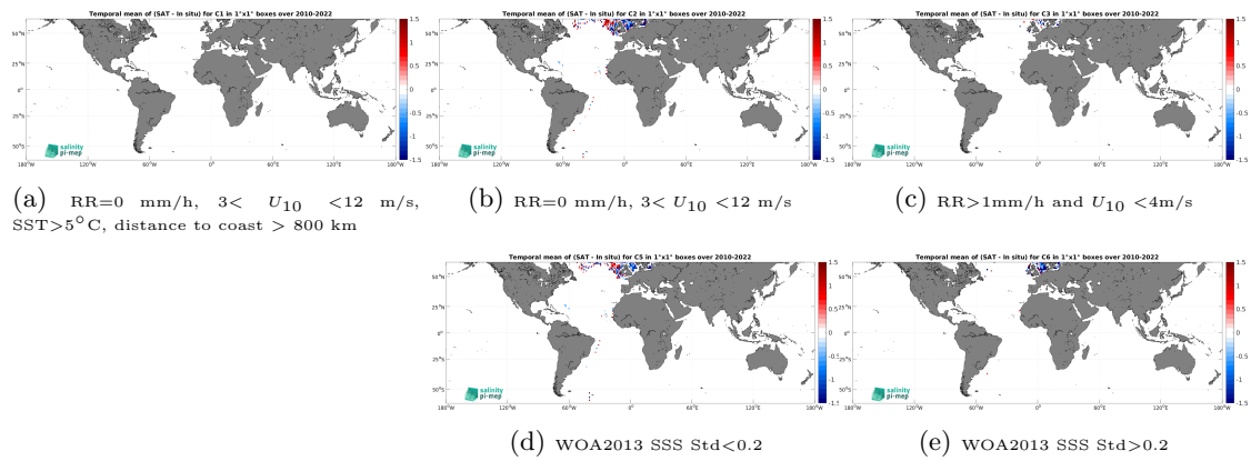
Figure 14: Temporal mean gridded over spatial boxes of size 1^\circ \times 1^\circ of \Delta\text{SSS} (SMOS SSS L2Q v331 - With FLAG (CMEMS-CATDS-CPDC) - ICES) for 5 different subdatasets corresponding to: RR=0 mm/h, 3 < U_{10} < 12 m/s, SST > 5^\circ\text{C} , distance to coast > 800 km (a), RR=0 mm/h, 3 < U_{10} < 12 m/s (b), RR > 1 mm/h and U_{10} < 4 m/s (c), WOA2013 SSS Std < 0.2 (d), WOA2013 SSS Std > 0.2 (e).
