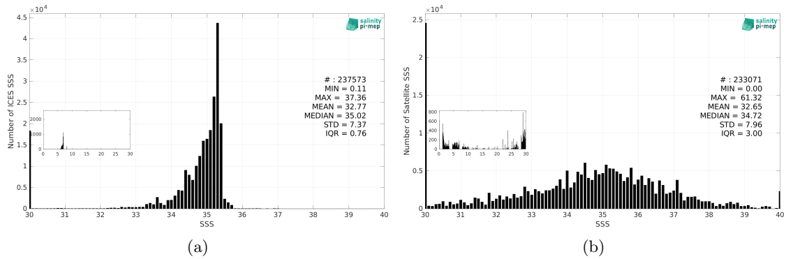
Figure 3: Histograms of SSS from ICES (a) and SMOS SSS L2Q v331 - With FLAG (CMEMS-CATDS-CPDC) (b) considering all match-up pairs per bins of 0.1 over the SMOS coastal zone (<800km) 60N-60S Pi-MEP region and for the full satellite product period.
