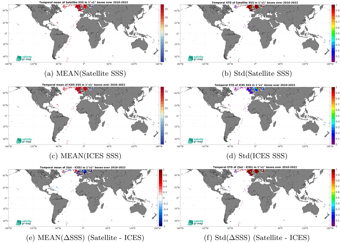
Figure 7: Temporal mean (left) and Std (right) of SSS from SMOS SSS L2Q v331 - With FLAG (CMEMS-CATDS-CPDC) (top), ICES (middle), and of \Delta SSS (Satellite - ICES). Only match-up pairs are used to generate these maps.
