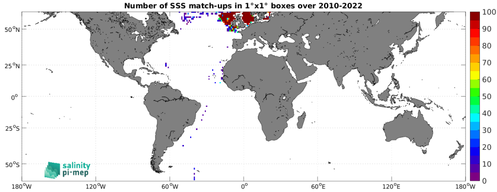
Figure 4: Number of SSS match-ups between ICES SSS and the SMOS SSS L2Q v331 - With FLAG (CMEMS-CATDS-CPDC) SSS product for the SMOS coastal zone ( <800\text{km} ) 60N-60S Pi-MEP region over 1^\circ \times 1^\circ boxes and for the full satellite product period.
