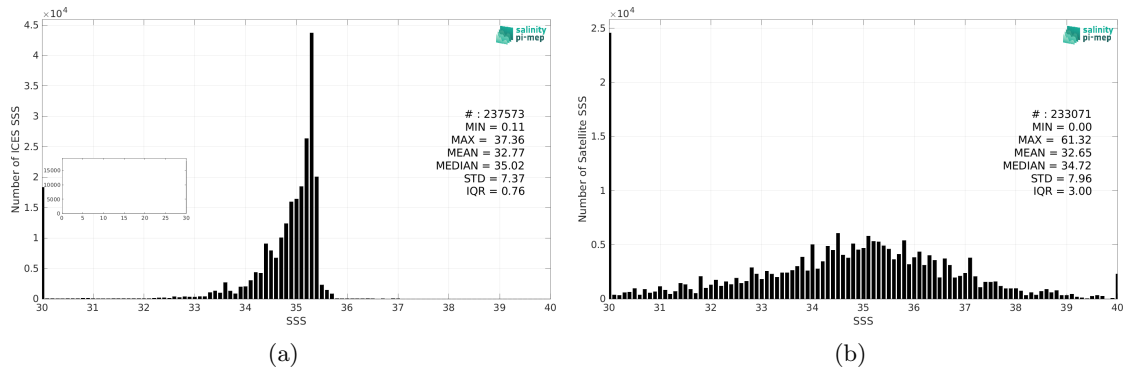
Figure 2: Histograms of SSS from ICES (a) and SMOS SSS L2Q v331 - With FLAG (CMEMS-CATDS-CPDC) (b) considering all match-up pairs per bins of 0.1 over the SMOS coastal zone (<800km) 60N-60S Pi-MEP region and for the full satellite product period.
