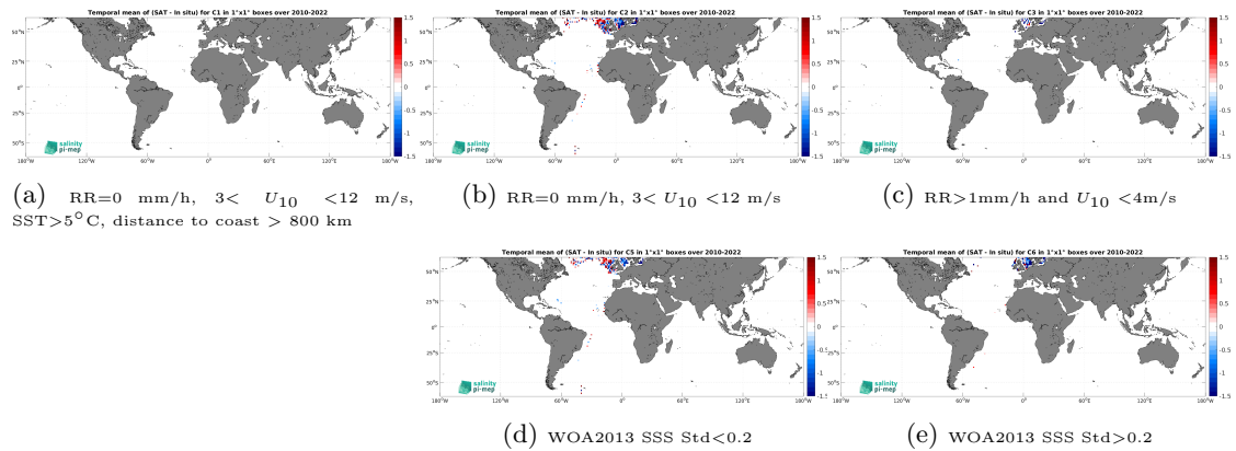
Figure 12: Temporal mean gridded over spatial boxes of size 1^\circ \times 1^\circ of \Delta\text{SSS} (SMOS SSS L2Q v331 - With FLAG (CMEMS-CATDS-CPDC) - ICES) for 5 different subdatasets corresponding to:RR=0 mm/h, 3 < U_{10} < 12 m/s, SST >5^\circ\text{C} , distance to coast > 800 km (a), RR=0 mm/h, 3 < U_{10} < 12 m/s (b), RR >1 mm/h and U_{10} < 4 m/s (c), WOA2013 SSS Std <0.2 (d), WOA2013 SSS Std >0.2 (e).
