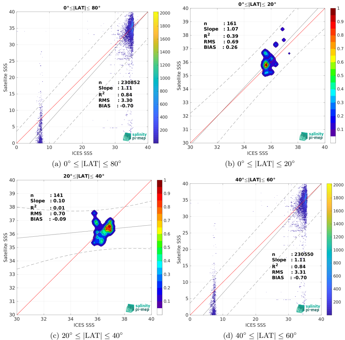
Figure 9: Contour maps of the concentration of SMOS SSS L2Q v331 - With FLAG (CMEMS-CATDS-CPDC) SSS ( y -axis) versus ICES SSS ( x -axis) at match-up pairs for different latitude bands. For each plot, the red line shows x=y . The black thin and dashed lines indicate a linear fit through the data cloud and the \pm 95\% confidence levels, respectively. The number match-up pairs n , the slope and R^2 coefficient of the linear fit, the root mean square (RMS) and the mean bias between satellite and in situ data are indicated for each latitude band in each plots.
