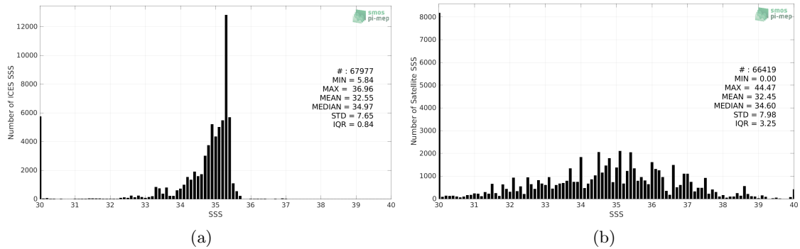
Figure 2: Histograms of SSS from ICES (a) and SMOS SSS L2Q v331 - With FLAG (CMEMS-CATDS-CPDC) (b) considering all match-up pairs per bins of 0.1 over the SMOS coastal zone (<800km) 60N-60S Pi-MEP region and for the full satellite product period.
