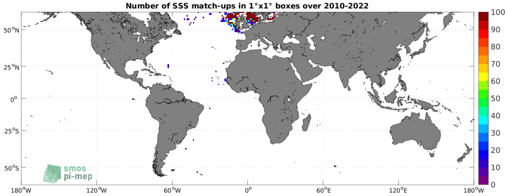
Figure 4: Number of SSS match-ups between ICES SSS and the SMOS SSS L2Q v331 - With FLAG (CMEMS-CATDS-CPDC) SSS product for the SMOS coastal zone (<800km) 60N-60S Pi-MEP region over 1^\circ \times 1^\circ boxes and for the full satellite product period.
