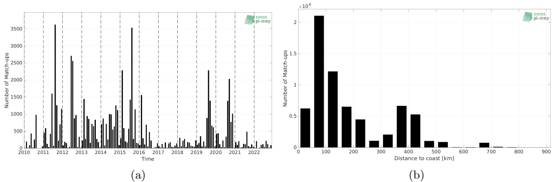
Figure 1: Number of match-ups between ICES and SMOS SSS L2Q v331 - With FLAG (CMEMS-CATDS-CPDC) SSS as a function of time (a) and as function of the distance to coast (b) over the SMOS coastal zone (<800km) 60N-60S Pi-MEP region and for the full satellite product period.
