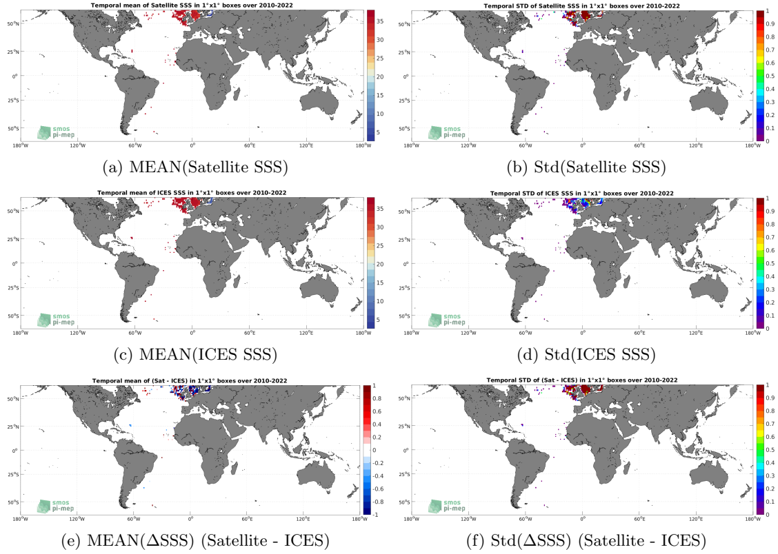
Figure 6: Temporal mean (left) and Std (right) of SSS from SMOS SSS L2Q v331 - With FLAG (CMEMS-CATDS-CPDC) (top), ICES (middle), and of \Delta SSS (Satellite - ICES). Only match-up pairs are used to generate these maps.
