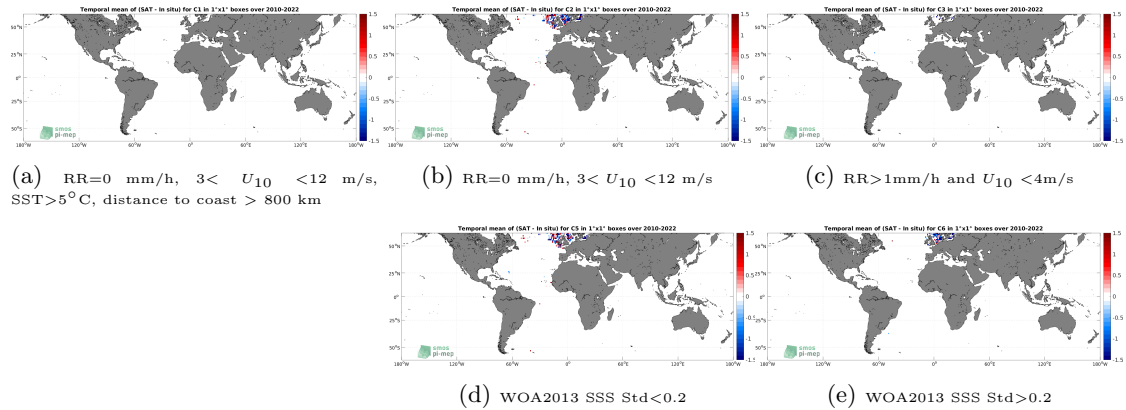
Figure 12: Temporal mean gridded over spatial boxes of size 1^\circ \times 1^\circ of \Delta SSS (SMOS SSS L2Q v331 - With FLAG (CMEMS-CATDS-CPDC) - ICES) for 5 different subdatasets corresponding to:RR=0 mm/h, 3 < U_{10} < 12 m/s, SST >5^\circ\text{C} , distance to coast > 800 km (a), RR=0 mm/h, 3 < U_{10} < 12 m/s (b), RR >1 mm/h and U_{10} < 4 m/s (c), WOA2013 SSS Std <0.2 (d), WOA2013 SSS Std >0.2 (e).
