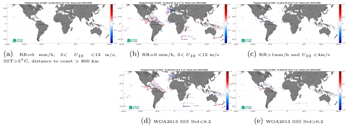
Figure 11: Temporal mean gridded over spatial boxes of size 1^\circ \times 1^\circ of \Delta\text{SSS} (SMOS SSS L2Q v331 - With FLAG (CMEMS-CATDS-CPDC) - Surface drifters) for 5 different subdatasets corresponding to:RR=0 mm/h, 3 < U_{10} < 12 m/s, SST >5^\circ\text{C} , distance to coast > 800 km (a), RR=0 mm/h, 3 < U_{10} < 12 m/s (b), RR >1 mm/h and U_{10} < 4 m/s (c), WOA2013 SSS Std <0.2 (d), WOA2013 SSS Std >0.2 (e).
