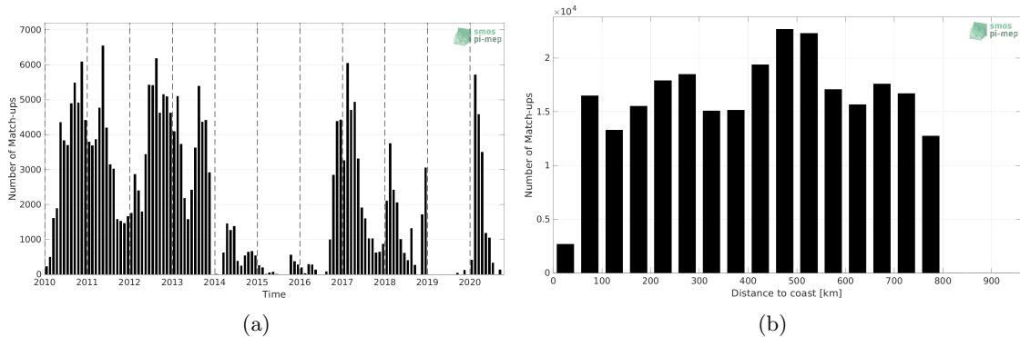
Figure 1: Number of match-ups between Surface drifters and SMOS SSS L2Q v331 - With FLAG (CMEMS-CATDS-CPDC) SSS as a function of time (a) and as function of the distance to coast (b) over the SMOS coastal zone (<800km) 60N-60S Pi-MEP region and for the full satellite product period.
