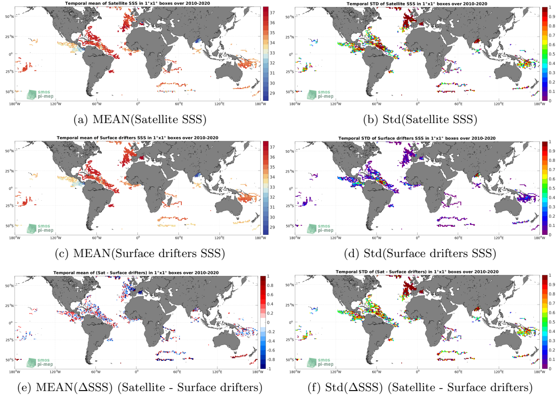
Figure 5: Temporal mean (left) and Std (right) of SSS from SMOS SSS L2Q v331 - With FLAG (CMEMS-CATDS-CPDC) (top), Surface drifters (middle), and of \Delta SSS (Satellite - Surface drifters). Only match-up pairs are used to generate these maps.
