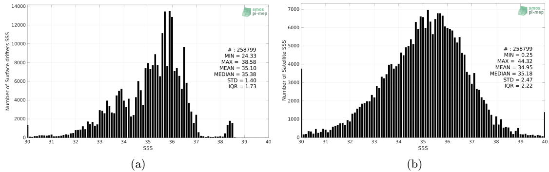
Figure 2: Histograms of SSS from Surface drifters (a) and SMOS SSS L2Q v331 - With FLAG (CMEMS-CATDS-CPDC) (b) considering all match-up pairs per bins of 0.1 over the SMOS coastal zone (<800km) 60N-60S Pi-MEP region and for the full satellite product period.
