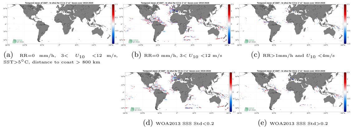
Figure 11: Temporal mean gridded over spatial boxes of size 1^\circ \times 1^\circ of \Delta SSS (SMOS SSS L2Q v331 - With FLAG (CMEMS-CATDS-CPDC) - Surface drifters) for 5 different subdatasets corresponding to:RR=0 mm/h, 3 < U_{10} < 12 m/s, SST >5^\circ C, distance to coast > 800 km (a), RR=0 mm/h, 3 < U_{10} < 12 m/s (b), RR >1 mm/h and U_{10} < 4 m/s (c), WOA2013 SSS Std <0.2 (d), WOA2013 SSS Std >0.2 (e).
