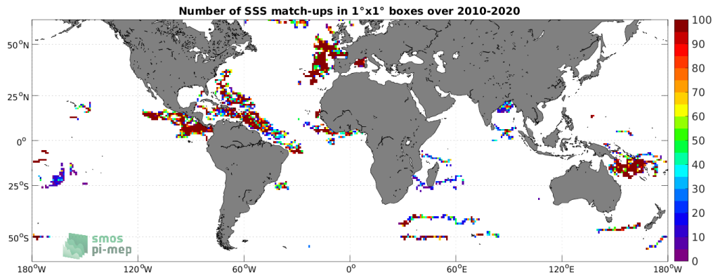
Figure 3: Number of SSS match-ups between Surface drifters SSS and the SMOS SSS L2Q v331 - With FLAG (CMEMS-CATDS-CPDC) SSS product for the SMOS coastal zone (<800km) 60N-60S Pi-MEP region over 1^\circ \times 1^\circ boxes and for the full satellite product period.
