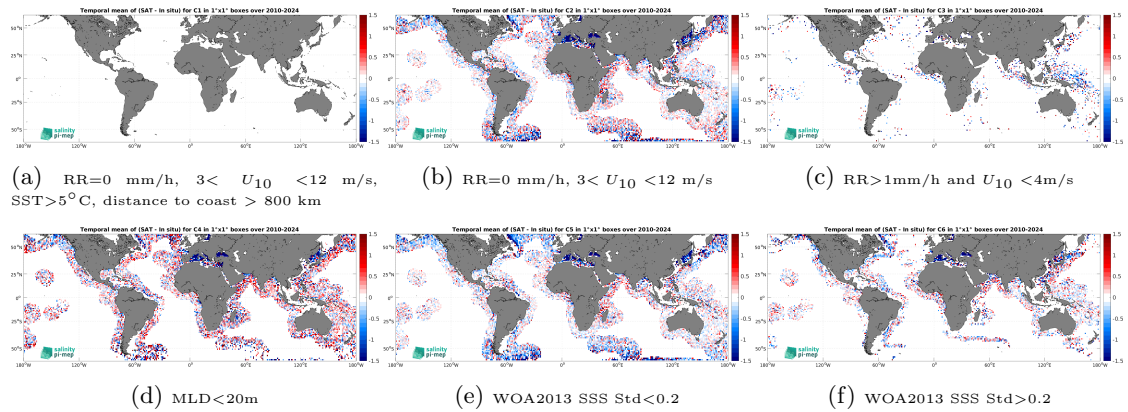
Figure 14: Temporal mean gridded over spatial boxes of size 1^\circ \times 1^\circ of \Delta SSS (SMOS SSS L2Q v331 - With FLAG (CMEMS-CATDS-CPDC) - Argo) for 6 different subdatasets corresponding to:RR=0 mm/h, 3 < U_{10} < 12 m/s, SST >5^\circ C, distance to coast > 800 km (a), RR=0 mm/h, 3 < U_{10} < 12 m/s (b), RR >1 mm/h and U_{10} < 4 m/s (c),MLD <20 m (d),WOA2013 SSS Std <0.2 (e),WOA2013 SSS Std >0.2 (f).
