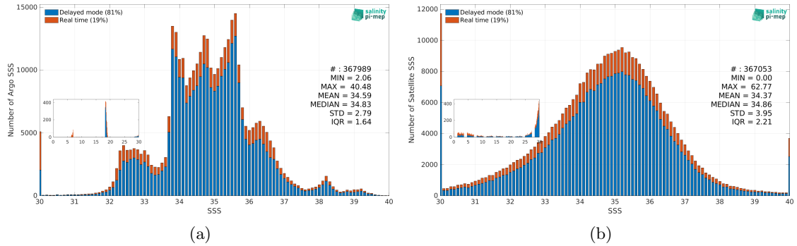
Figure 3: Histograms of SSS from Argo (a) and SMOS SSS L2Q v331 - With FLAG (CMEMS-CATDS-CPDC) (b) considering all match-up pairs per bins of 0.1 over the SMOS coastal zone (<800km) 60N-60S Pi-MEP region and for the full satellite product period.
