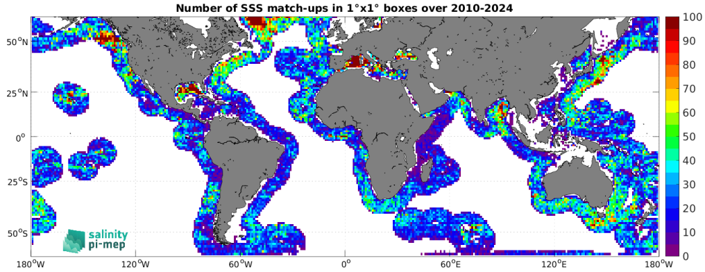
Figure 5: Number of SSS match-ups between Argo SSS and the SMOS SSS L2Q v331 - With FLAG (CMEMS-CATDS-CPDC) SSS product for the SMOS coastal zone (<800km) 60N-60S Pi-MEP region over 1^\circ \times 1^\circ boxes and for the full satellite product period.
