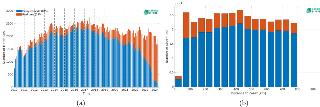
Figure 2: Number of match-ups between Argo and SMOS SSS L2Q v331 - With FLAG (CMEMS-CATDS-CPDC) SSS as a function of time (a) and as function of the distance to coast (b) over the SMOS coastal zone (<800km) 60N-60S Pi-MEP region and for the full satellite product period.
