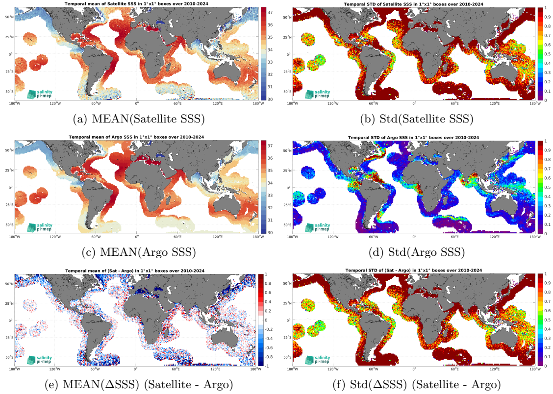
Figure 7: Temporal mean (left) and Std (right) of SSS from SMOS SSS L2Q v331 - With FLAG (CMEMS-CATDS-CPDC) (top), Argo (middle), and of \Delta SSS (Satellite - Argo). Only match-up pairs are used to generate these maps.
