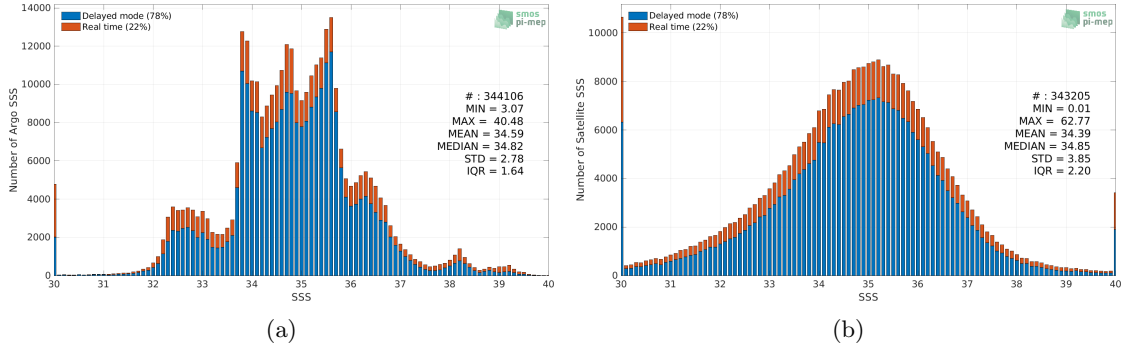
Figure 2: Histograms of SSS from Argo (a) and SMOS SSS L2Q v331 - With FLAG (CMEMS-CATDS-CPDC) (b) considering all match-up pairs per bins of 0.1 over the SMOS coastal zone (<800km) 60N-60S Pi-MEP region and for the full satellite product period.
