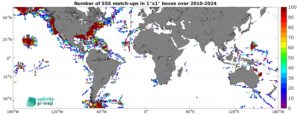
Figure 5: Number of SSS match-ups between TSG (SAMOS) SSS and the SMOS SSS L2Q v331 - No FLAG (CMEMS-CATDS-CPDC) SSS product for the SMOS coastal zone (<800km) 60N-60S Pi-MEP region over 1^\circ \times 1^\circ boxes and for the full satellite product period.
