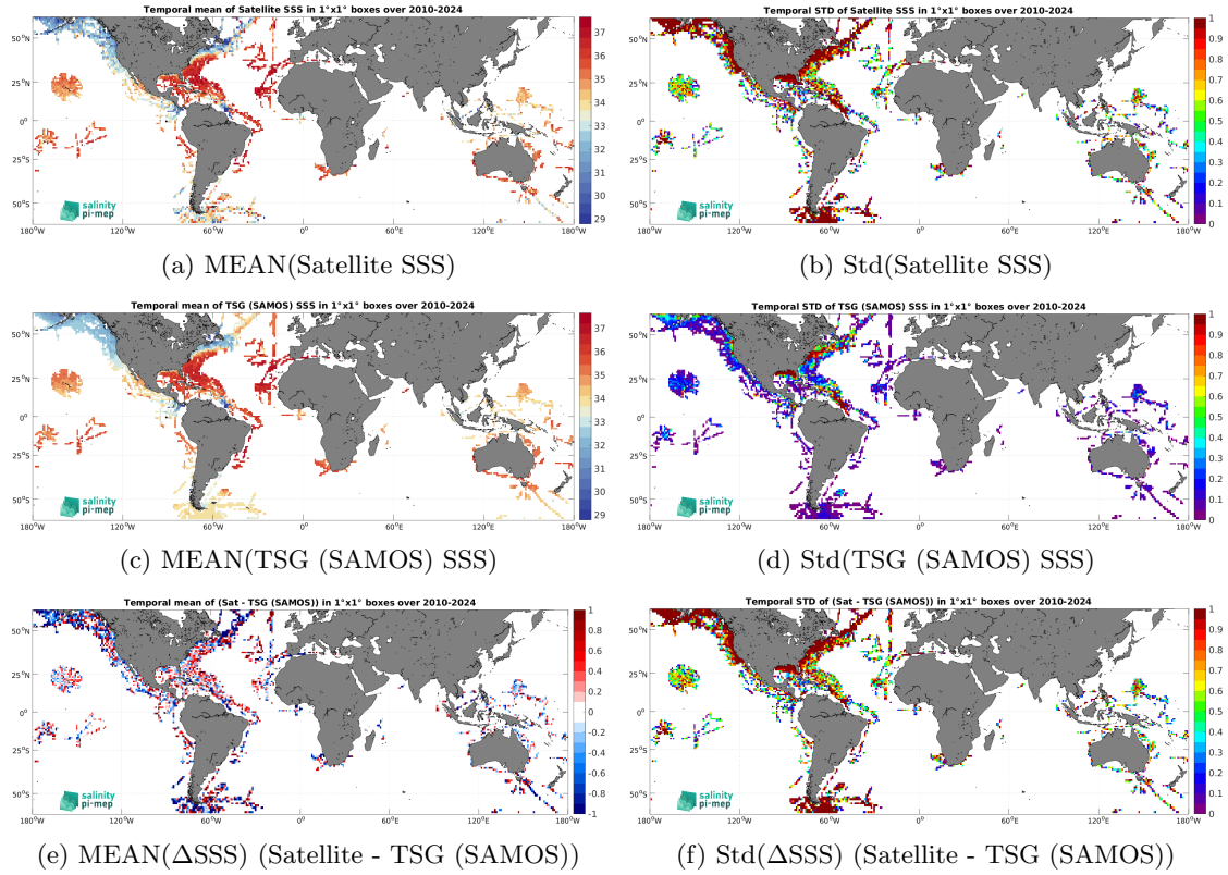
Figure 7: Temporal mean (left) and Std (right) of SSS from SMOS SSS L2Q v331 - No FLAG (CMEMS-CATDS-CPDC) (top), TSG (SAMOS) (middle), and of \Delta SSS (Satellite - TSG (SAMOS)). Only match-up pairs are used to generate these maps.
