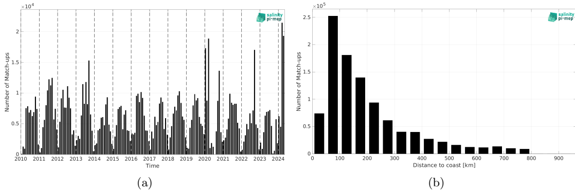
Figure 2: Number of match-ups between TSG (SAMOS) and SMOS SSS L2Q v331 - No FLAG (CMEMS-CATDS-CPDC) SSS as a function of time (a) and as function of the distance to coast (b) over the SMOS coastal zone (<800km) 60N-60S Pi-MEP region and for the full satellite product period.
