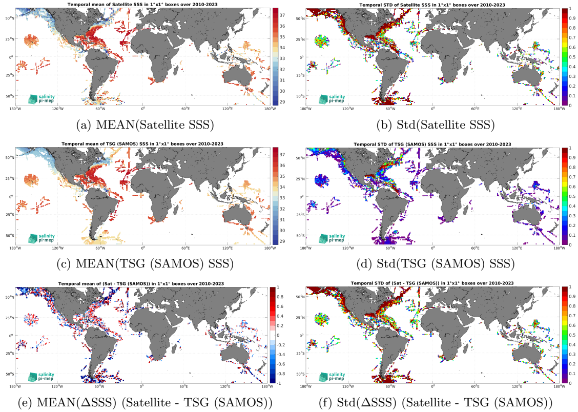
Figure 6: Temporal mean (left) and Std (right) of SSS from SMOS SSS L2Q v331 - No FLAG (CMEMS-CATDS-CPDC) (top), TSG (SAMOS) (middle), and of \Delta SSS (Satellite - TSG (SAMOS)). Only match-up pairs are used to generate these maps.
