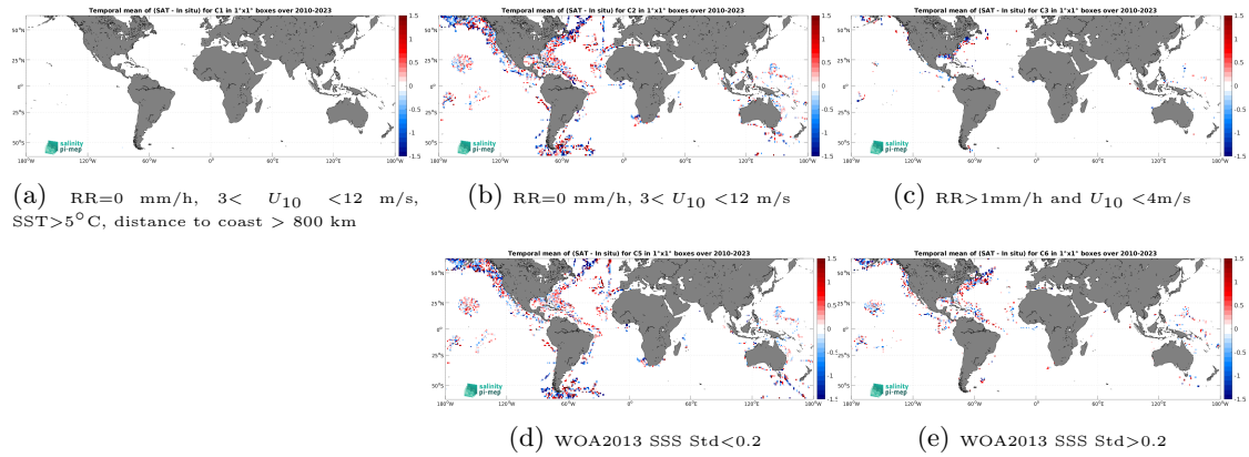
Figure 12: Temporal mean gridded over spatial boxes of size 1^\circ \times 1^\circ of \Delta SSS (SMOS SSS L2Q v331 - No FLAG (CMEMS-CATDS-CPDC) - TSG (SAMOS)) for 5 different subdatasets corresponding to:RR=0 mm/h, 3 < U_{10} < 12 m/s, SST >5^\circ\text{C} , distance to coast > 800 km (a), RR=0 mm/h, 3 < U_{10} < 12 m/s (b), RR >1 mm/h and U_{10} < 4 m/s (c), WOA2013 SSS Std <0.2 (d), WOA2013 SSS Std >0.2 (e).
