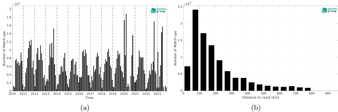
Figure 1: Number of match-ups between TSG (SAMOS) and SMOS SSS L2Q v331 - No FLAG (CMEMS-CATDS-CPDC) SSS as a function of time (a) and as function of the distance to coast (b) over the SMOS coastal zone (<800km) 60N-60S Pi-MEP region and for the full satellite product period.
