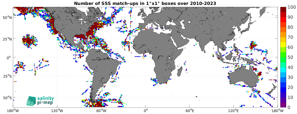
Figure 4: Number of SSS match-ups between TSG (SAMOS) SSS and the SMOS SSS L2Q v331 - No FLAG (CMEMS-CATDS-CPDC) SSS product for the SMOS coastal zone (<800km) 60N-60S Pi-MEP region over 1^\circ \times 1^\circ boxes and for the full satellite product period.
