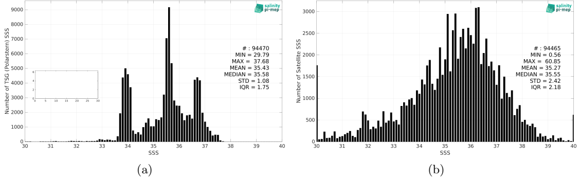
Figure 2: Histograms of SSS from TSG (Polarstern) (a) and SMOS SSS L2Q v331 - No FLAG (CMEMS-CATDS-CPDC) (b) considering all match-up pairs per bins of 0.1 over the SMOS coastal zone (<800km) 60N-60S Pi-MEP region and for the full satellite product period.
