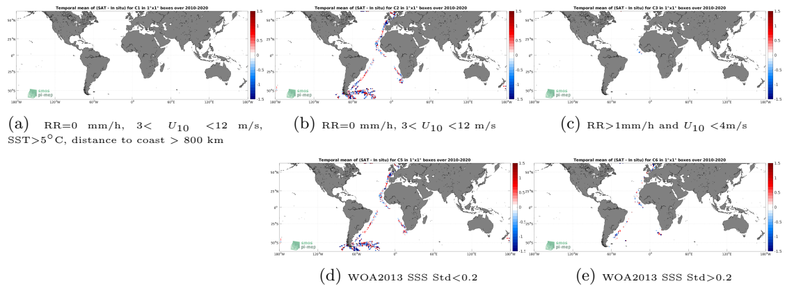
Figure 12: Temporal mean gridded over spatial boxes of size 1^\circ \times 1^\circ of \Delta SSS (SMOS SSS L2Q v331 - No FLAG (CMEMS-CATDS-CPDC) - TSG (Polarstern)) for 5 different subdatasets corresponding to:RR=0 mm/h, 3 < U_{10} < 12 m/s, SST >5^\circ C, distance to coast > 800 km (a), RR=0 mm/h, 3 < U_{10} < 12 m/s (b), RR >1 mm/h and U_{10} < 4 m/s (c), WOA2013 SSS Std <0.2 (d), WOA2013 SSS Std >0.2 (e).
