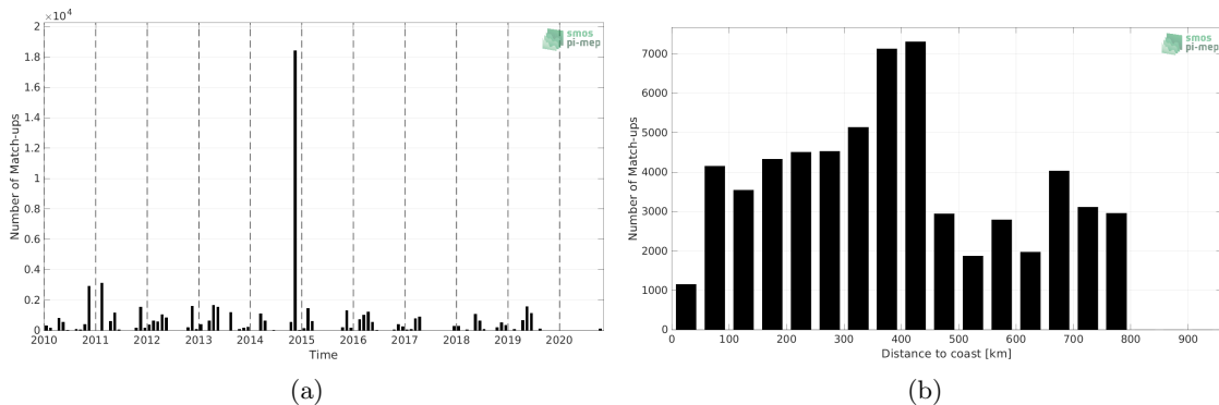
Figure 1: Number of match-ups between TSG (Polarstern) and SMOS SSS L2Q v331 - No FLAG (CMEMS-CATDS-CPDC) SSS as a function of time (a) and as function of the distance to coast (b) over the SMOS coastal zone (<800km) 60N-60S Pi-MEP region and for the full satellite product period.
