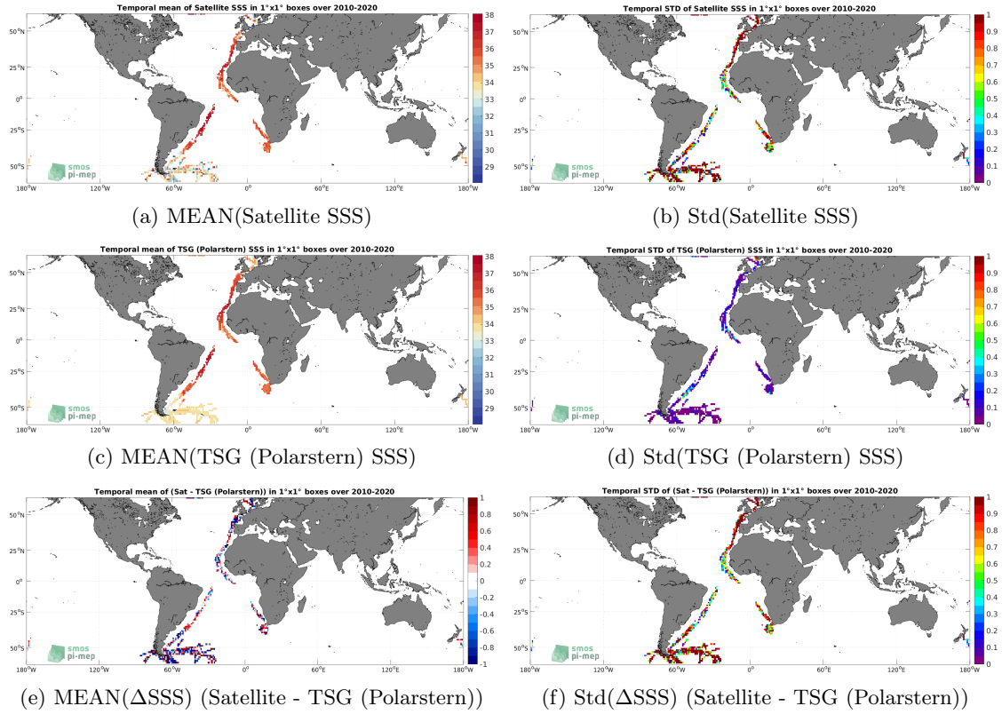
Figure 6: Temporal mean (left) and Std (right) of SSS from SMOS SSS L2Q v331 - No FLAG (CMEMS-CATDS-CPDC) (top), TSG (Polarstern) (middle), and of \Delta SSS (Satellite - TSG (Polarstern)). Only match-up pairs are used to generate these maps.
