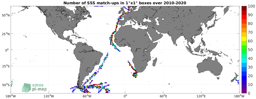
Figure 4: Number of SSS match-ups between TSG (Polarstern) SSS and the SMOS SSS L2Q v331 - No FLAG (CMEMS-CATDS-CPDC) SSS product for the SMOS coastal zone (<800km) 60N-60S Pi-MEP region over 1^\circ \times 1^\circ boxes and for the full satellite product period.
