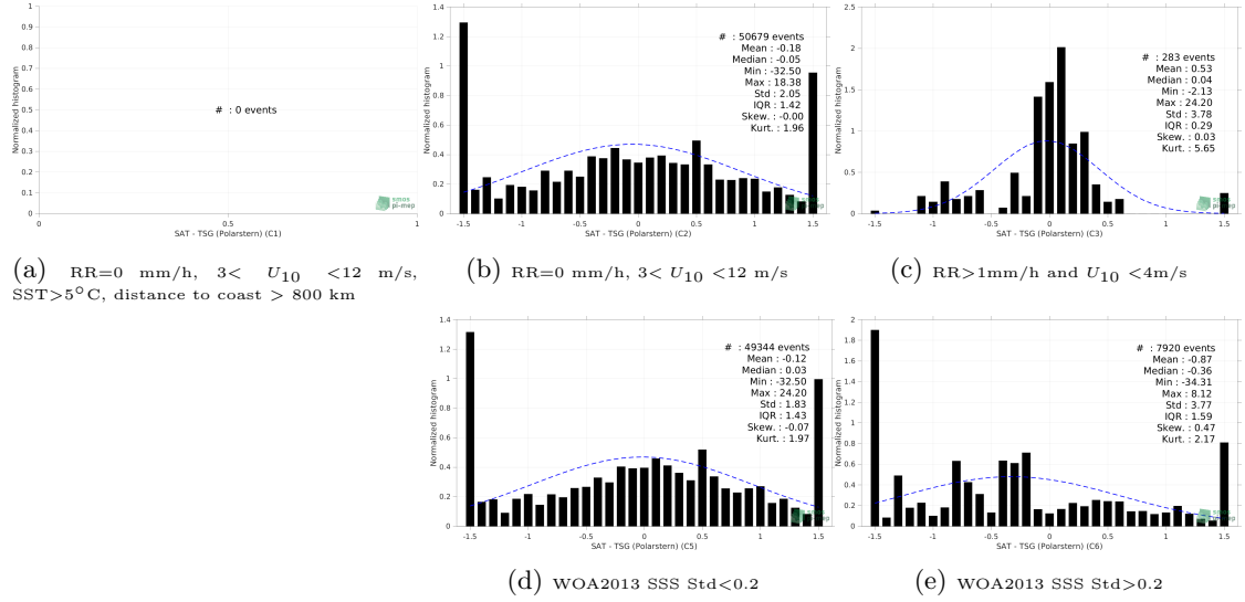
Figure 13: Normalized histogram of \Delta SSS (SMOS SSS L2Q v331 - No FLAG (CMEMS-CATDS-CPDC) - TSG (Polarstern)) for 5 different subdatasets corresponding to: RR=0 mm/h, 3 < U_{10} < 12 m/s, SST > 5°C, distance to coast > 800 km (a), RR=0 mm/h, 3 < U_{10} < 12 m/s (b), RR > 1mm/h and U_{10} < 4 m/s (c), WOA2013 SSS Std < 0.2 (d), WOA2013 SSS Std > 0.2 (e).
