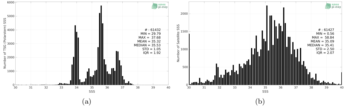
Figure 2: Histograms of SSS from TSG (Polarstern) (a) and SMOS SSS L2Q v331 - No FLAG (CMEMS-CATDS-CPDC) (b) considering all match-up pairs per bins of 0.1 over the SMOS coastal zone (<800km) 60N-60S Pi-MEP region and for the full satellite product period.
