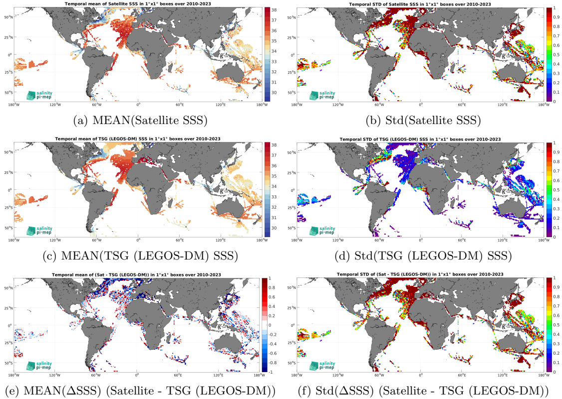
Figure 7: Temporal mean (left) and Std (right) of SSS from SMOS SSS L2Q v331 - No FLAG (CMEMS-CATDS-CPDC) (top), TSG (LEGOS-DM) (middle), and of \Delta\text{SSS} (Satellite - TSG (LEGOS-DM)). Only match-up pairs are used to generate these maps.
