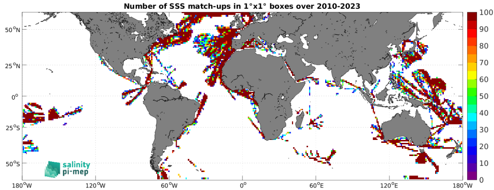
Figure 5: Number of SSS match-ups between TSG (LEGOS-DM) SSS and the SMOS SSS L2Q v331 - No FLAG (CMEMS-CATDS-CPDC) SSS product for the SMOS coastal zone ( <800\text{km} ) 60N-60S Pi-MEP region over 1^\circ \times 1^\circ boxes and for the full satellite product period.
