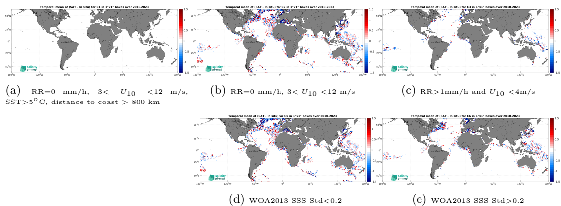
Figure 14: Temporal mean gridded over spatial boxes of size 1^\circ \times 1^\circ of \Delta\text{SSS} (SMOS SSS L2Q v331 - No FLAG (CMEMS-CATDS-CPDC) - TSG (LEGOS-DM)) for 5 different subdatasets corresponding to:RR=0 mm/h, 3 < U_{10} < 12 m/s, SST >5^\circ\text{C} , distance to coast > 800 km (a), RR=0 mm/h, 3 < U_{10} < 12 m/s (b), RR >1 mm/h and U_{10} < 4 m/s (c), WOA2013 SSS Std <0.2 (d), WOA2013 SSS Std >0.2 (e).
