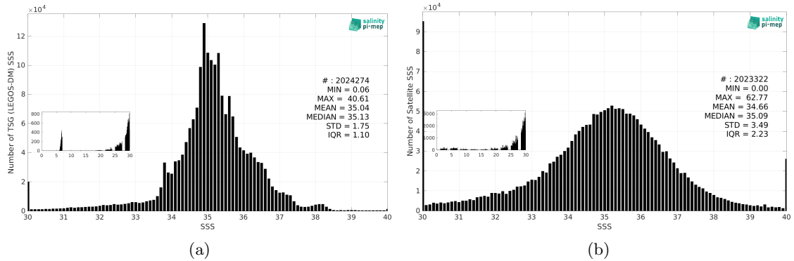
Figure 3: Histograms of SSS from TSG (LEGOS-DM) (a) and SMOS SSS L2Q v331 - No FLAG (CMEMS-CATDS-CPDC) (b) considering all match-up pairs per bins of 0.1 over the SMOS coastal zone (<800km) 60N-60S Pi-MEP region and for the full satellite product period.
