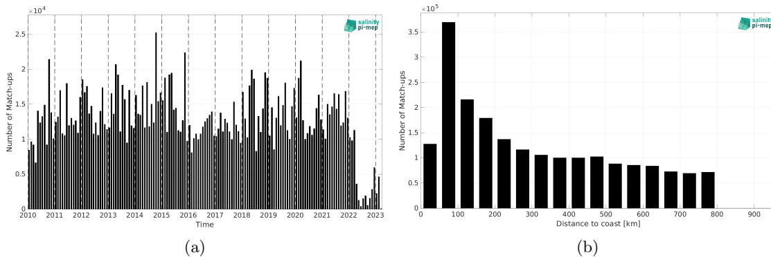
Figure 2: Number of match-ups between TSG (LEGOS-DM) and SMOS SSS L2Q v331 - No FLAG (CMEMS-CATDS-CPDC) SSS as a function of time (a) and as function of the distance to coast (b) over the SMOS coastal zone (<800km) 60N-60S Pi-MEP region and for the full satellite product period.
