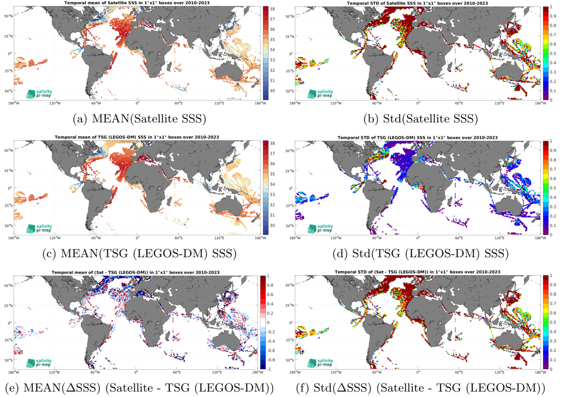
Figure 6: Temporal mean (left) and Std (right) of SSS from SMOS SSS L2Q v331 - No FLAG (CMEMS-CATDS-CPDC) (top), TSG (LEGOS-DM) (middle), and of \Delta\text{SSS} (Satellite - TSG (LEGOS-DM)). Only match-up pairs are used to generate these maps.
