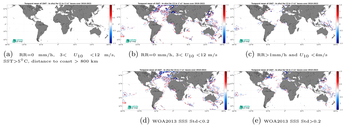
Figure 12: Temporal mean gridded over spatial boxes of size 1^\circ \times 1^\circ of \Delta SSS (SMOS SSS L2Q v331 - No FLAG (CMEMS-CATDS-CPDC) - TSG (LEGOS-DM)) for 5 different subdatasets corresponding to:RR=0 mm/h, 3 < U_{10} < 12 m/s, SST >5^\circ\text{C} , distance to coast > 800 km (a), RR=0 mm/h, 3 < U_{10} < 12 m/s (b), RR >1 mm/h and U_{10} < 4 m/s (c), WOA2013 SSS Std <0.2 (d), WOA2013 SSS Std >0.2 (e).
