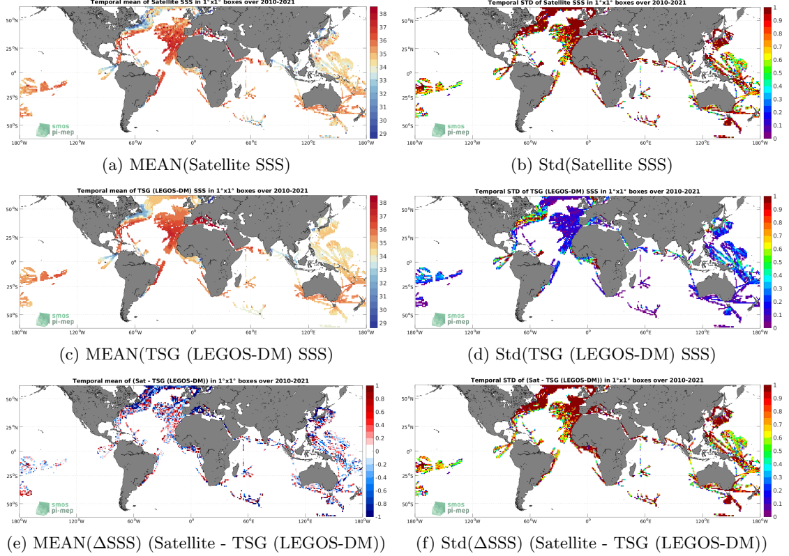
Figure 6: Temporal mean (left) and Std (right) of SSS from SMOS SSS L2Q v331 - No FLAG (CMEMS-CATDS-CPDC) (top), TSG (LEGOS-DM) (middle), and of \Delta SSS (Satellite - TSG (LEGOS-DM)). Only match-up pairs are used to generate these maps.
