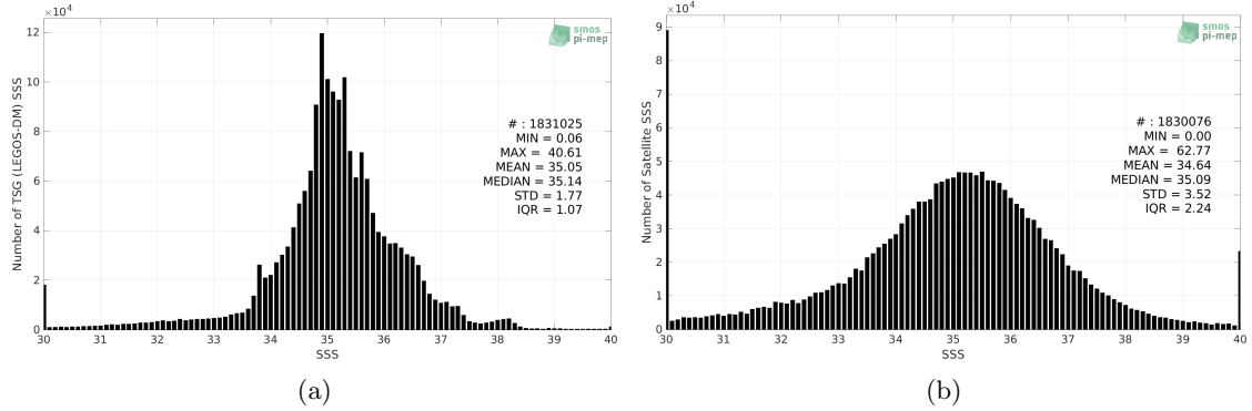
Figure 2: Histograms of SSS from TSG (LEGOS-DM) (a) and SMOS SSS L2Q v331 - No FLAG (CMEMS-CATDS-CPDC) (b) considering all match-up pairs per bins of 0.1 over the SMOS coastal zone (<800km) 60N-60S Pi-MEP region and for the full satellite product period.
