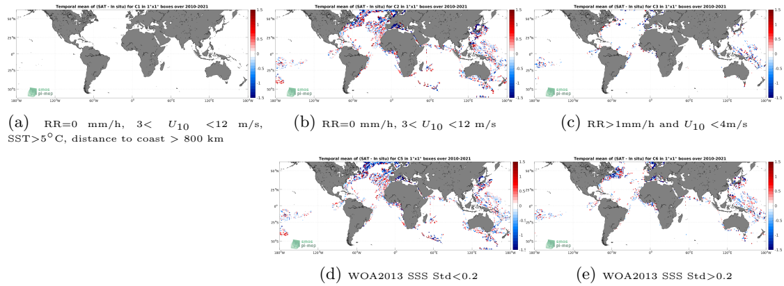
Figure 12: Temporal mean gridded over spatial boxes of size 1^\circ \times 1^\circ of \Delta\text{SSS} (SMOS SSS L2Q v331 - No FLAG (CMEMS-CATDS-CPDC) - TSG (LEGOS-DM)) for 5 different subdatasets corresponding to:RR=0 mm/h, 3 < U_{10} < 12 m/s, SST >5^\circ\text{C} , distance to coast > 800 km (a), RR=0 mm/h, 3 < U_{10} < 12 m/s (b), RR >1 mm/h and U_{10} < 4 m/s (c), WOA2013 SSS Std <0.2 (d), WOA2013 SSS Std >0.2 (e).
