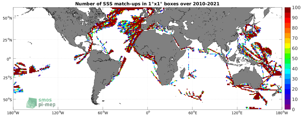
Figure 4: Number of SSS match-ups between TSG (LEGOS-DM) SSS and the SMOS SSS L2Q v331 - No FLAG (CMEMS-CATDS-CPDC) SSS product for the SMOS coastal zone ( <800\text{km} ) 60N-60S Pi-MEP region over 1^\circ \times 1^\circ boxes and for the full satellite product period.
