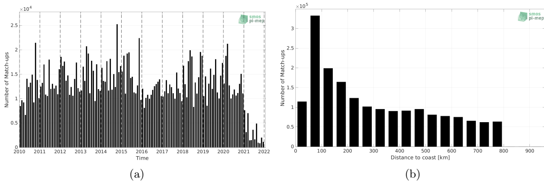
Figure 1: Number of match-ups between TSG (LEGOS-DM) and SMOS SSS L2Q v331 - No FLAG (CMEMS-CATDS-CPDC) SSS as a function of time (a) and as function of the distance to coast (b) over the SMOS coastal zone (<800km) 60N-60S Pi-MEP region and for the full satellite product period.
