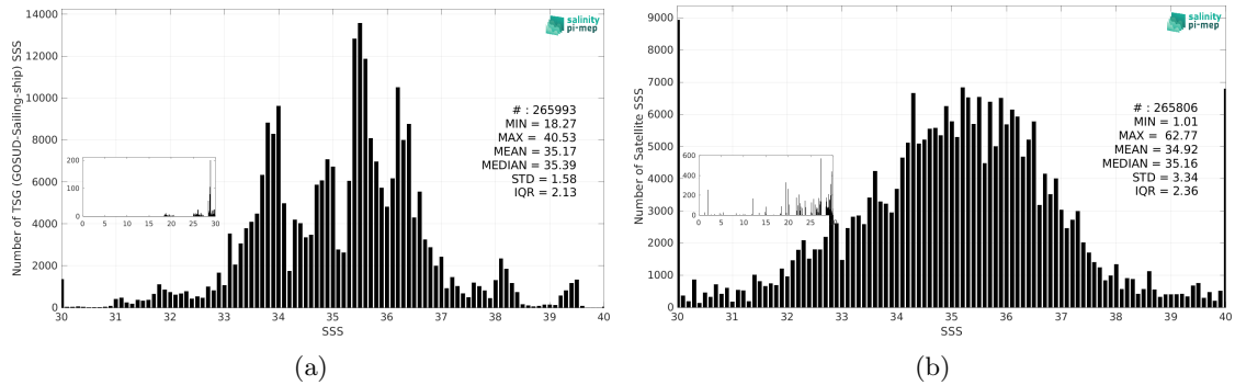
Figure 3: Histograms of SSS from TSG (GOSUD-Sailing-ship) (a) and SMOS SSS L2Q v331 - No FLAG (CMEMS-CATDS-CPDC) (b) considering all match-up pairs per bins of 0.1 over the SMOS coastal zone (<800km) 60N-60S Pi-MEP region and for the full satellite product period.
