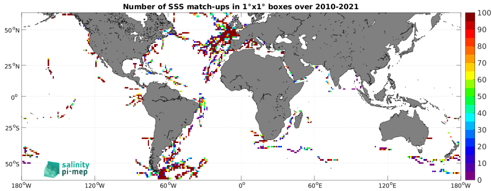
Figure 5: Number of SSS match-ups between TSG (GOSUD-Sailing-ship) SSS and the SMOS SSS L2Q v331 - No FLAG (CMEMS-CATDS-CPDC) SSS product for the SMOS coastal zone (<800km) 60N-60S Pi-MEP region over 1^\circ \times 1^\circ boxes and for the full satellite product period.
