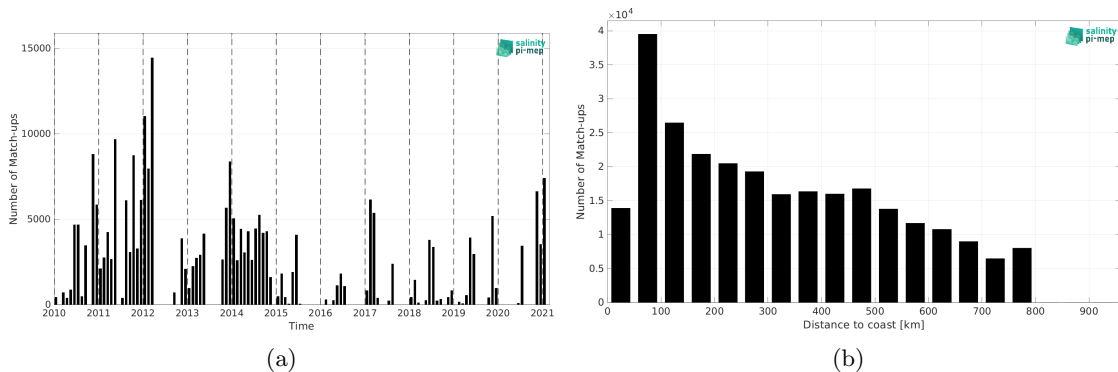
Figure 2: Number of match-ups between TSG (GOSUD-Sailing-ship) and SMOS SSS L2Q v331 - No FLAG (CMEMS-CATDS-CPDC) SSS as a function of time (a) and as function of the distance to coast (b) over the SMOS coastal zone (<800km) 60N-60S Pi-MEP region and for the full satellite product period.
