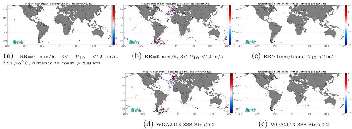
Figure 14: Temporal mean gridded over spatial boxes of size 1^\circ \times 1^\circ of \Delta\text{SSS} (SMOS SSS L2Q v331 - No FLAG (CMEMS-CATDS-CPDC) - TSG (GOSUD-Sailing-ship)) for 5 different sub-datasets corresponding to:RR=0 mm/h, 3 < U_{10} < 12 m/s, SST>5°C, distance to coast > 800 km (a), RR=0 mm/h, 3 < U_{10} < 12 m/s (b), RR>1mm/h and U_{10} < 4 m/s (c), WOA2013 SSS Std<0.2 (d), WOA2013 SSS Std>0.2 (e).
