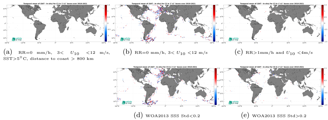
Figure 12: Temporal mean gridded over spatial boxes of size 1^\circ \times 1^\circ of \Delta\text{SSS} (SMOS SSS L2Q v331 - No FLAG (CMEMS-CATDS-CPDC) - TSG (GOSUD-Sailing-ship)) for 5 different sub-datasets corresponding to:RR=0 mm/h, 3 < U_{10} < 12 m/s, SST>5°C, distance to coast > 800 km (a), RR=0 mm/h, 3 < U_{10} < 12 m/s (b), RR>1mm/h and U_{10} < 4 m/s (c), WOA2013 SSS Std<0.2 (d), WOA2013 SSS Std>0.2 (e).
