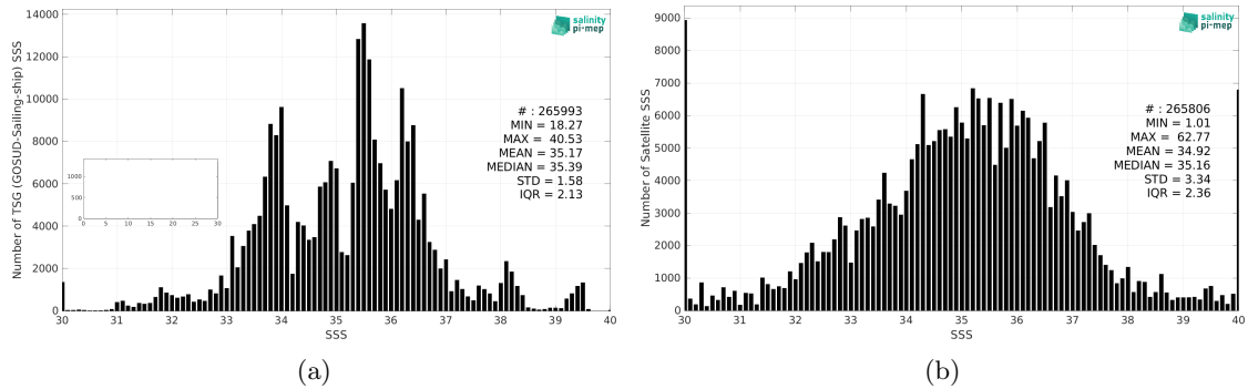
Figure 2: Histograms of SSS from TSG (GOSUD-Sailing-ship) (a) and SMOS SSS L2Q v331 - No FLAG (CMEMS-CATDS-CPDC) (b) considering all match-up pairs per bins of 0.1 over the SMOS coastal zone (<800km) 60N-60S Pi-MEP region and for the full satellite product period.
