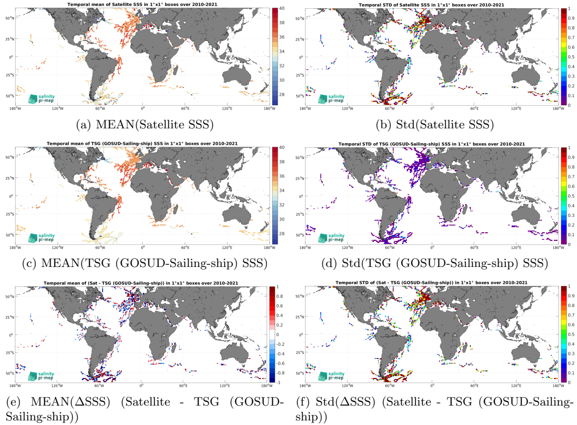
Figure 6: Temporal mean (left) and Std (right) of SSS from SMOS SSS L2Q v331 - No FLAG (CMEMS-CATDS-CPDC) (top), TSG (GOSUD-Sailing-ship) (middle), and of \Delta SSS (Satellite - TSG (GOSUD-Sailing-ship)). Only match-up pairs are used to generate these maps.
