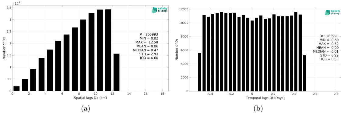
Figure 5: Histograms of the spatial (a) and temporal (b) lags between the location/time of the TSG (GOSUD-Sailing-ship) measurement and the date of the corresponding SMOS SSS L2Q v331 - No FLAG (CMEMS-CATDS-CPDC) SSS pixel.
