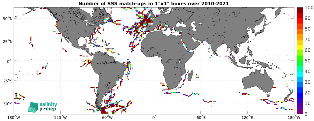
Figure 4: Number of SSS match-ups between TSG (GOSUD-Sailing-ship) SSS and the SMOS SSS L2Q v331 - No FLAG (CMEMS-CATDS-CPDC) SSS product for the SMOS coastal zone (<800km) 60N-60S Pi-MEP region over 1^{\circ} \times 1^{\circ} boxes and for the full satellite product period.
