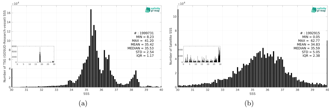
Figure 3: Histograms of SSS from TSG (GOSUD-Research-vessel) (a) and SMOS SSS L2Q v331 - No FLAG (CMEMS-CATDS-CPDC) (b) considering all match-up pairs per bins of 0.1 over the SMOS coastal zone (<800km) 60N-60S Pi-MEP region and for the full satellite product period.
