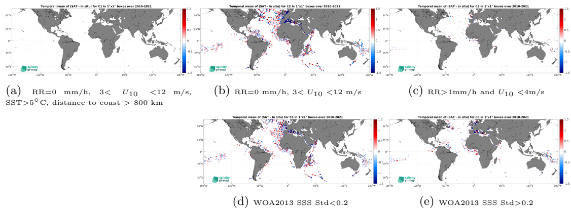
Figure 14: Temporal mean gridded over spatial boxes of size 1^\circ \times 1^\circ of \Delta SSS (SMOS SSS L2Q v331 - No FLAG (CMEMS-CATDS-CPDC) - TSG (GOSUD-Research-vessel)) for 5 different subdatasets corresponding to:RR=0 mm/h, 3 < U_{10} < 12 m/s, SST >5^\circ\text{C} , distance to coast > 800 km (a), RR=0 mm/h, 3 < U_{10} < 12 m/s (b), RR >1 mm/h and U_{10} < 4 m/s (c), WOA2013 SSS Std <0.2 (d), WOA2013 SSS Std >0.2 (e).
