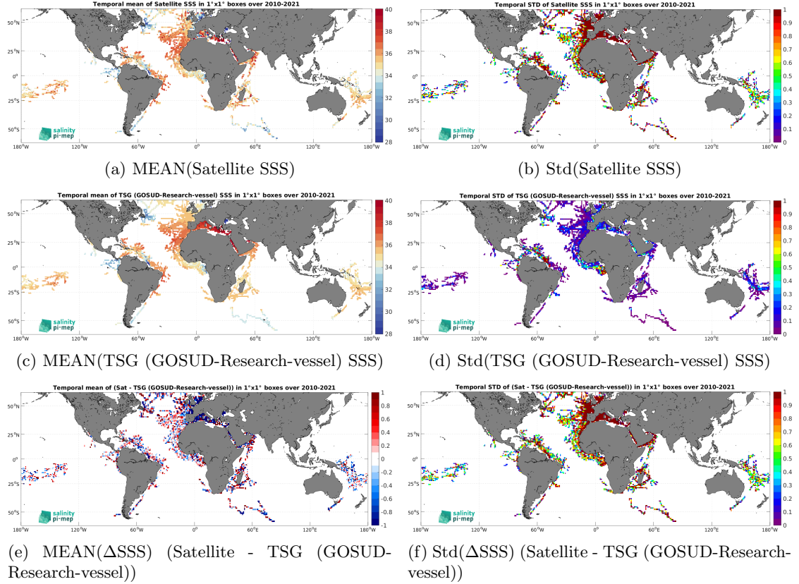
Figure 7: Temporal mean (left) and Std (right) of SSS from SMOS SSS L2Q v331 - No FLAG (CMEMS-CATDS-CPDC) (top), TSG (GOSUD-Research-vessel) (middle), and of \Delta\text{SSS} (Satellite - TSG (GOSUD-Research-vessel)). Only match-up pairs are used to generate these maps.
