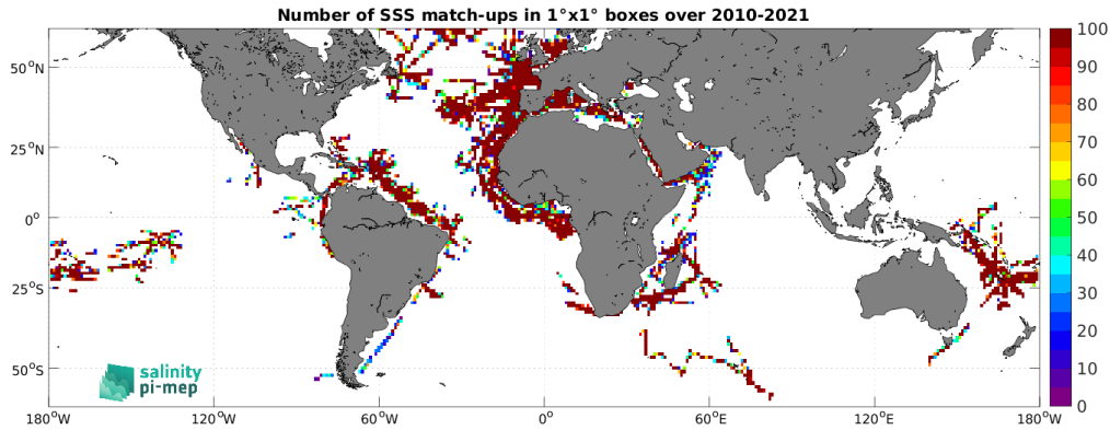
Figure 5: Number of SSS match-ups between TSG (GOSUD-Research-vessel) SSS and the SMOS SSS L2Q v331 - No FLAG (CMEMS-CATDS-CPDC) SSS product for the SMOS coastal zone (<800km) 60N-60S Pi-MEP region over 1^\circ \times 1^\circ boxes and for the full satellite product period.
