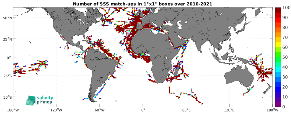
Figure 4: Number of SSS match-ups between TSG (GOSUD-Research-vessel) SSS and the SMOS SSS L2Q v331 - No FLAG (CMEMS-CATDS-CPDC) SSS product for the SMOS coastal zone (<800km) 60N-60S Pi-MEP region over 1^\circ \times 1^\circ boxes and for the full satellite product period.
