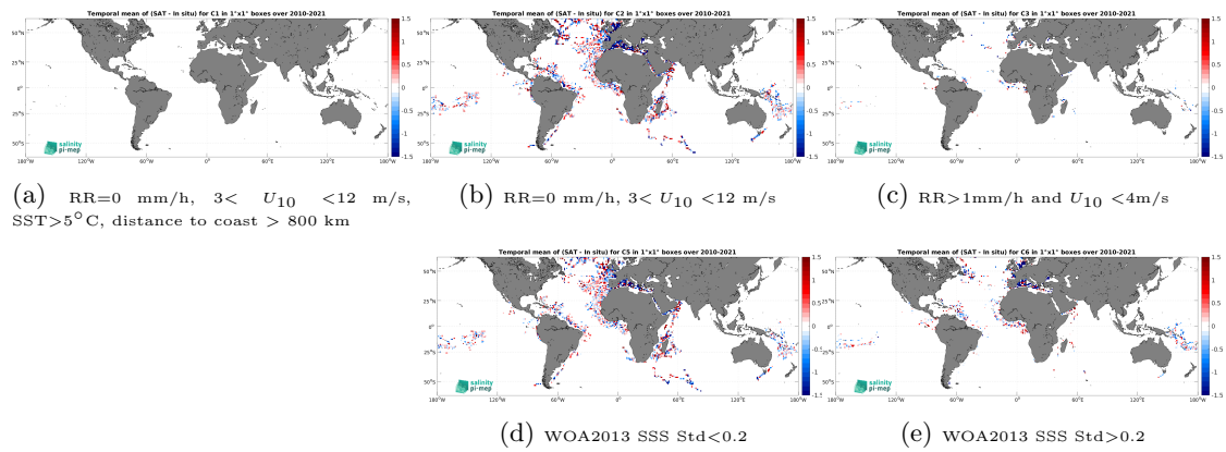
Figure 12: Temporal mean gridded over spatial boxes of size 1^\circ \times 1^\circ of \Delta SSS (SMOS SSS L2Q v331 - No FLAG (CMEMS-CATDS-CPDC) - TSG (GOSUD-Research-vessel)) for 5 different subdatasets corresponding to:RR=0 mm/h, 3 < U_{10} < 12 m/s, SST >5^\circ\text{C} , distance to coast > 800 km (a), RR=0 mm/h, 3 < U_{10} < 12 m/s (b), RR >1 mm/h and U_{10} < 4 m/s (c), WOA2013 SSS Std <0.2 (d), WOA2013 SSS Std >0.2 (e).
