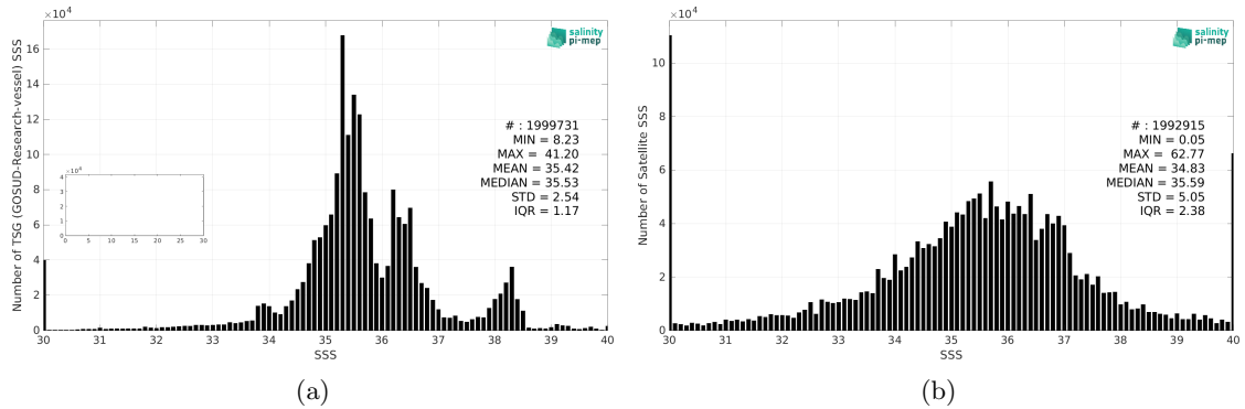
Figure 2: Histograms of SSS from TSG (GOSUD-Research-vessel) (a) and SMOS SSS L2Q v331 - No FLAG (CMEMS-CATDS-CPDC) (b) considering all match-up pairs per bins of 0.1 over the SMOS coastal zone (<800km) 60N-60S Pi-MEP region and for the full satellite product period.
