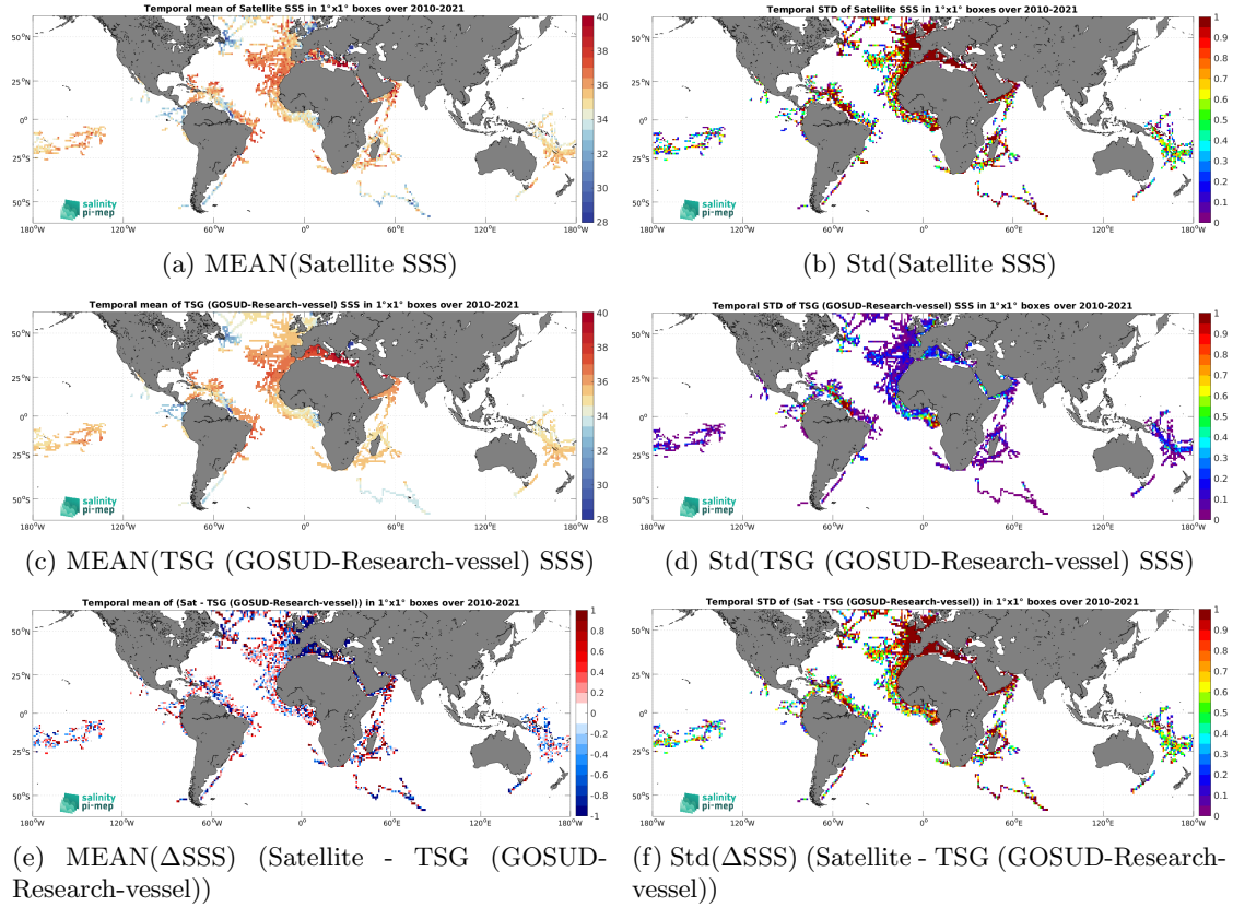
Figure 6: Temporal mean (left) and Std (right) of SSS from SMOS SSS L2Q v331 - No FLAG (CMEMS-CATDS-CPDC) (top), TSG (GOSUD-Research-vessel) (middle), and of \Delta\text{SSS} (Satellite - TSG (GOSUD-Research-vessel)). Only match-up pairs are used to generate these maps.
