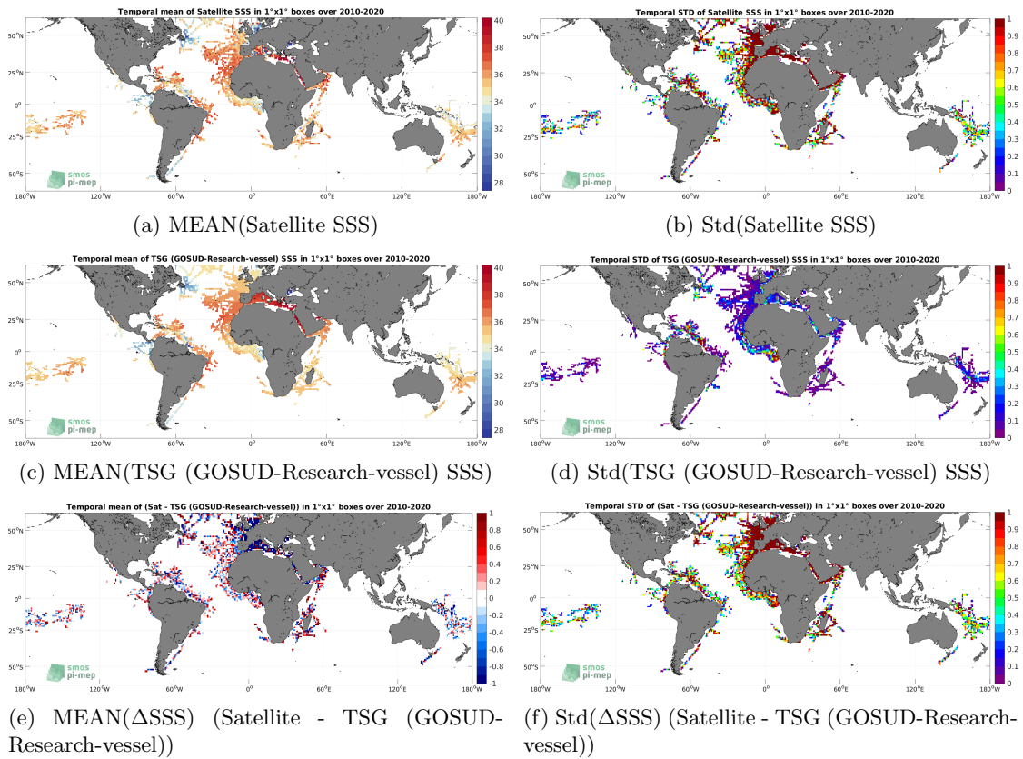
Figure 6: Temporal mean (left) and Std (right) of SSS from SMOS SSS L2Q v331 - No FLAG (CMEMS-CATDS-CPDC) (top), TSG (GOSUD-Research-vessel) (middle), and of \Delta SSS (Satellite - TSG (GOSUD-Research-vessel)). Only match-up pairs are used to generate these maps.
