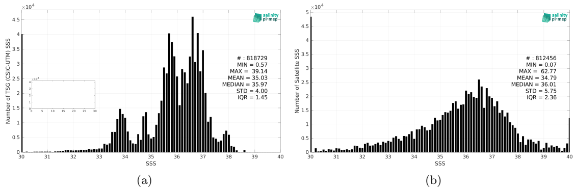
Figure 2: Histograms of SSS from TSG (CSIC-UTM) (a) and SMOS SSS L2Q v331 - No FLAG (CMEMS-CATDS-CPDC) (b) considering all match-up pairs per bins of 0.1 over the SMOS coastal zone (<800km) 60N-60S Pi-MEP region and for the full satellite product period.
