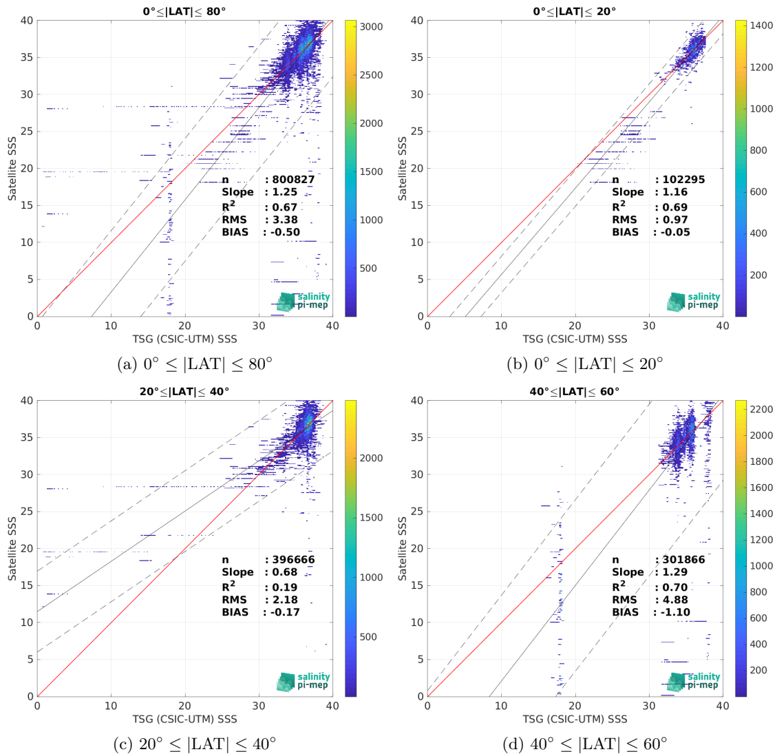
Figure 9: Contour maps of the concentration of SMOS SSS L2Q v331 - No FLAG (CMEMS-CATDS-CPDC) SSS (y-axis) versus TSG (CSIC-UTM) SSS (x-axis) at match-up pairs for different latitude bands. For each plot, the red line shows x=y . The black thin and dashed lines indicate a linear fit through the data cloud and the \pm 95\% confidence levels, respectively. The number match-up pairs n , the slope and R^2 coefficient of the linear fit, the root mean square (RMS) and the mean bias between satellite and in situ data are indicated for each latitude band in each plots.
