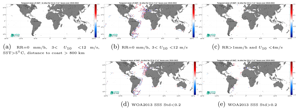
Figure 12: Temporal mean gridded over spatial boxes of size 1^\circ \times 1^\circ of \Delta SSS (SMOS SSS L2Q v331 - No FLAG (CMEMS-CATDS-CPDC) - TSG (CSIC-UTM)) for 5 different subdatasets corresponding to:RR=0 mm/h, 3 < U_{10} < 12 m/s, SST >5^\circ C, distance to coast > 800 km (a), RR=0 mm/h, 3 < U_{10} < 12 m/s (b), RR >1 mm/h and U_{10} < 4 m/s (c), WOA2013 SSS Std <0.2 (d), WOA2013 SSS Std >0.2 (e).
