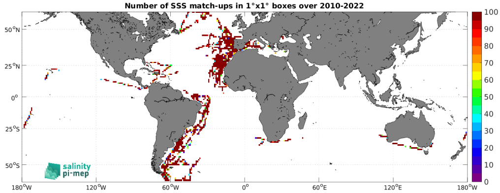
Figure 4: Number of SSS match-ups between TSG (CSIC-UTM) SSS and the SMOS SSS L2Q v331 - No FLAG (CMEMS-CATDS-CPDC) SSS product for the SMOS coastal zone (<800km) 60N-60S Pi-MEP region over 1^\circ \times 1^\circ boxes and for the full satellite product period.
