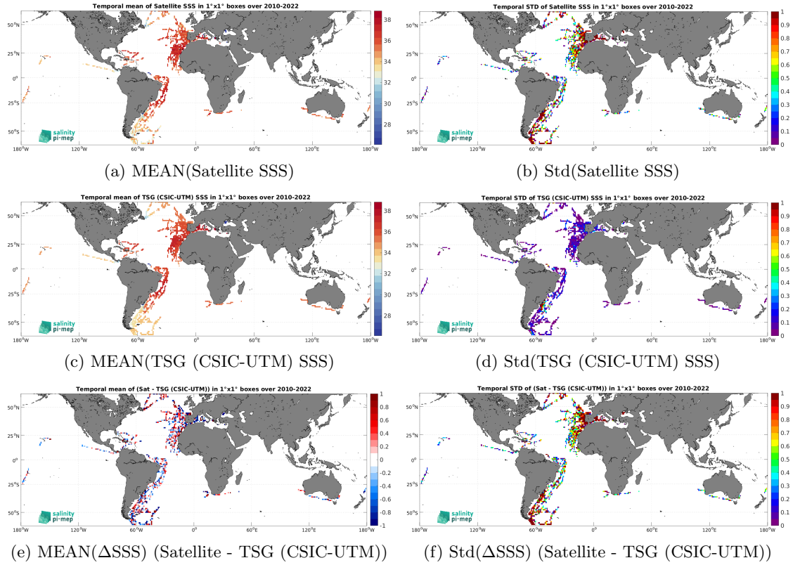
Figure 6: Temporal mean (left) and Std (right) of SSS from SMOS SSS L2Q v331 - No FLAG (CMEMS-CATDS-CPDC) (top), TSG (CSIC-UTM) (middle), and of \Delta SSS (Satellite - TSG (CSIC-UTM)). Only match-up pairs are used to generate these maps.
