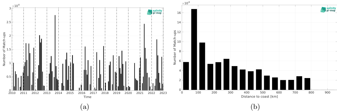
Figure 1: Number of match-ups between TSG (CSIC-UTM) and SMOS SSS L2Q v331 - No FLAG (CMEMS-CATDS-CPDC) SSS as a function of time (a) and as function of the distance to coast (b) over the SMOS coastal zone (<800km) 60N-60S Pi-MEP region and for the full satellite product period.
