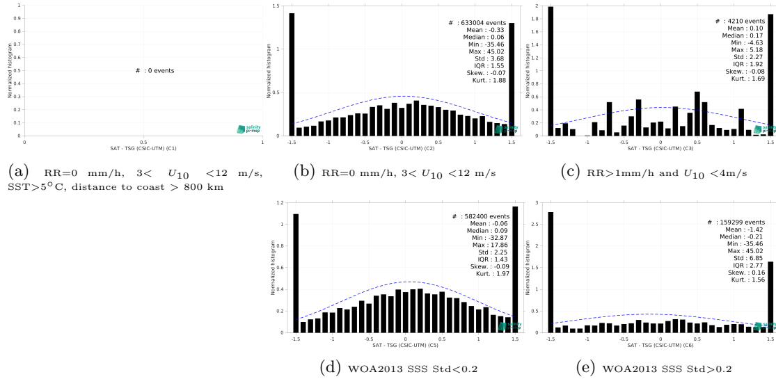
Figure 13: Normalized histogram of \Delta SSS (SMOS SSS L2Q v331 - No FLAG (CMEMS-CATDS-CPDC) - TSG (CSIC-UTM)) for 5 different subdatasets corresponding to: RR=0 mm/h, 3 < U_{10} < 12 m/s, SST>5°C, distance to coast > 800 km (a), RR=0 mm/h, 3 < U_{10} < 12 m/s (b), RR>1mm/h and U_{10} < 4 m/s (c), WOA2013 SSS Std<0.2 (d), WOA2013 SSS Std>0.2 (e).
