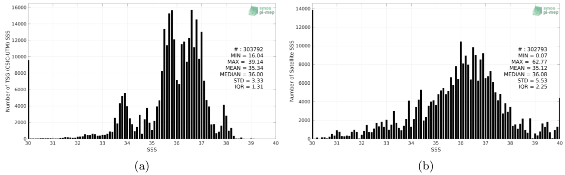
Figure 2: Histograms of SSS from TSG (CSIC-UTM) (a) and SMOS SSS L2Q v331 - No FLAG (CMEMS-CATDS-CPDC) (b) considering all match-up pairs per bins of 0.1 over the SMOS coastal zone (<800km) 60N-60S Pi-MEP region and for the full satellite product period.
