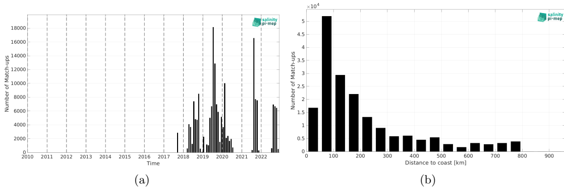
Figure 2: Number of match-ups between Saildrone and SMOS SSS L2Q v331 - No FLAG (CMEMS-CATDS-CPDC) SSS as a function of time (a) and as function of the distance to coast (b) over the SMOS coastal zone (<800km) 60N-60S Pi-MEP region and for the full satellite product period.
