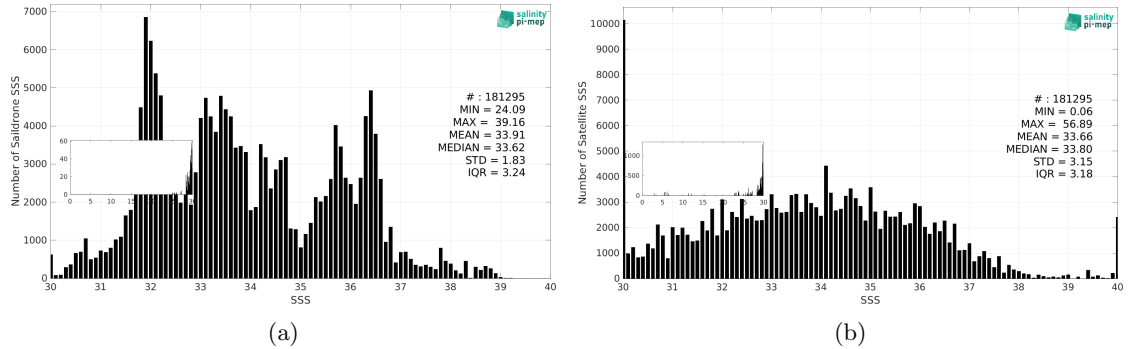
Figure 3: Histograms of SSS from Saildrone (a) and SMOS SSS L2Q v331 - No FLAG (CMEMS-CATDS-CPDC) (b) considering all match-up pairs per bins of 0.1 over the SMOS coastal zone (<800km) 60N-60S Pi-MEP region and for the full satellite product period.
