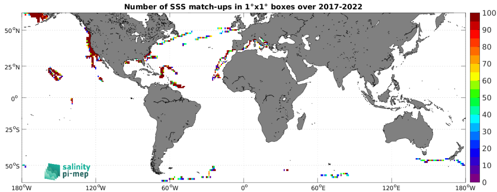
Figure 5: Number of SSS match-ups between Saildrone SSS and the SMOS SSS L2Q v331 - No FLAG (CMEMS-CATDS-CPDC) SSS product for the SMOS coastal zone (<800km) 60N-60S Pi-MEP region over 1^{\circ} \times 1^{\circ} boxes and for the full satellite product period.
