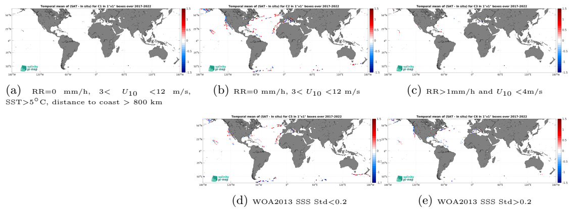
Figure 14: Temporal mean gridded over spatial boxes of size 1^\circ \times 1^\circ of \Delta\text{SSS} (SMOS SSS L2Q v331 - No FLAG (CMEMS-CATDS-CPDC) - Sairdrone) for 5 different subdatasets corresponding to:RR=0 mm/h, 3 < U_{10} < 12 m/s, SST >5^\circ\text{C} , distance to coast > 800 km (a), RR=0 mm/h, 3 < U_{10} < 12 m/s (b), RR >1 mm/h and U_{10} < 4 m/s (c), WOA2013 SSS Std <0.2 (d), WOA2013 SSS Std >0.2 (e).
