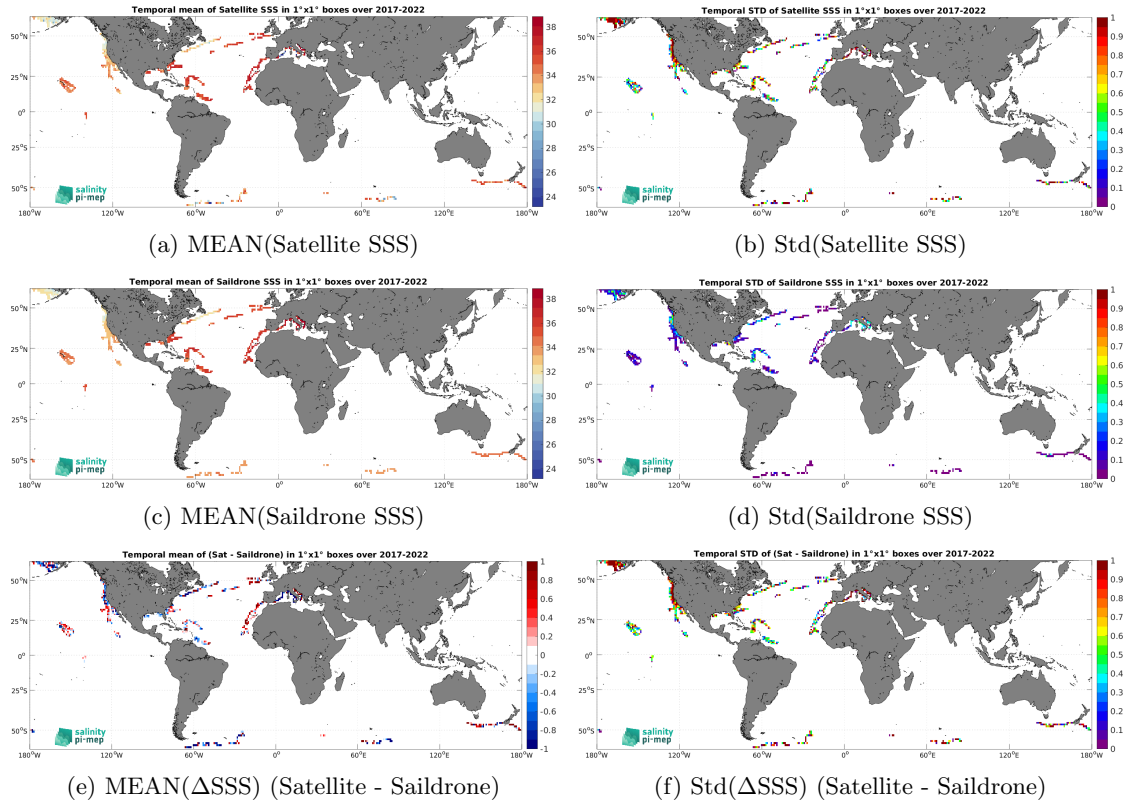
Figure 7: Temporal mean (left) and Std (right) of SSS from SMOS SSS L2Q v331 - No FLAG (CMEMS-CATDS-CPDC) (top), Saildrone (middle), and of \Delta SSS (Satellite - Saildrone). Only match-up pairs are used to generate these maps.
