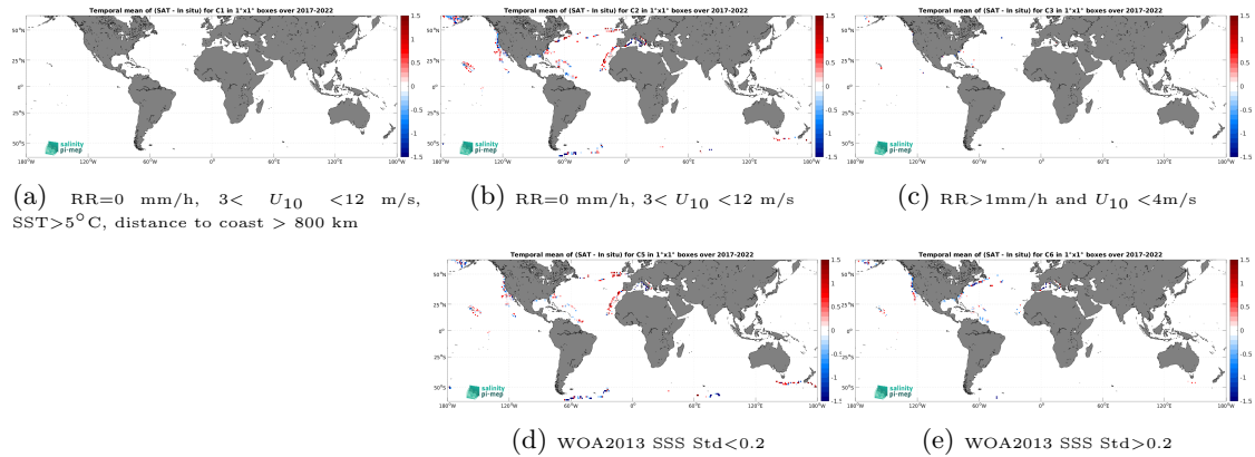
Figure 12: Temporal mean gridded over spatial boxes of size 1^\circ \times 1^\circ of \Delta\text{SSS} (SMOS SSS L2Q v331 - No FLAG (CMEMS-CATDS-CPDC) - Saildrone) for 5 different subdatasets corresponding to:RR=0 mm/h, 3 < U_{10} < 12 m/s, SST >5^\circ\text{C} , distance to coast > 800 km (a), RR=0 mm/h, 3 < U_{10} < 12 m/s (b), RR >1 mm/h and U_{10} < 4 m/s (c), WOA2013 SSS Std <0.2 (d), WOA2013 SSS Std >0.2 (e).
