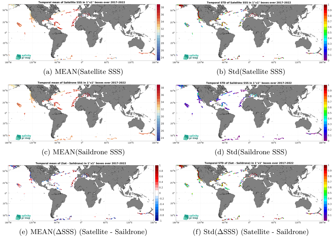
Figure 6: Temporal mean (left) and Std (right) of SSS from SMOS SSS L2Q v331 - No FLAG (CMEMS-CATDS-CPDC) (top), Saildrone (middle), and of \Delta SSS (Satellite - Saildrone). Only match-up pairs are used to generate these maps.
