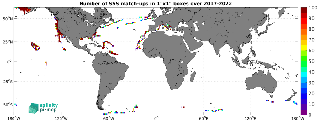
Figure 4: Number of SSS match-ups between Saildrone SSS and the SMOS SSS L2Q v331 - No FLAG (CMEMS-CATDS-CPDC) SSS product for the SMOS coastal zone ( <800\text{km} ) 60N-60S Pi-MEP region over 1^\circ \times 1^\circ boxes and for the full satellite product period.
