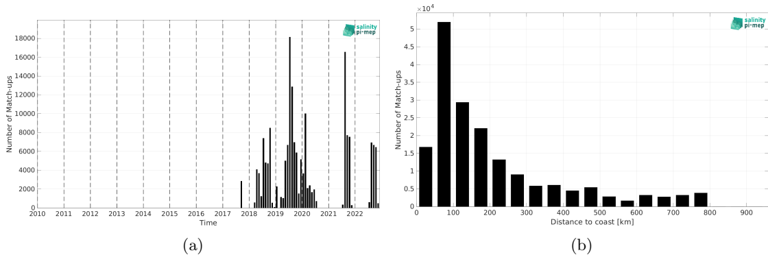
Figure 1: Number of match-ups between Saildrone and SMOS SSS L2Q v331 - No FLAG (CMEMS-CATDS-CPDC) SSS as a function of time (a) and as function of the distance to coast (b) over the SMOS coastal zone (<800km) 60N-60S Pi-MEP region and for the full satellite product period.
