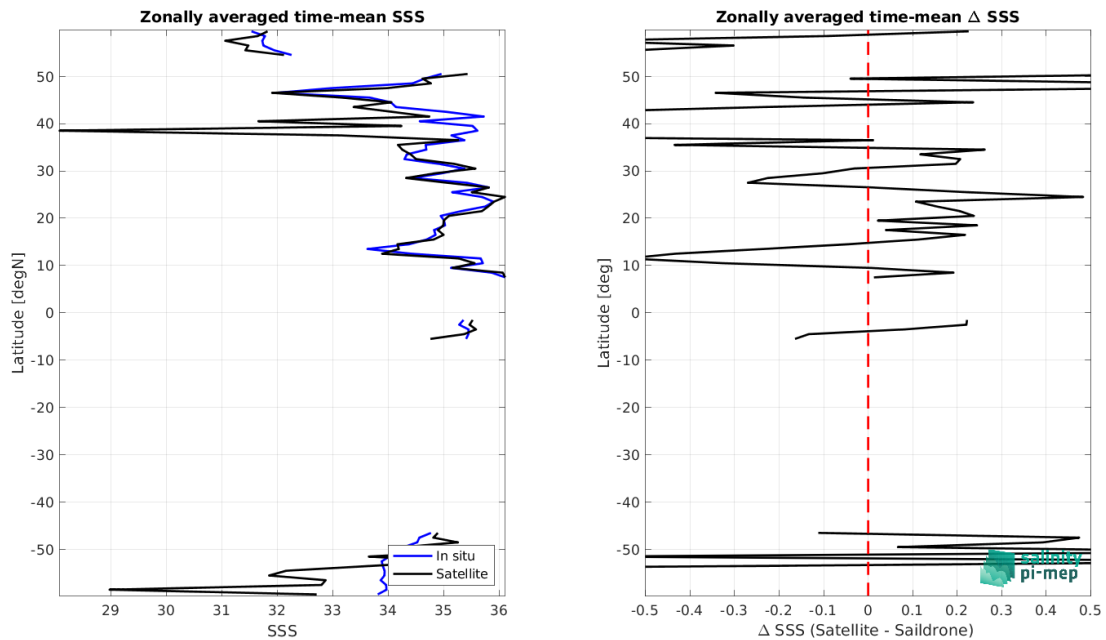
Figure 8: Left panel: Zonal mean SSS from SMOS SSS L2Q v331 - No FLAG (CMEMS-CATDS-CPDC) satellite product (black) and from Sailldrone (blue). Right panel: Zonal mean of \Delta SSS (Satellite - Sailldrone) for all the collected Pi-MEP match-up pairs estimated over the full satellite product period.
