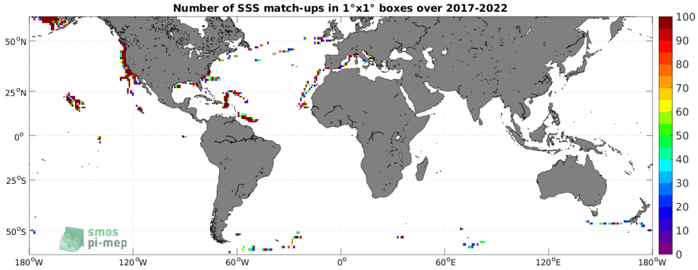
Figure 4: Number of SSS match-ups between Sairdrone SSS and the SMOS SSS L2Q v331 - No FLAG (CMEMS-CATDS-CPDC) SSS product for the SMOS coastal zone ( <800\text{km} ) 60N-60S Pi-MEP region over 1^\circ \times 1^\circ boxes and for the full satellite product period.
