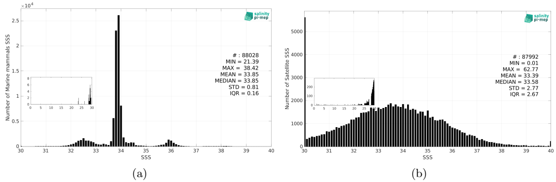
Figure 3: Histograms of SSS from Marine mammals (a) and SMOS SSS L2Q v331 - No FLAG (CMEMS-CATDS-CPDC) (b) considering all match-up pairs per bins of 0.1 over the SMOS coastal zone (<800km) 60N-60S Pi-MEP region and for the full satellite product period.
