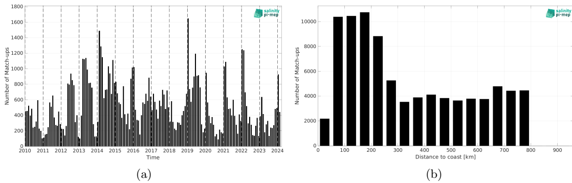
Figure 2: Number of match-ups between Marine mammals and SMOS SSS L2Q v331 - No FLAG (CMEMS-CATDS-CPDC) SSS as a function of time (a) and as function of the distance to coast (b) over the SMOS coastal zone (<800km) 60N-60S Pi-MEP region and for the full satellite product period.
