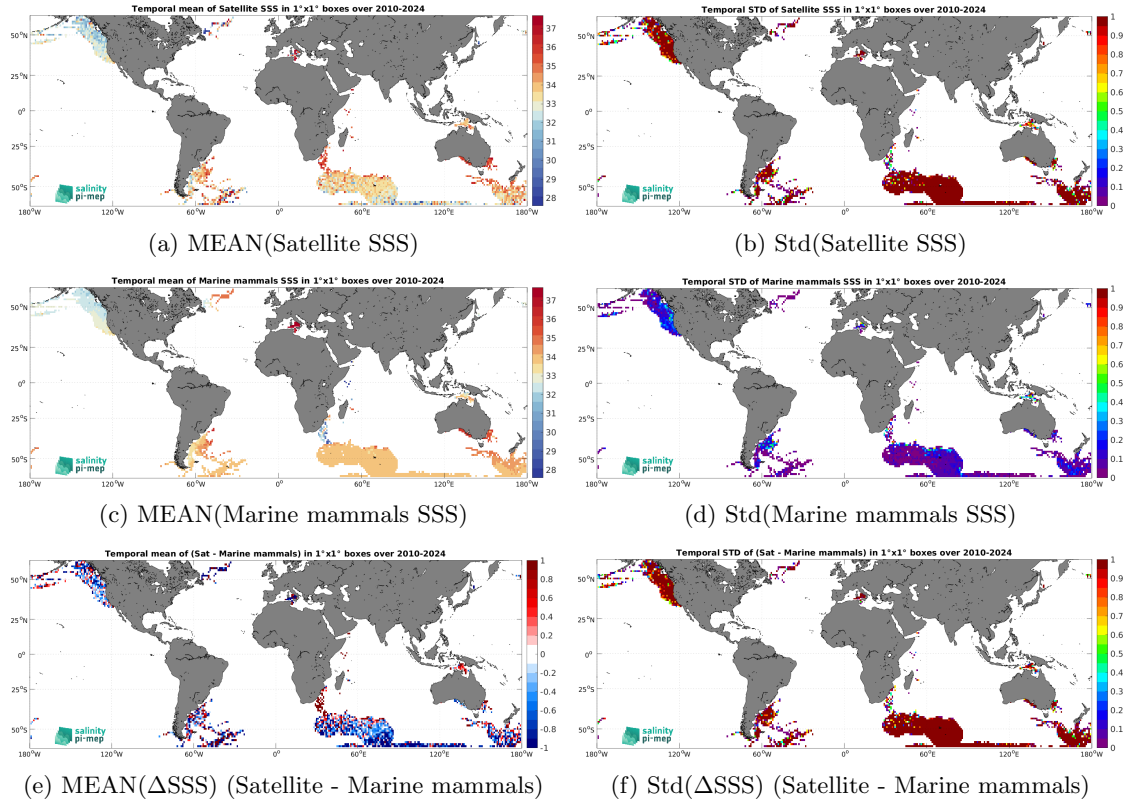
Figure 7: Temporal mean (left) and Std (right) of SSS from SMOS SSS L2Q v331 - No FLAG (CMEMS-CATDS-CPDC) (top), Marine mammals (middle), and of \Delta SSS (Satellite - Marine mammals). Only match-up pairs are used to generate these maps.
