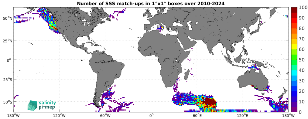
Figure 5: Number of SSS match-ups between Marine mammals SSS and the SMOS SSS L2Q v331 - No FLAG (CMEMS-CATDS-CPDC) SSS product for the SMOS coastal zone (<800km) 60N-60S Pi-MEP region over 1^{\circ} \times 1^{\circ} boxes and for the full satellite product period.
