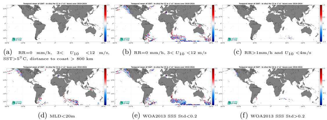
Figure 14: Temporal mean gridded over spatial boxes of size 1^\circ \times 1^\circ of \Delta\text{SSS} (SMOS SSS L2Q v331 - No FLAG (CMEMS-CATDS-CPDC) - Marine mammals) for 6 different subdatasets corresponding to:RR=0 mm/h, 3 < U_{10} < 12 m/s, SST>5°C, distance to coast > 800 km (a), RR=0 mm/h, 3 < U_{10} < 12 m/s (b), RR>1mm/h and U_{10} < 4 m/s (c),MLD<20m (d),WOA2013 SSS Std<0.2 (e),WOA2013 SSS Std>0.2 (f).
