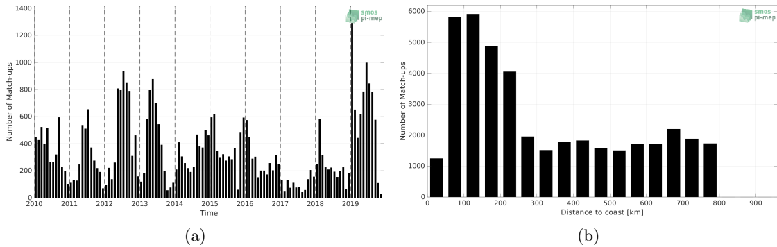
Figure 1: Number of match-ups between Marine mammals and SMOS SSS L2Q v331 - No FLAG (CMEMS-CATDS-CPDC) SSS as a function of time (a) and as function of the distance to coast (b) over the SMOS coastal zone (<800km) 60N-60S Pi-MEP region and for the full satellite product period.
