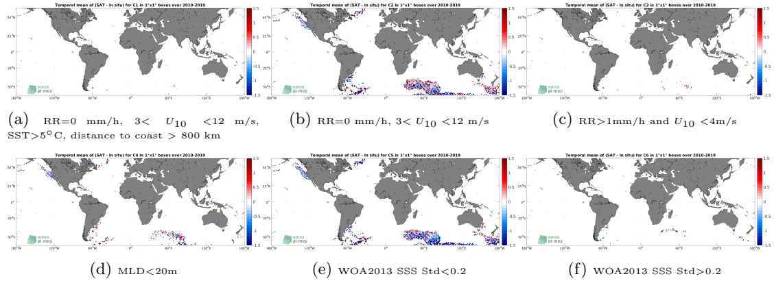
Figure 12: Temporal mean gridded over spatial boxes of size 1^{\circ}\times 1^{\circ} of \Delta\text{SSS} (SMOS SSS L2Q v331 - No FLAG (CMEMS-CATDS-CPDC) - Marine mammals) for 6 different subdatasets corresponding to:RR=0 mm/h, 3 < U_{10} < 12 m/s, SST >5^{\circ}\text{C} , distance to coast > 800 km (a), RR=0 mm/h, 3 < U_{10} < 12 m/s (b), RR >1 mm/h and U_{10} < 4 m/s (c),MLD <20 m (d),WOA2013 SSS Std <0.2 (e),WOA2013 SSS Std >0.2 (f).
