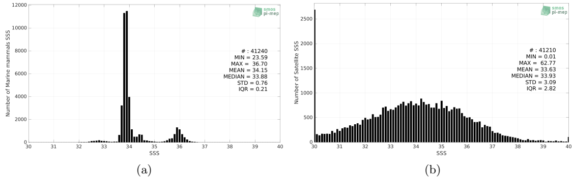
Figure 2: Histograms of SSS from Marine mammals (a) and SMOS SSS L2Q v331 - No FLAG (CMEMS-CATDS-CPDC) (b) considering all match-up pairs per bins of 0.1 over the SMOS coastal zone (<800km) 60N-60S Pi-MEP region and for the full satellite product period.
