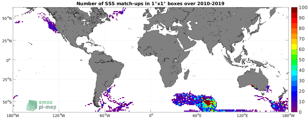
Figure 4: Number of SSS match-ups between Marine mammals SSS and the SMOS SSS L2Q v331 - No FLAG (CMEMS-CATDS-CPDC) SSS product for the SMOS coastal zone (<800km) 60N-60S Pi-MEP region over 1^\circ \times 1^\circ boxes and for the full satellite product period.
