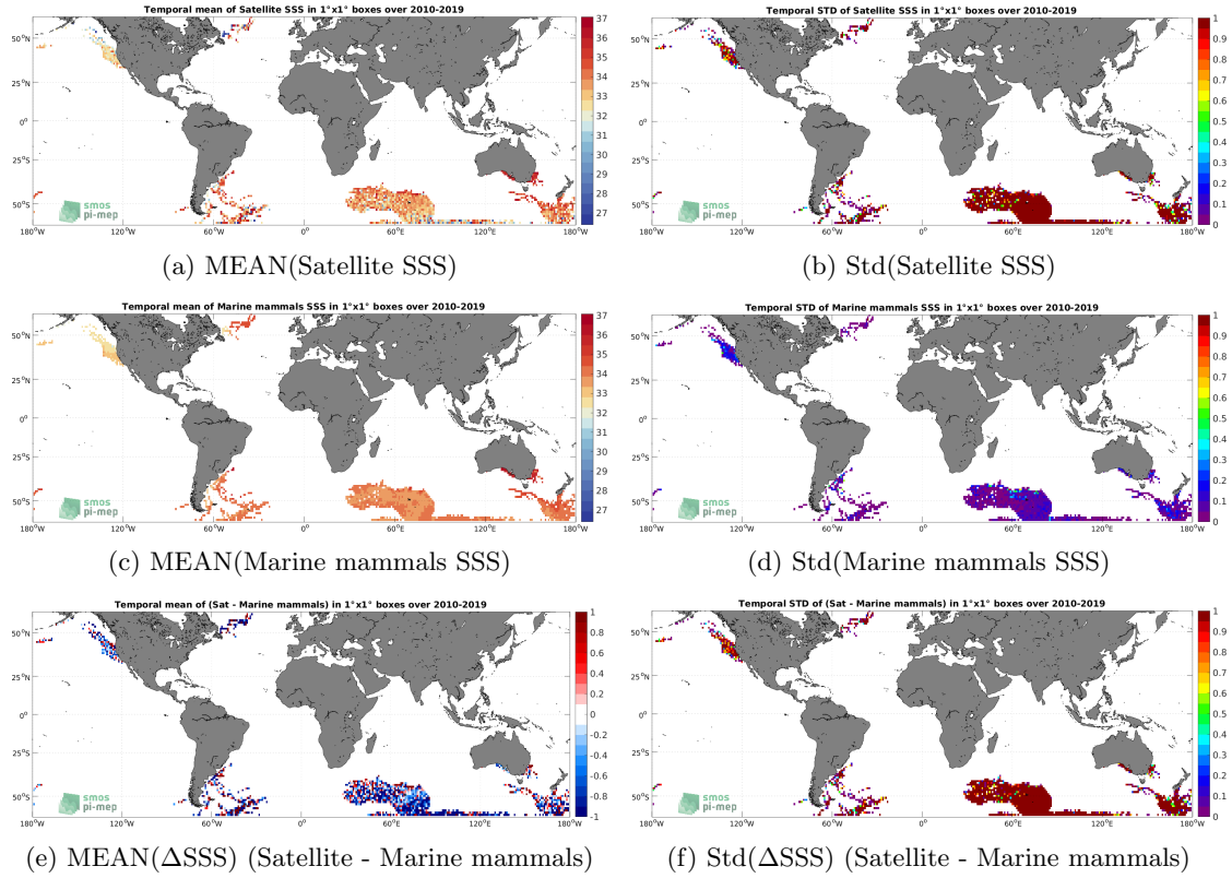
Figure 6: Temporal mean (left) and Std (right) of SSS from SMOS SSS L2Q v331 - No FLAG (CMEMS-CATDS-CPDC) (top), Marine mammals (middle), and of \Delta SSS (Satellite - Marine mammals). Only match-up pairs are used to generate these maps.
