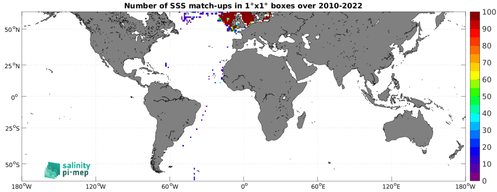
Figure 5: Number of SSS match-ups between ICES SSS and the SMOS SSS L2Q v331 - No FLAG (CMEMS-CATDS-CPDC) SSS product for the SMOS coastal zone (<800km) 60N-60S Pi-MEP region over 1^{\circ} \times 1^{\circ} boxes and for the full satellite product period.
