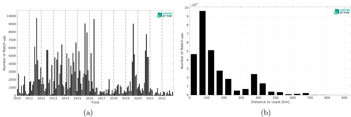
Figure 2: Number of match-ups between ICES and SMOS SSS L2Q v331 - No FLAG (CMEMS-CATDS-CPDC) SSS as a function of time (a) and as function of the distance to coast (b) over the SMOS coastal zone (<800km) 60N-60S Pi-MEP region and for the full satellite product period.
