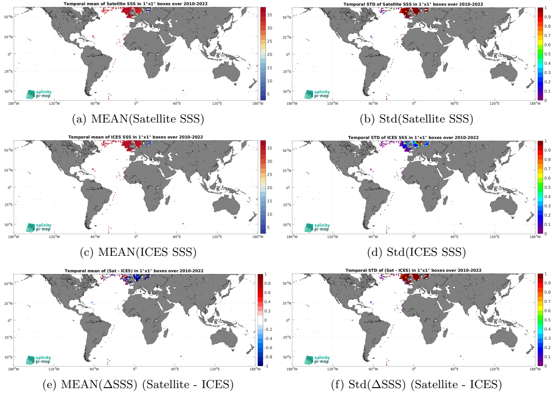
Figure 7: Temporal mean (left) and Std (right) of SSS from SMOS SSS L2Q v331 - No FLAG (CMEMS-CATDS-CPDC) (top), ICES (middle), and of \Delta SSS (Satellite - ICES). Only match-up pairs are used to generate these maps.
