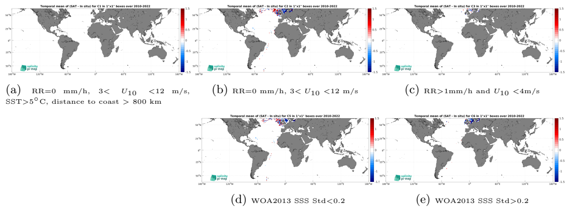
Figure 14: Temporal mean gridded over spatial boxes of size 1^\circ \times 1^\circ of \Delta SSS (SMOS SSS L2Q v331 - No FLAG (CMEMS-CATDS-CPDC) - ICES) for 5 different subdatasets corresponding to:RR=0 mm/h, 3 < U_{10} < 12 m/s, SST > 5^\circ\text{C} , distance to coast > 800 km (a), RR=0 mm/h, 3 < U_{10} < 12 m/s (b), RR > 1 mm/h and U_{10} < 4 m/s (c), WOA2013 SSS Std < 0.2 (d), WOA2013 SSS Std > 0.2 (e).
