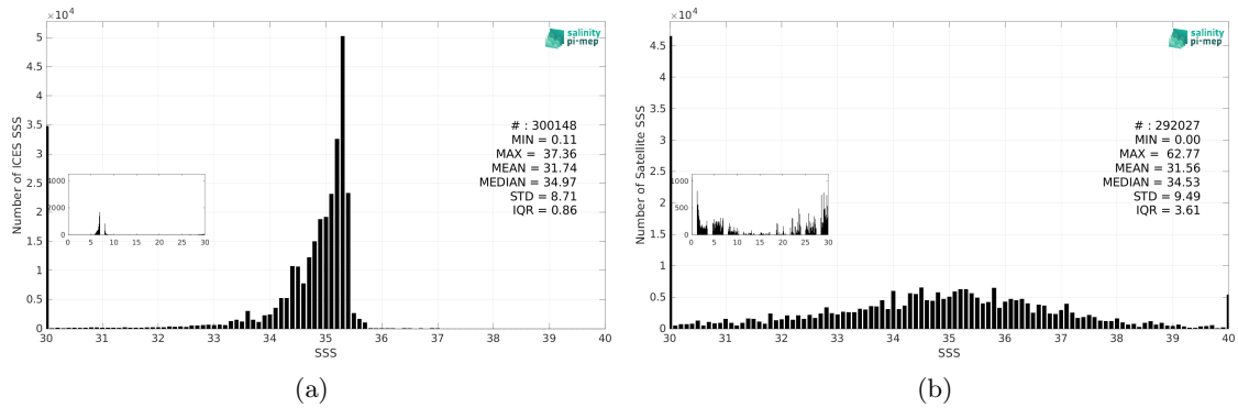
Figure 3: Histograms of SSS from ICES (a) and SMOS SSS L2Q v331 - No FLAG (CMEMS-CATDS-CPDC) (b) considering all match-up pairs per bins of 0.1 over the SMOS coastal zone (<800km) 60N-60S Pi-MEP region and for the full satellite product period.
