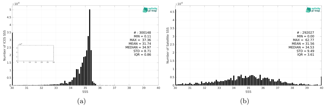
Figure 2: Histograms of SSS from ICES (a) and SMOS SSS L2Q v331 - No FLAG (CMEMS-CATDS-CPDC) (b) considering all match-up pairs per bins of 0.1 over the SMOS coastal zone (<800km) 60N-60S Pi-MEP region and for the full satellite product period.
