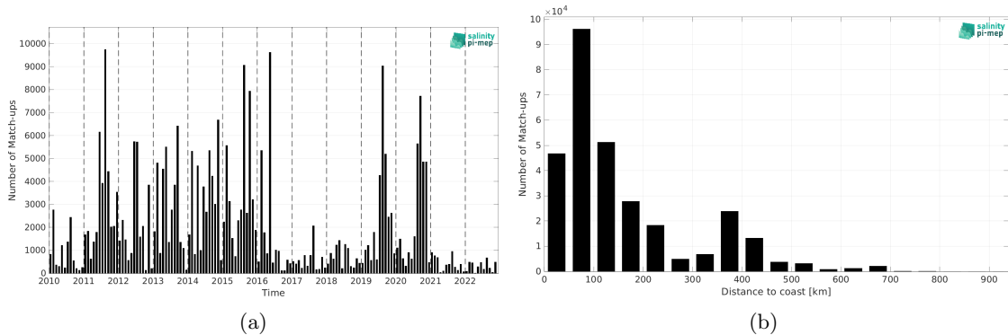
Figure 1: Number of match-ups between ICES and SMOS SSS L2Q v331 - No FLAG (CMEMS-CATDS-CPDC) SSS as a function of time (a) and as function of the distance to coast (b) over the SMOS coastal zone (<800km) 60N-60S Pi-MEP region and for the full satellite product period.
