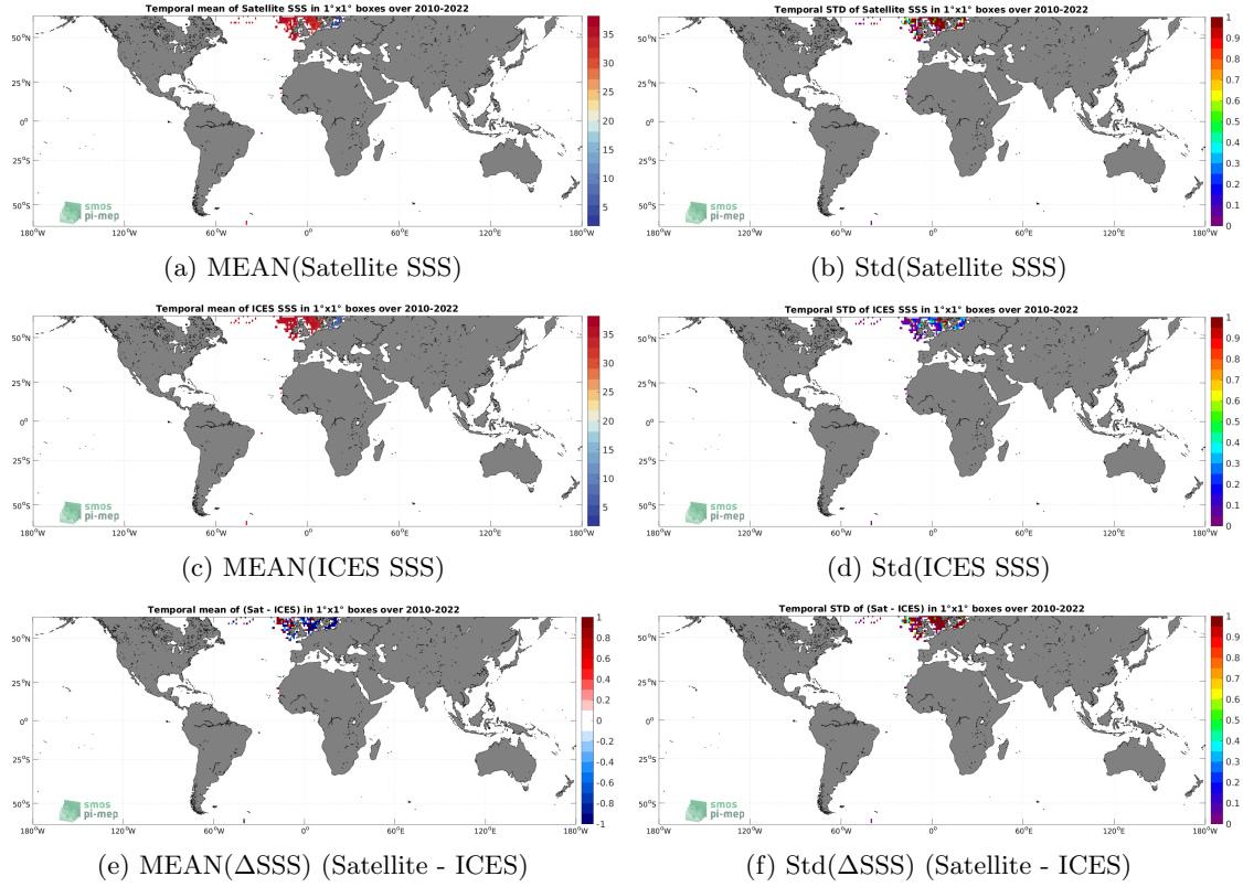
Figure 6: Temporal mean (left) and Std (right) of SSS from SMOS SSS L2Q v331 - No FLAG (CMEMS-CATDS-CPDC) (top), ICES (middle), and of \Delta SSS (Satellite - ICES). Only match-up pairs are used to generate these maps.
