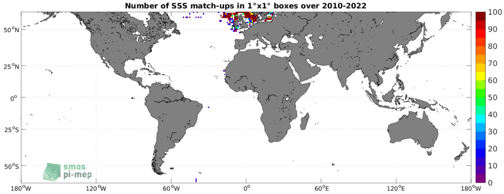
Figure 4: Number of SSS match-ups between ICES SSS and the SMOS SSS L2Q v331 - No FLAG (CMEMS-CATDS-CPDC) SSS product for the SMOS coastal zone (<800km) 60N-60S Pi-MEP region over 1^\circ \times 1^\circ boxes and for the full satellite product period.
