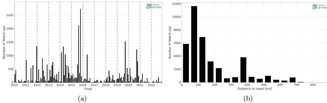
Figure 1: Number of match-ups between ICES and SMOS SSS L2Q v331 - No FLAG (CMEMS-CATDS-CPDC) SSS as a function of time (a) and as function of the distance to coast (b) over the SMOS coastal zone (<800km) 60N-60S Pi-MEP region and for the full satellite product period.
