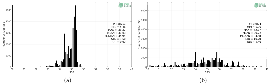
Figure 2: Histograms of SSS from ICES (a) and SMOS SSS L2Q v331 - No FLAG (CMEMS-CATDS-CPDC) (b) considering all match-up pairs per bins of 0.1 over the SMOS coastal zone (<800km) 60N-60S Pi-MEP region and for the full satellite product period.
