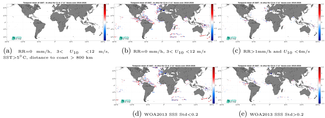
Figure 13: Temporal mean gridded over spatial boxes of size 1^\circ \times 1^\circ of \Delta\text{SSS} (SMOS SSS L2Q v331 - No FLAG (CMEMS-CATDS-CPDC) - Surface drifters) for 5 different subdatasets corresponding to:RR=0 mm/h, 3 < U_{10} < 12 m/s, SST >5^\circ\text{C} , distance to coast > 800 km (a), RR=0 mm/h, 3 < U_{10} < 12 m/s (b), RR >1 mm/h and U_{10} < 4 m/s (c), WOA2013 SSS Std <0.2 (d), WOA2013 SSS Std >0.2 (e).
