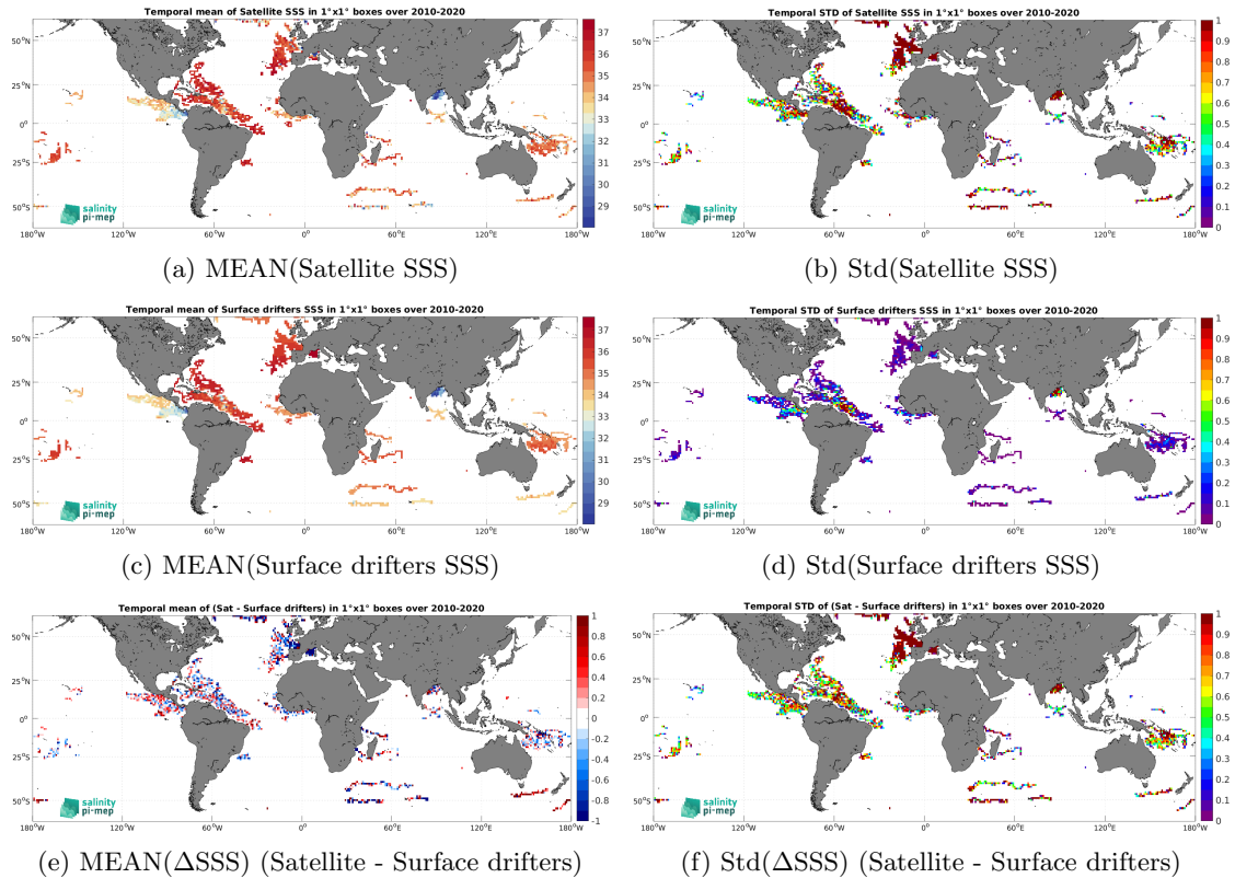
Figure 6: Temporal mean (left) and Std (right) of SSS from SMOS SSS L2Q v331 - No FLAG (CMEMS-CATDS-CPDC) (top), Surface drifters (middle), and of \Delta SSS (Satellite - Surface drifters). Only match-up pairs are used to generate these maps.
