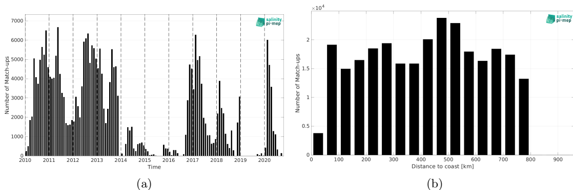
Figure 2: Number of match-ups between Surface drifters and SMOS SSS L2Q v331 - No FLAG (CMEMS-CATDS-CPDC) SSS as a function of time (a) and as function of the distance to coast (b) over the SMOS coastal zone (<800km) 60N-60S Pi-MEP region and for the full satellite product period.
