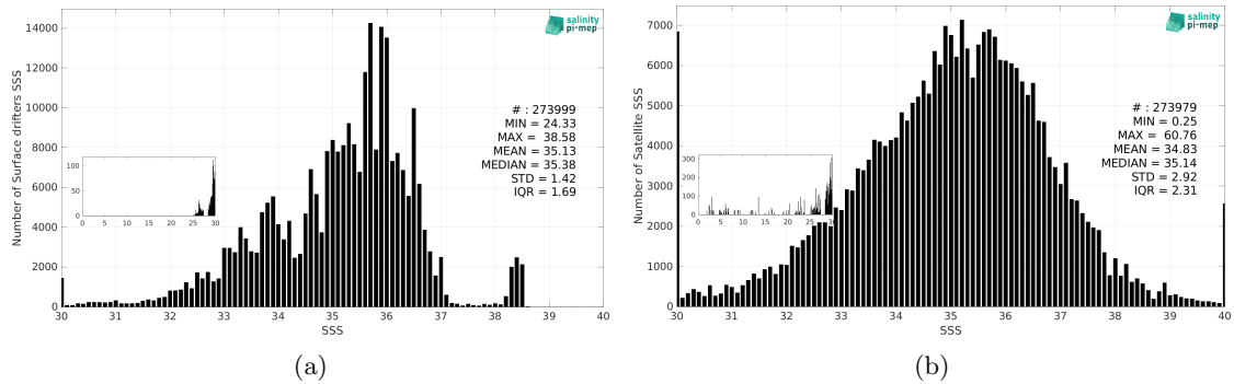
Figure 3: Histograms of SSS from Surface drifters (a) and SMOS SSS L2Q v331 - No FLAG (CMEMS-CATDS-CPDC) (b) considering all match-up pairs per bins of 0.1 over the SMOS coastal zone (<800km) 60N-60S Pi-MEP region and for the full satellite product period.
