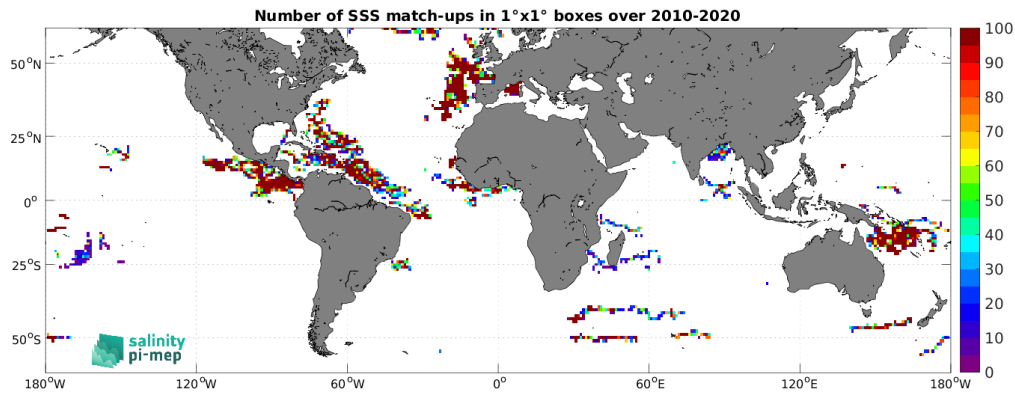
Figure 4: Number of SSS match-ups between Surface drifters SSS and the SMOS SSS L2Q v331 - No FLAG (CMEMS-CATDS-CPDC) SSS product for the SMOS coastal zone (<800km) 60N-60S Pi-MEP region over 1^\circ \times 1^\circ boxes and for the full satellite product period.
