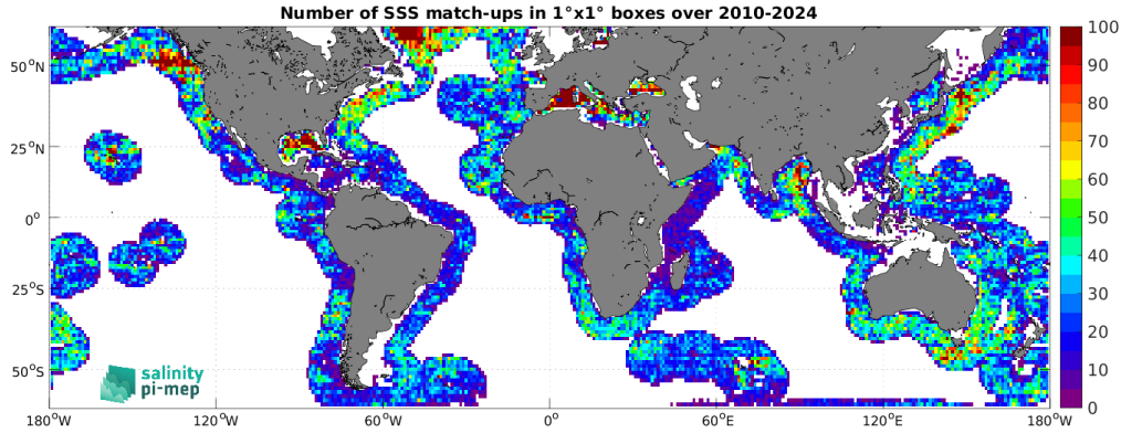
Figure 5: Number of SSS match-ups between Argo SSS and the SMOS SSS L2Q v331 - No FLAG (CMEMS-CATDS-CPDC) SSS product for the SMOS coastal zone (<800km) 60N-60S Pi-MEP region over 1^\circ \times 1^\circ boxes and for the full satellite product period.
