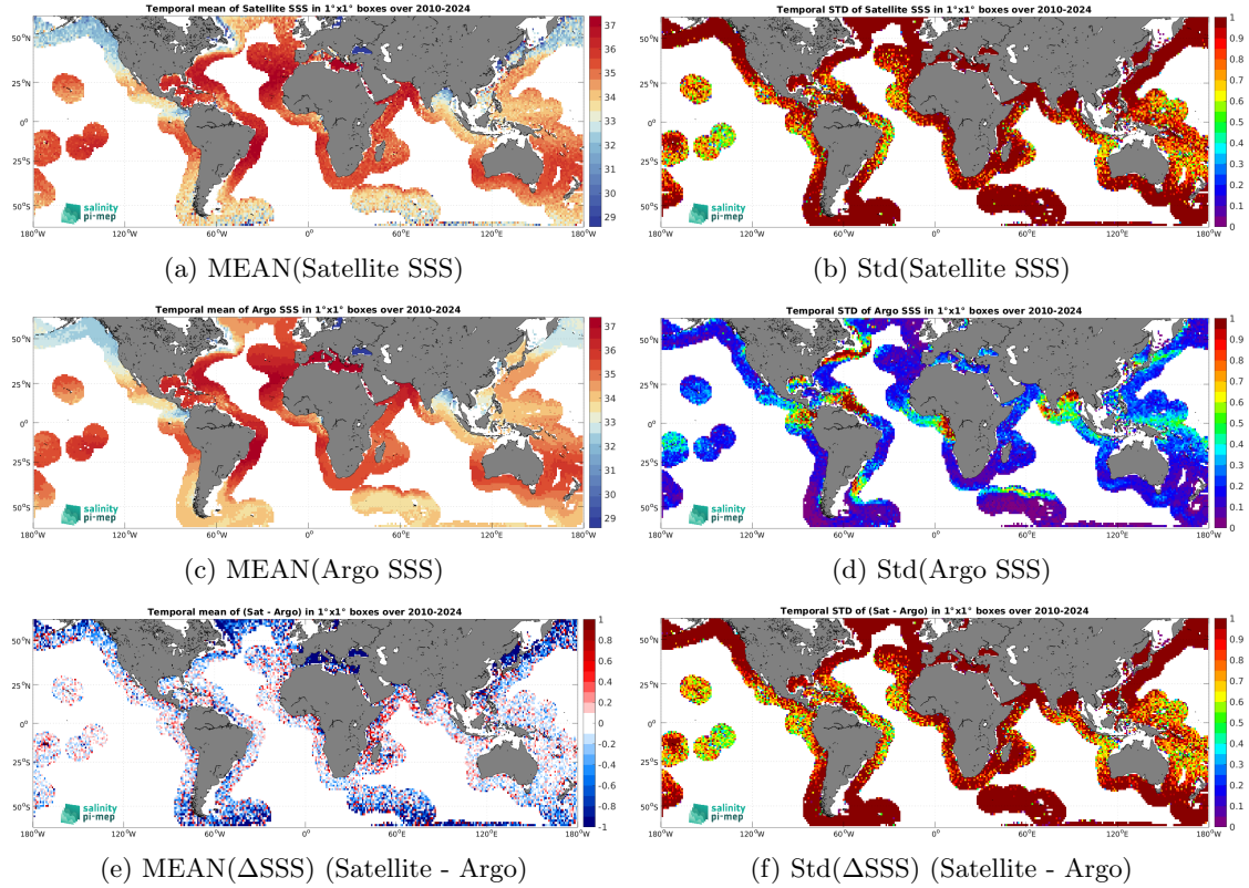
Figure 7: Temporal mean (left) and Std (right) of SSS from SMOS SSS L2Q v331 - No FLAG (CMEMS-CATDS-CPDC) (top), Argo (middle), and of \Delta SSS (Satellite - Argo). Only match-up pairs are used to generate these maps.
