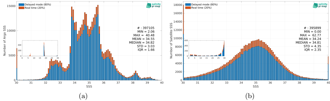
Figure 3: Histograms of SSS from Argo (a) and SMOS SSS L2Q v331 - No FLAG (CMEMS-CATDS-CPDC) (b) considering all match-up pairs per bins of 0.1 over the SMOS coastal zone (<800km) 60N-60S Pi-MEP region and for the full satellite product period.
