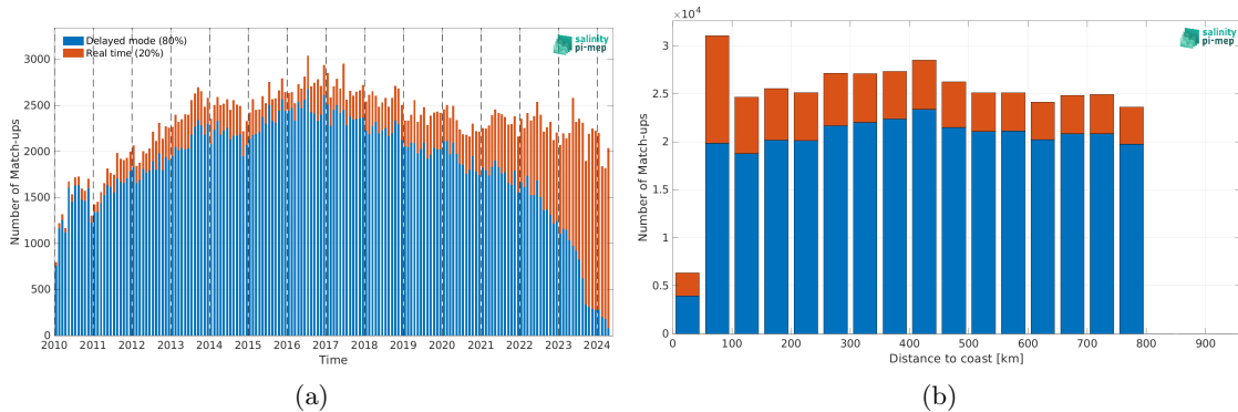
Figure 2: Number of match-ups between Argo and SMOS SSS L2Q v331 - No FLAG (CMEMS-CATDS-CPDC) SSS as a function of time (a) and as function of the distance to coast (b) over the SMOS coastal zone (<800km) 60N-60S Pi-MEP region and for the full satellite product period.
