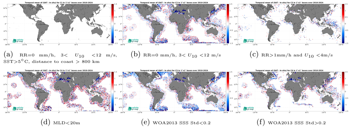
Figure 14: Temporal mean gridded over spatial boxes of size 1^\circ \times 1^\circ of \Delta\text{SSS} (SMOS SSS L2Q v331 - No FLAG (CMEMS-CATDS-CPDC) - Argo) for 6 different subdatasets corresponding to:RR=0 mm/h, 3 < U_{10} < 12 m/s, SST>5°C, distance to coast > 800 km (a), RR=0 mm/h, 3 < U_{10} < 12 m/s (b), RR>1mm/h and U_{10} < 4 m/s (c),MLD<20m (d),WOA2013 SSS Std<0.2 (e),WOA2013 SSS Std>0.2 (f).
