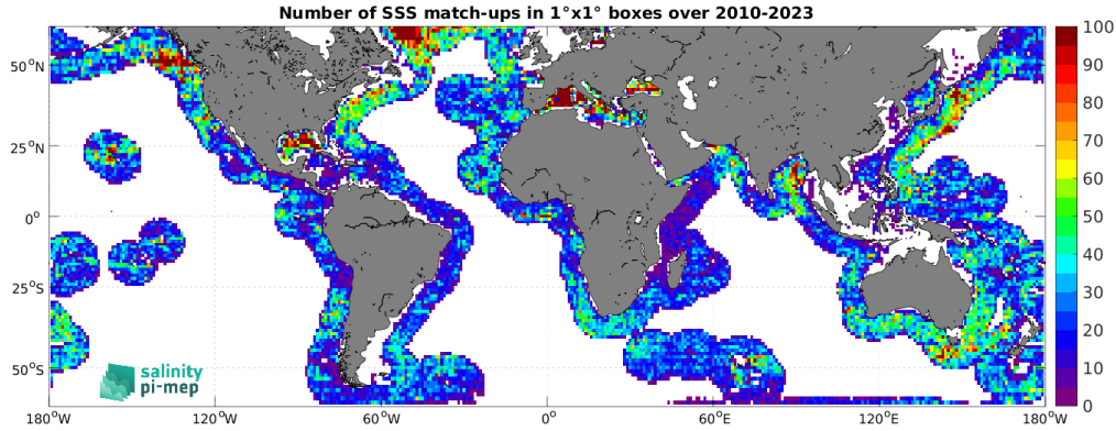
Figure 4: Number of SSS match-ups between Argo SSS and the SMOS SSS L2Q v331 - No FLAG (CMEMS-CATDS-CPDC) SSS product for the SMOS coastal zone ( <800\text{km} ) 60N-60S Pi-MEP region over 1^\circ \times 1^\circ boxes and for the full satellite product period.
