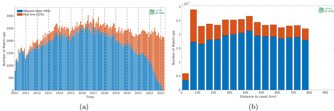
Figure 1: Number of match-ups between Argo and SMOS SSS L2Q v331 - No FLAG (CMEMS-CATDS-CPDC) SSS as a function of time (a) and as function of the distance to coast (b) over the SMOS coastal zone (<800km) 60N-60S Pi-MEP region and for the full satellite product period.
