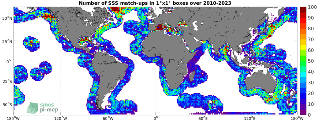
Figure 4: Number of SSS match-ups between Argo SSS and the SMOS SSS L2Q v331 - No FLAG (CMEMS-CATDS-CPDC) SSS product for the SMOS coastal zone (<800km) 60N-60S Pi-MEP region over 1^\circ \times 1^\circ boxes and for the full satellite product period.
