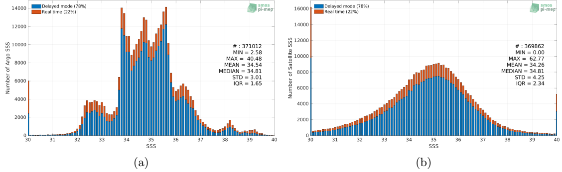
Figure 2: Histograms of SSS from Argo (a) and SMOS SSS L2Q v331 - No FLAG (CMEMS-CATDS-CPDC) (b) considering all match-up pairs per bins of 0.1 over the SMOS coastal zone (<800km) 60N-60S Pi-MEP region and for the full satellite product period.
