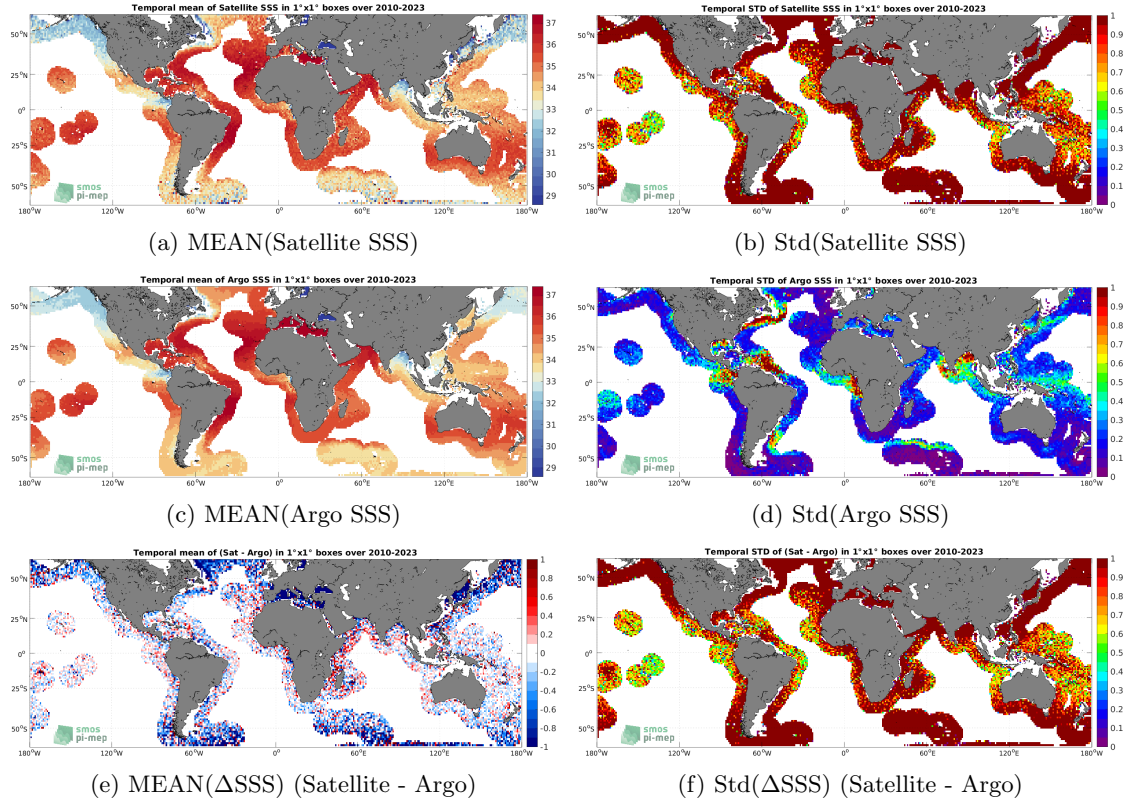
Figure 6: Temporal mean (left) and Std (right) of SSS from SMOS SSS L2Q v331 - No FLAG (CMEMS-CATDS-CPDC) (top), Argo (middle), and of \Delta SSS (Satellite - Argo). Only match-up pairs are used to generate these maps.
