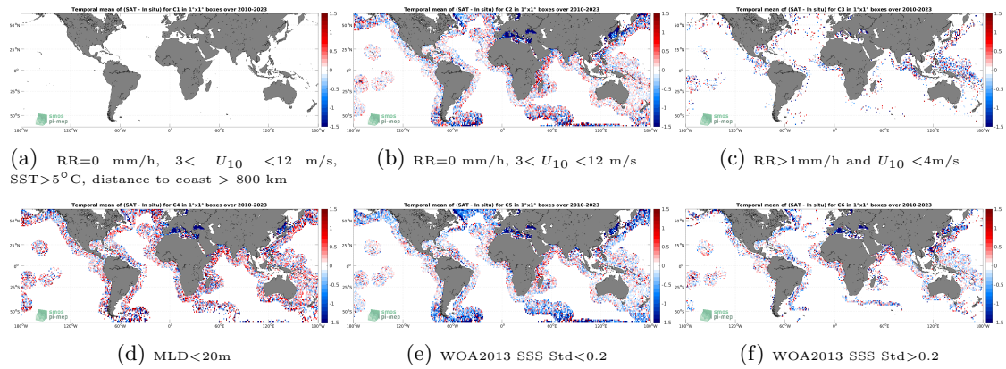
Figure 12: Temporal mean gridded over spatial boxes of size 1^\circ \times 1^\circ of \Delta SSS (SMOS SSS L2Q v331 - No FLAG (CMEMS-CATDS-CPDC) - Argo) for 6 different subdatasets corresponding to:RR=0 mm/h, 3 < U_{10} < 12 m/s, SST >5^\circ C, distance to coast > 800 km (a), RR=0 mm/h, 3 < U_{10} < 12 m/s (b), RR >1 mm/h and U_{10} < 4 m/s (c),MLD <20 m (d),WOA2013 SSS Std <0.2 (e),WOA2013 SSS Std >0.2 (f).
