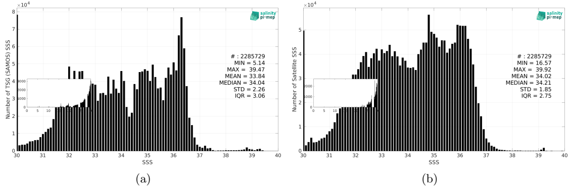
Figure 3: Histograms of SSS from TSG (SAMOS) (a) and SMOS SSS L3 v9 - 9 Days (CATDS-CEC-LOCEAN) (b) considering all match-up pairs per bins of 0.1 over the SMOS coastal zone (<800km) 60N-60S Pi-MEP region and for the full satellite product period.
