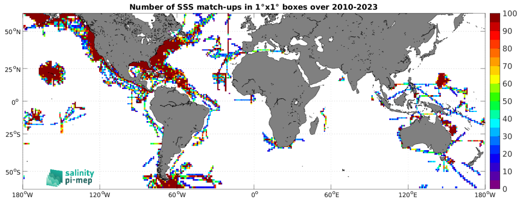
Figure 5: Number of SSS match-ups between TSG (SAMOS) SSS and the SMOS SSS L3 v9 - 9 Days (CATDS-CEC-LOCEAN) SSS product for the SMOS coastal zone (<800km) 60N-60S Pi-MEP region over 1^\circ \times 1^\circ boxes and for the full satellite product period.
