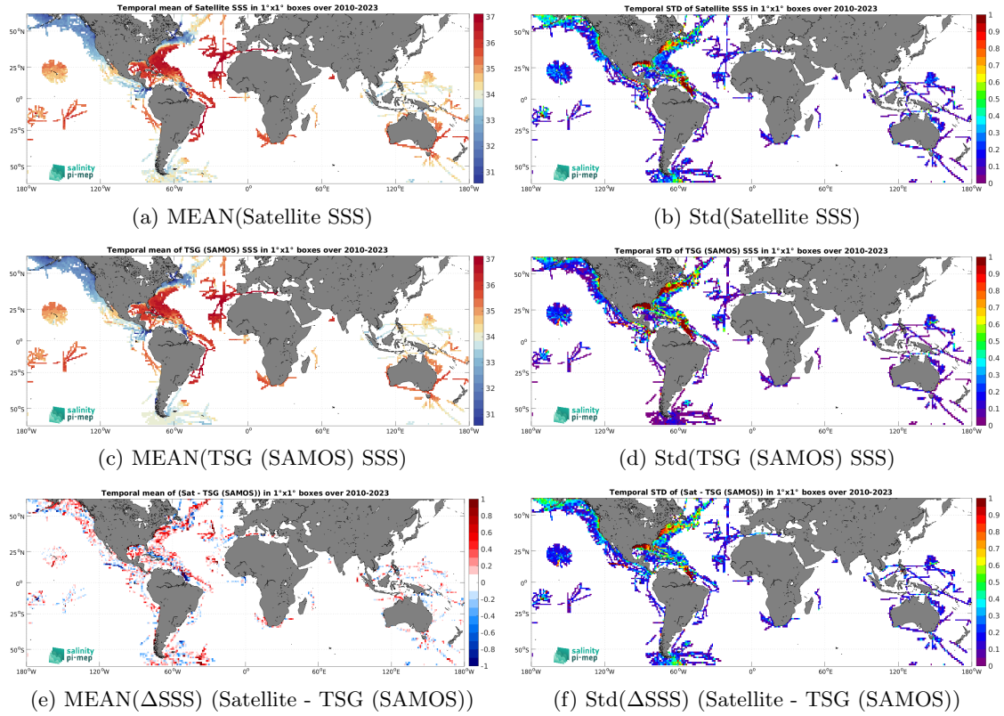
Figure 7: Temporal mean (left) and Std (right) of SSS from SMOS SSS L3 v9 - 9 Days (CATDS-CEC-LOCEAN) (top), TSG (SAMOS) (middle), and of \Delta SSS (Satellite - TSG (SAMOS)). Only match-up pairs are used to generate these maps.
