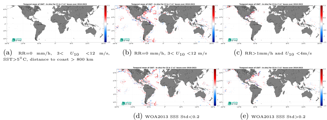
Figure 14: Temporal mean gridded over spatial boxes of size 1^\circ \times 1^\circ of \Delta\text{SSS} (SMOS SSS L3 v9 - 9 Days (CATDS-CEC-LOCEAN) - TSG (SAMOS)) for 5 different subdatasets corresponding to:RR=0 mm/h, 3 < U_{10} < 12 m/s, SST >5^\circ\text{C} , distance to coast > 800 km (a), RR=0 mm/h, 3 < U_{10} < 12 m/s (b), RR >1 mm/h and U_{10} < 4 m/s (c), WOA2013 SSS Std <0.2 (d), WOA2013 SSS Std >0.2 (e).
