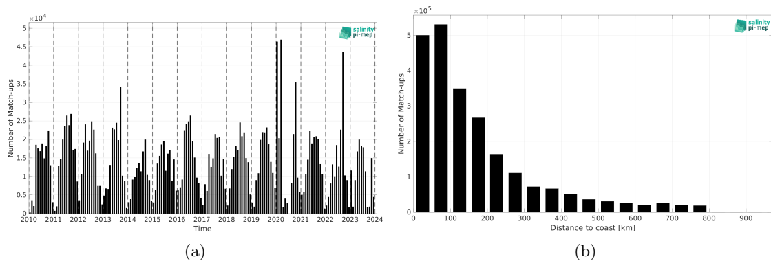
Figure 2: Number of match-ups between TSG (SAMOS) and SMOS SSS L3 v9 - 9 Days (CATDS-CEC-LOCEAN) SSS as a function of time (a) and as function of the distance to coast (b) over the SMOS coastal zone (<800km) 60N-60S Pi-MEP region and for the full satellite product period.
